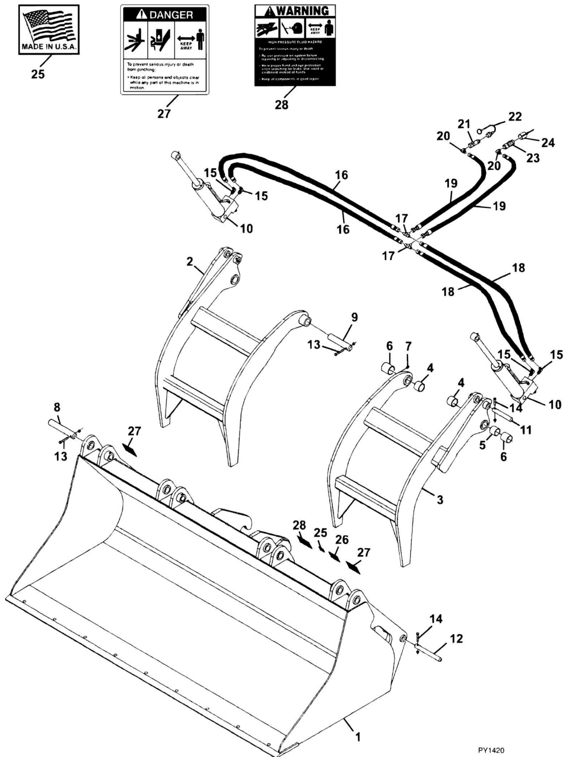
FIGURE 3-22. GRAPPLE BUCKET (SN 0160037900 to Present, Including 0160037855)
