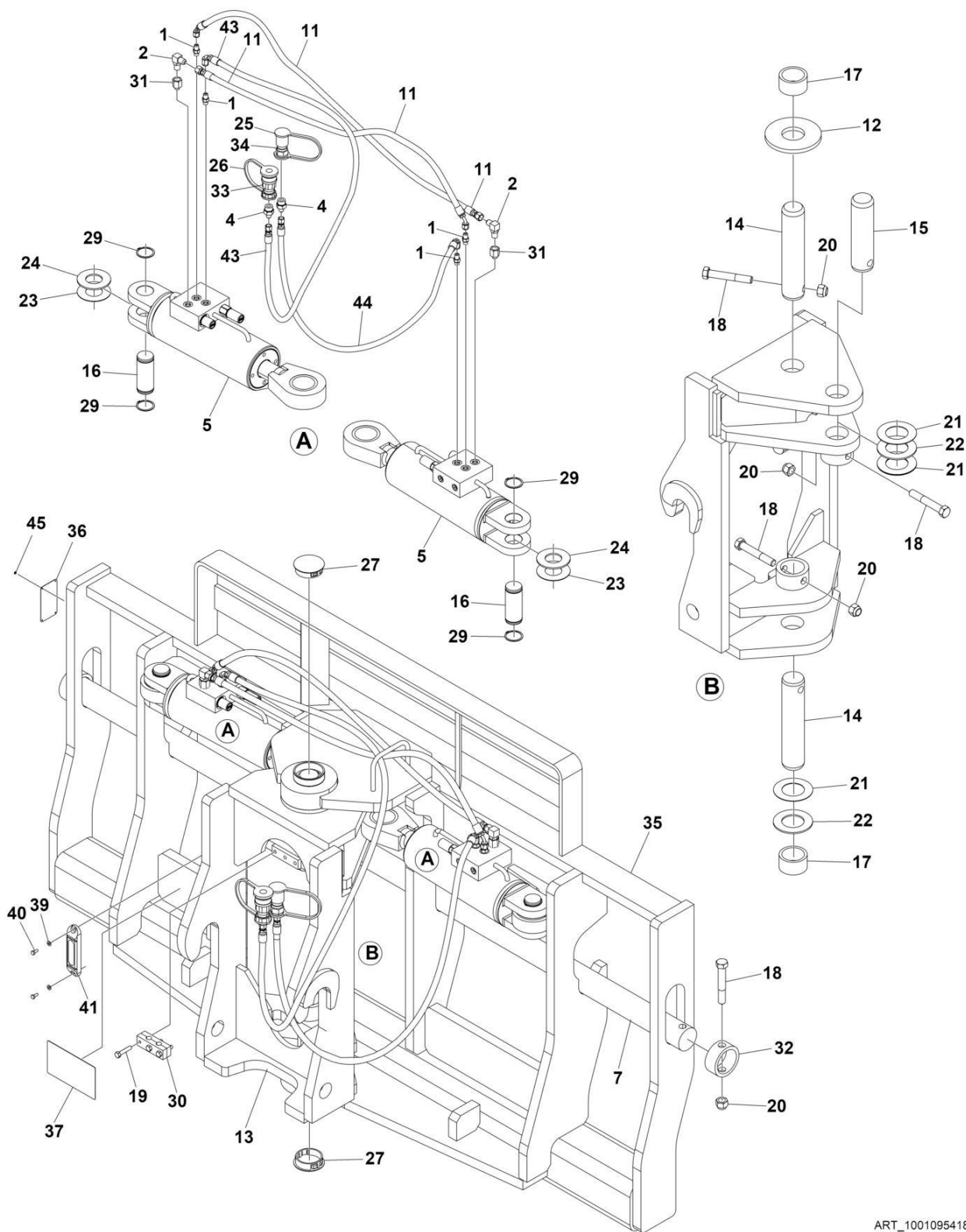
FIGURE 3-21. CARRIAGE ASSEMBLY - 72IN SWING
