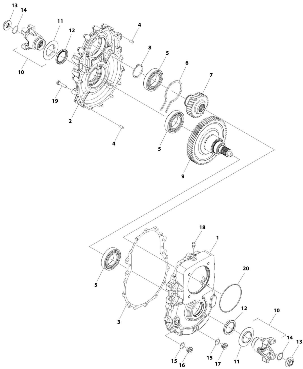
FIGURE 5-27. GEARBOX ASSEMBLY
