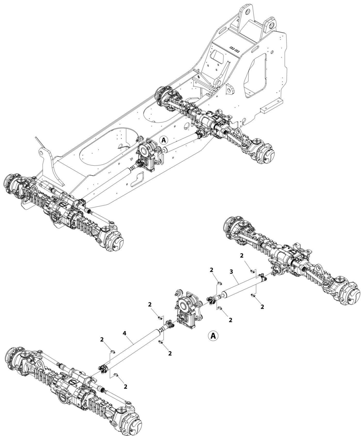
FIGURE 5-21. DRIVESHAFT INSTALLATION
