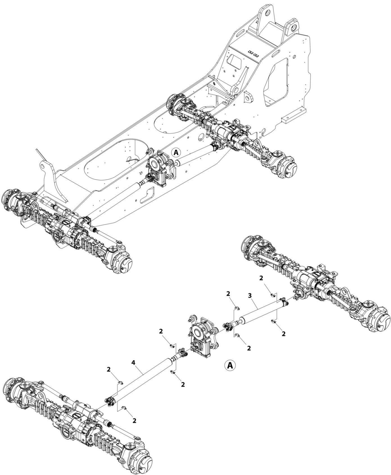
FIGURE 5-16. DRIVESHAFT INSTALLATION
