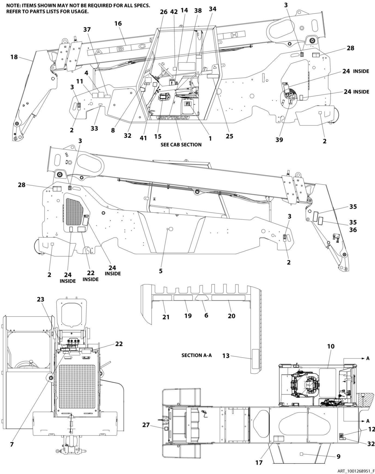
FIGURE 11-1. DECALS INSTALLATION (ANSI SPECS)
