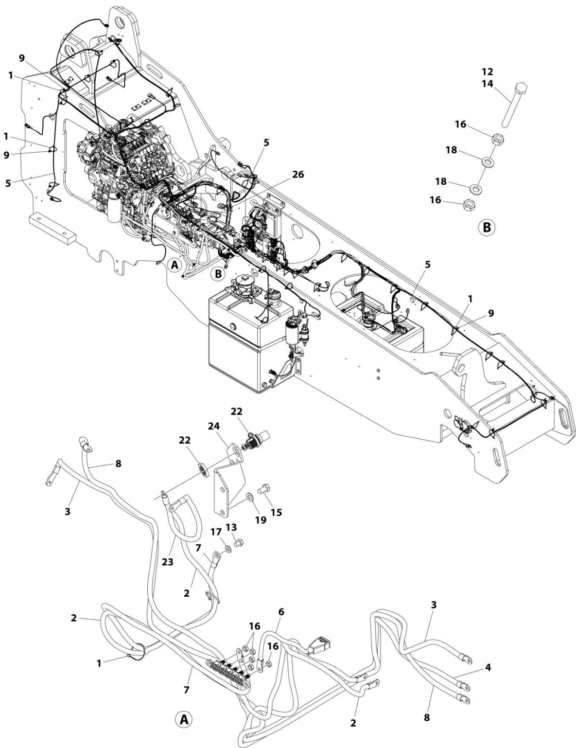
FIGURE 10-22. FRAME HARNESS INSTALLATION
