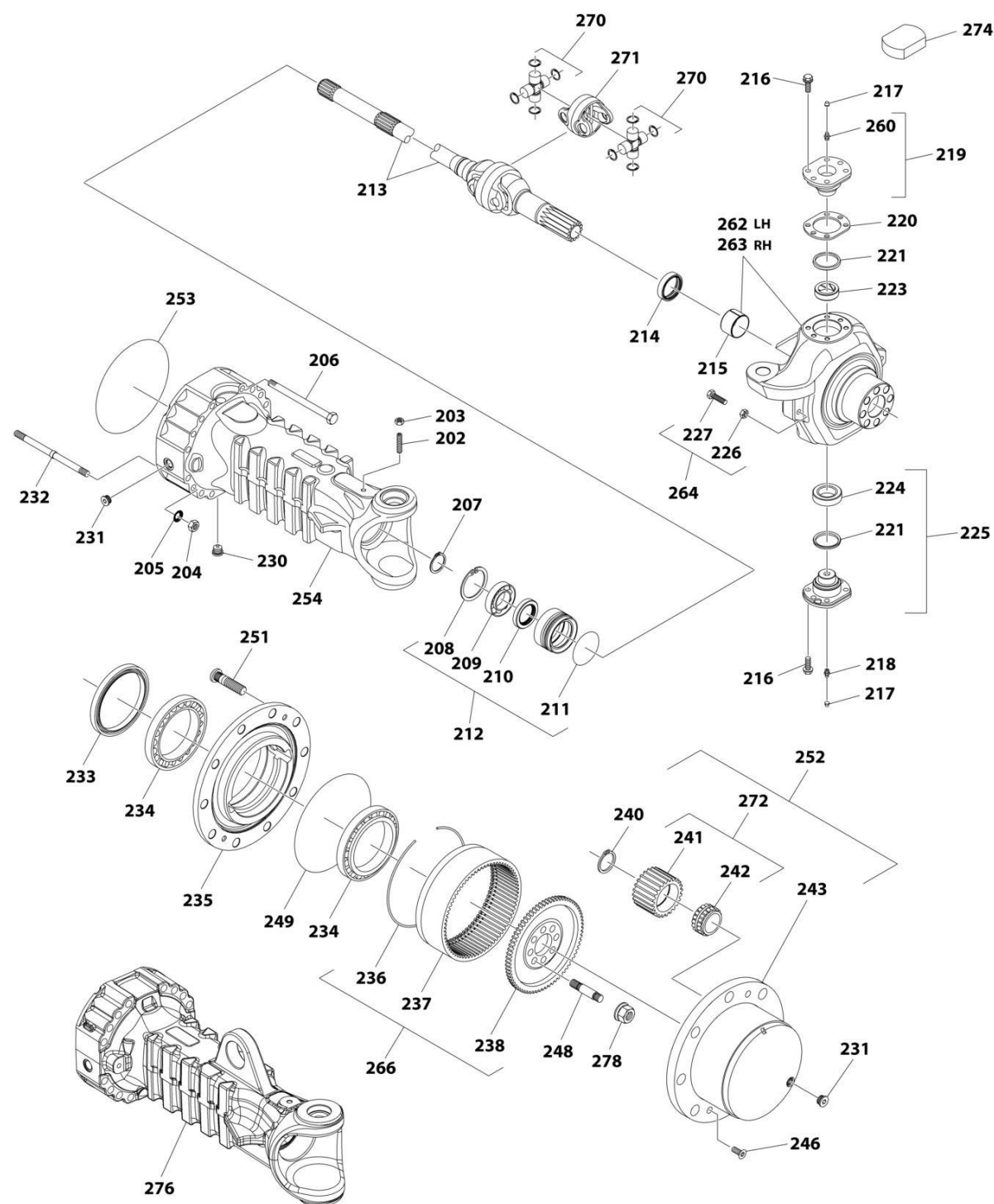
FIGURE 5-4. FRONT AXLE ASSEMBLY - HUB REDUCTION
