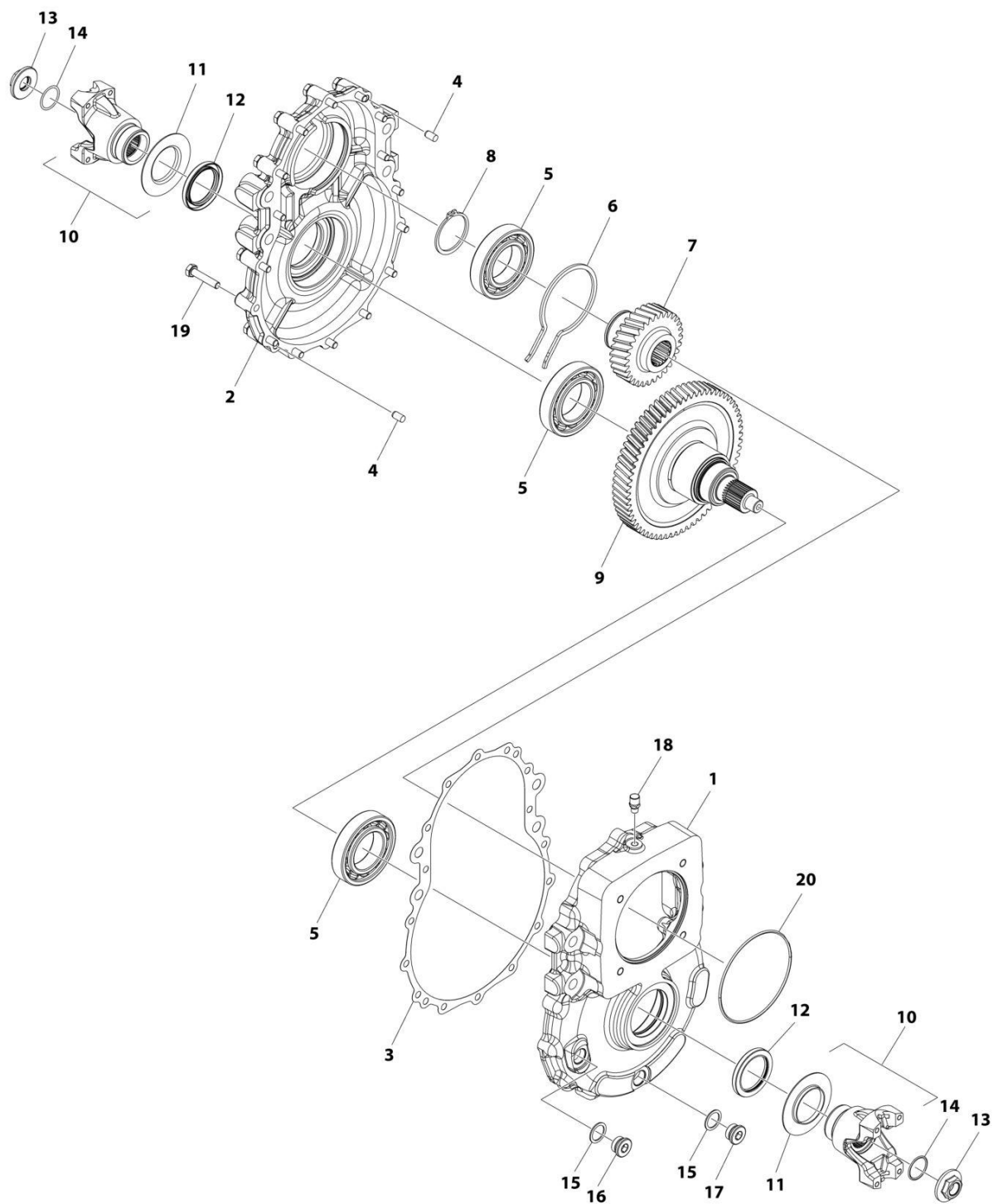
FIGURE 5-21. GEARBOX ASSEMBLY
