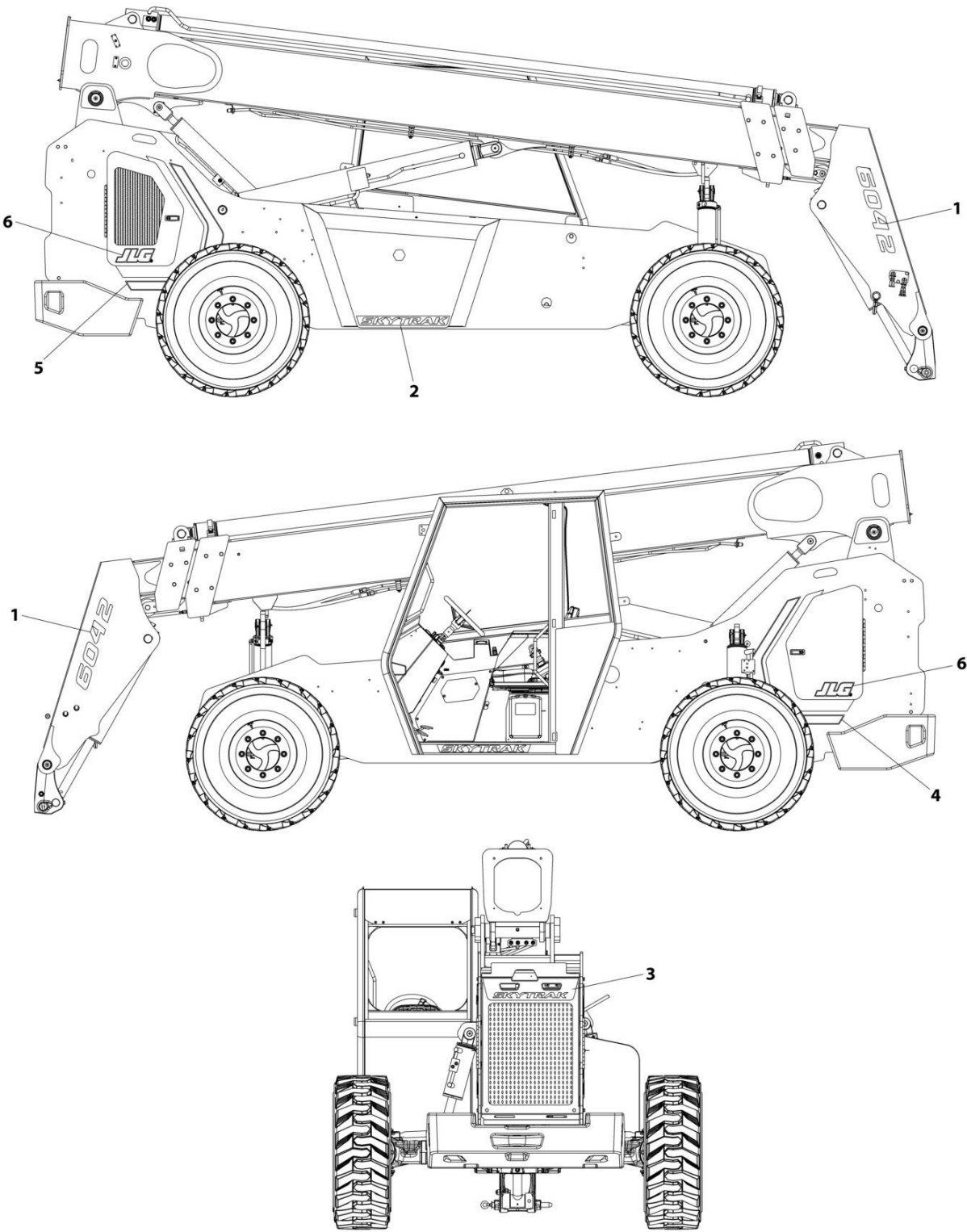
FIGURE 11-6. DECALS INSTALLATION - BRAND
