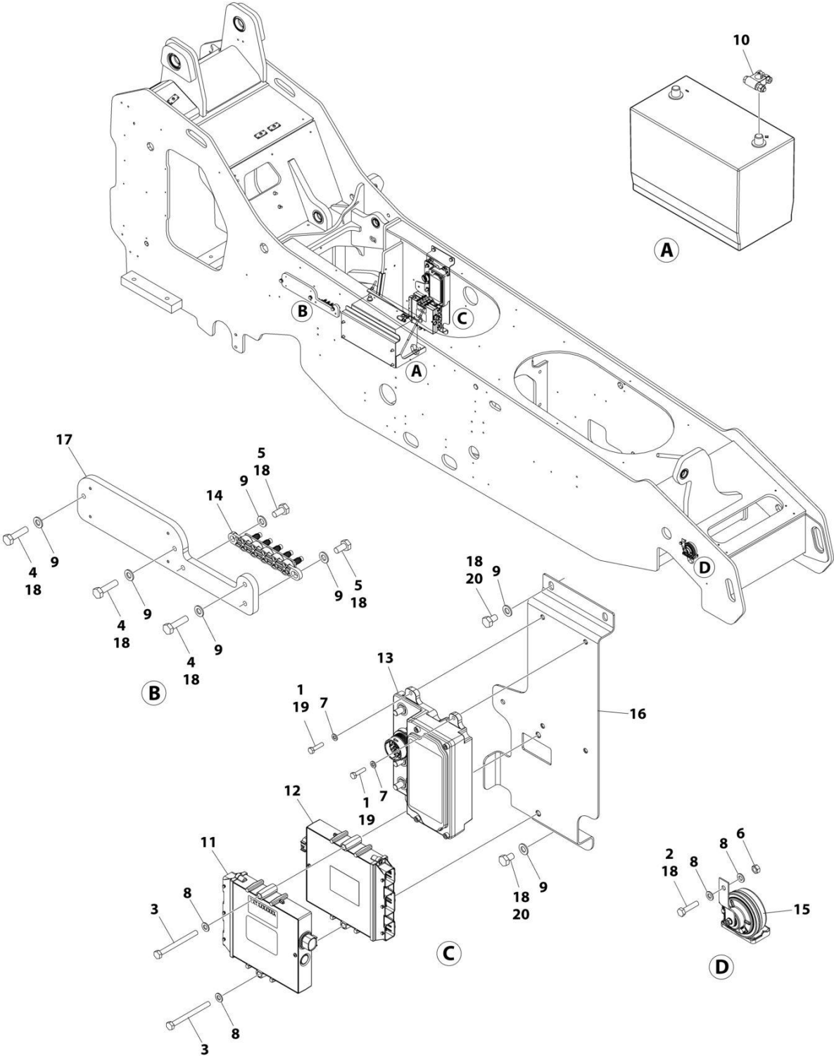
FIGURE 10-24. FRAME ELECTRICAL COMPONENTS INSTALLATION
