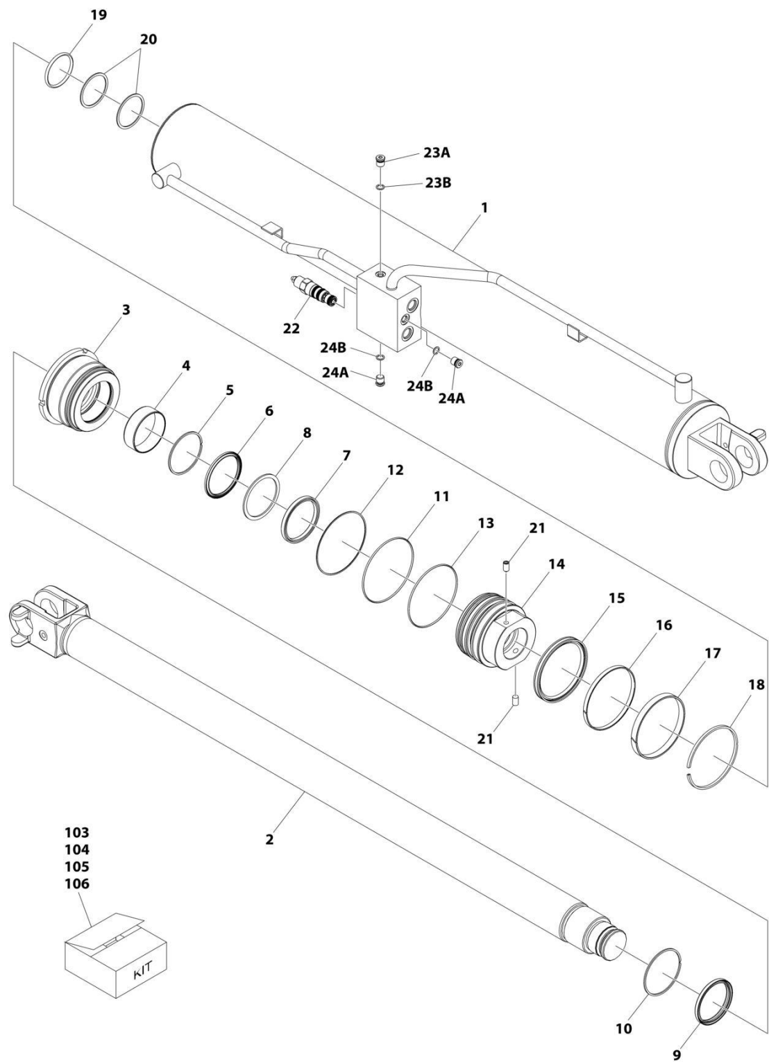
FIGURE 9-7. CYLINDER - LIFT
