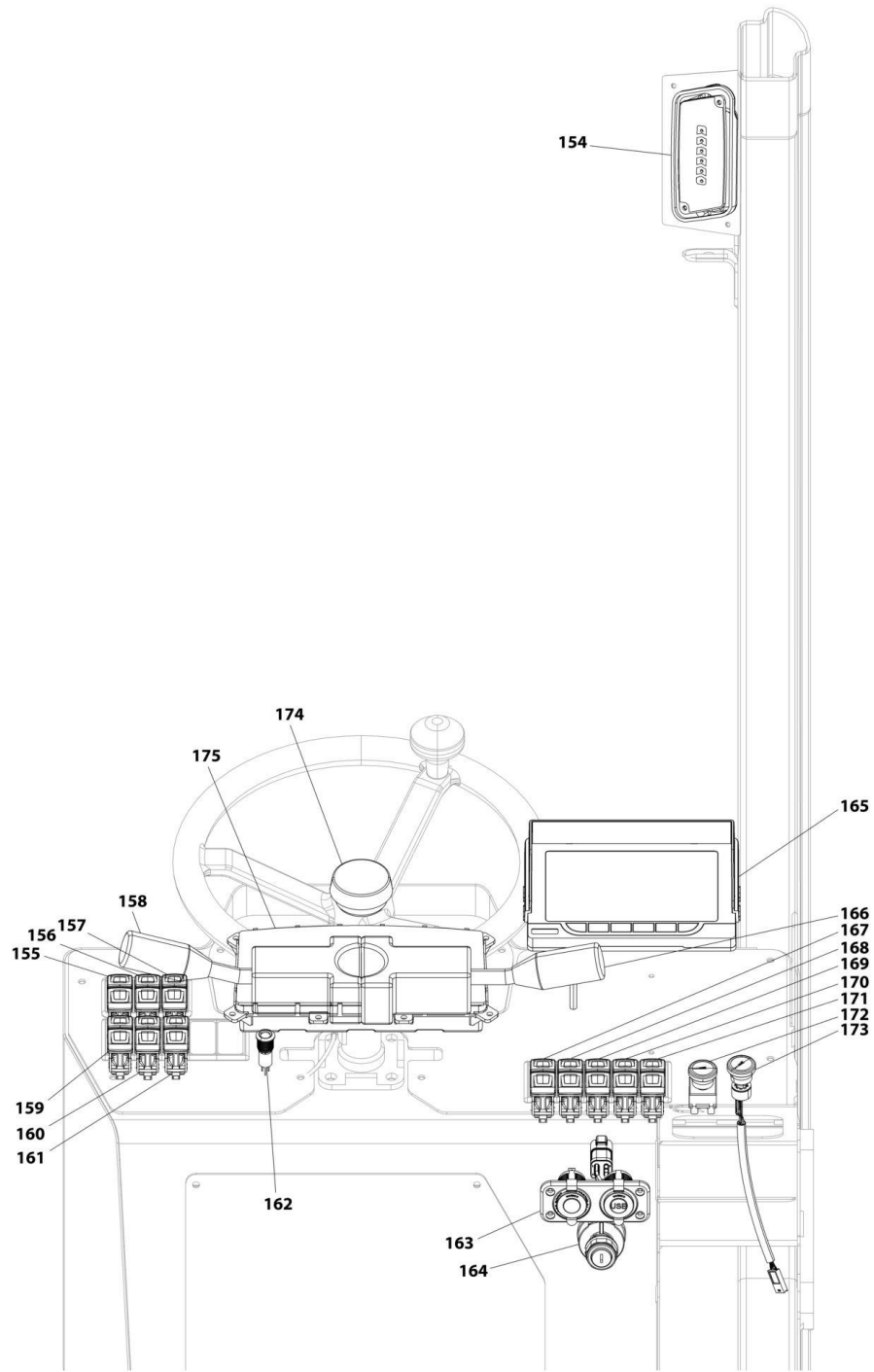
ART_6042-ELECTRICAL_FRAME-CONTROLS
