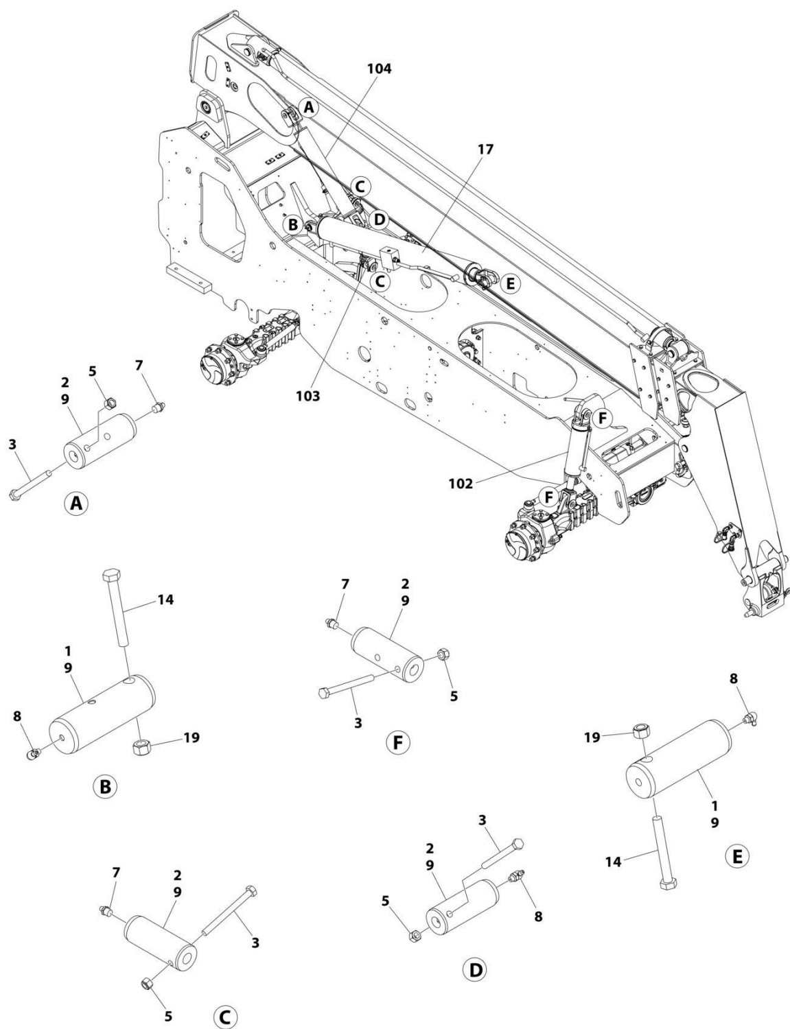
FIGURE 9-6. CYLINDERS INSTALLATION
