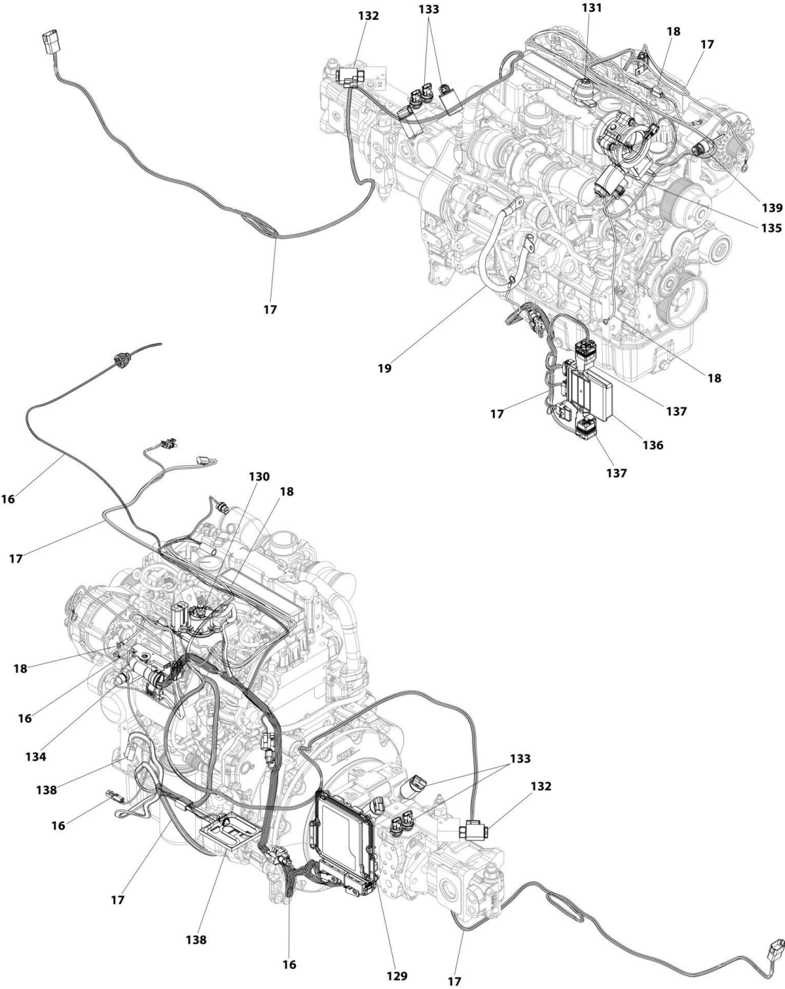
ART_6034-ELECTRICAL_ENGINE_DEUTZ-2.9L4
