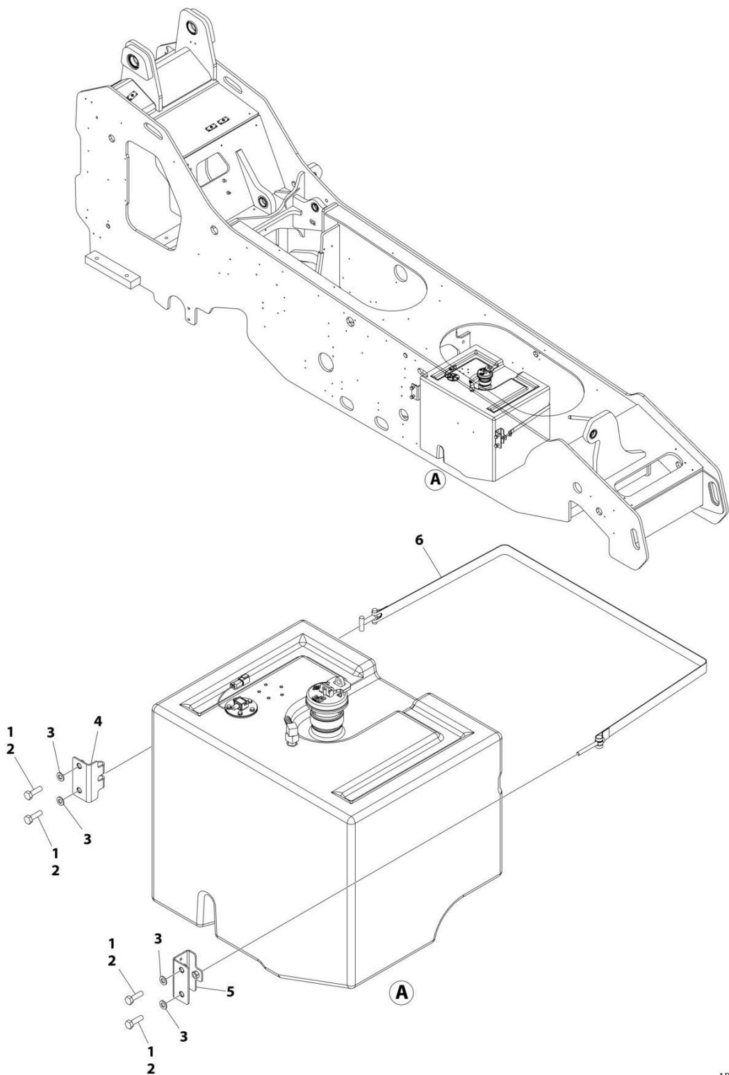
FIGURE 1-4. FUEL TANK MOUNTING INSTALLATION
