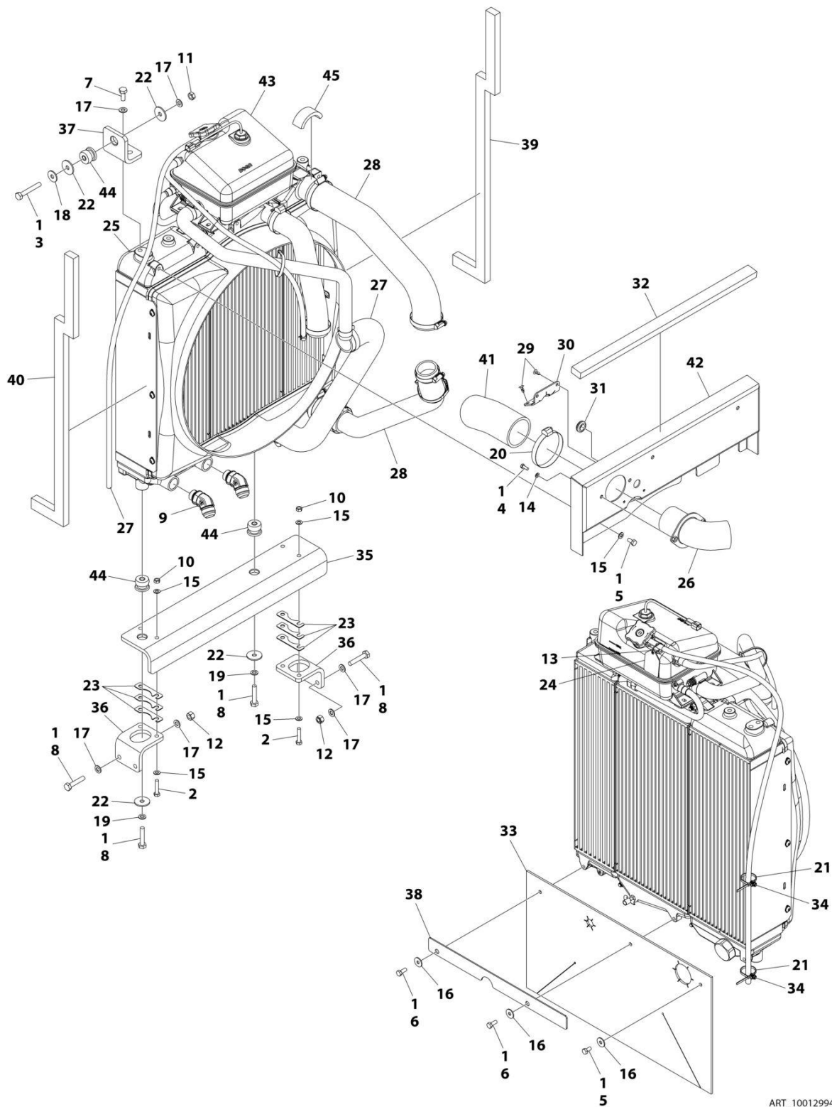
FIGURE 4-11. ENGINE COOLING SYSTEM INSTALLATION
