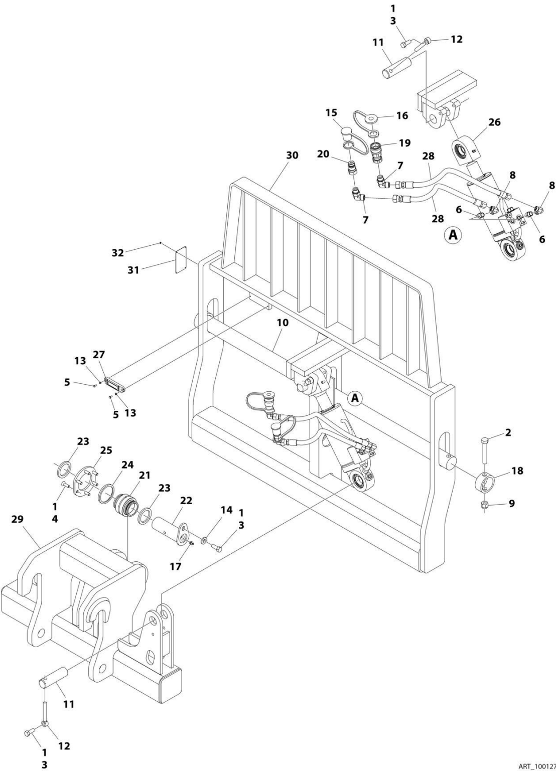
FIGURE 3-18. CARRIAGE ASSEMBLY - 50IN/12000# CAPICITY SIDE TILT
