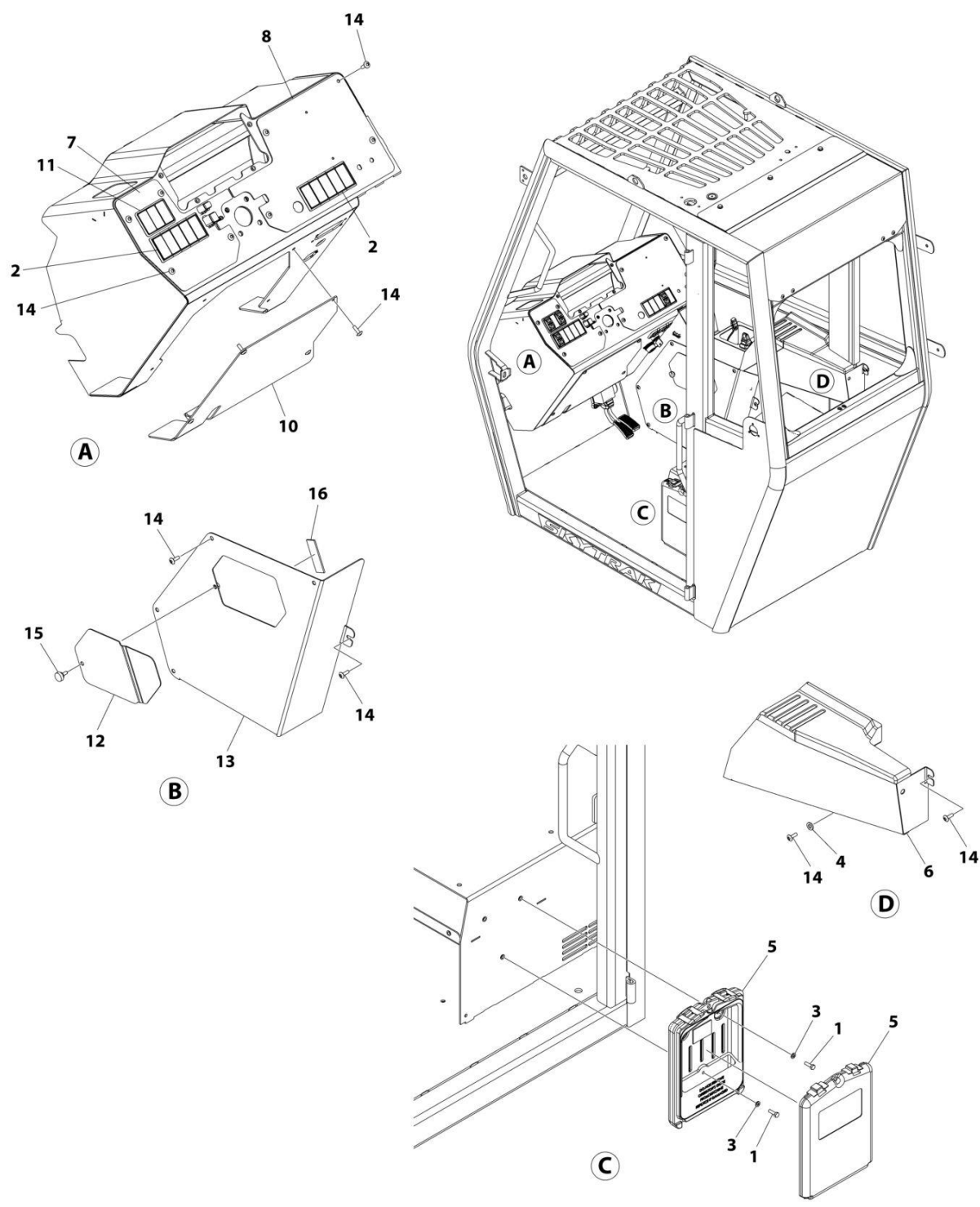
FIGURE 6-4. CAB INTERIOR INSTALLATION
