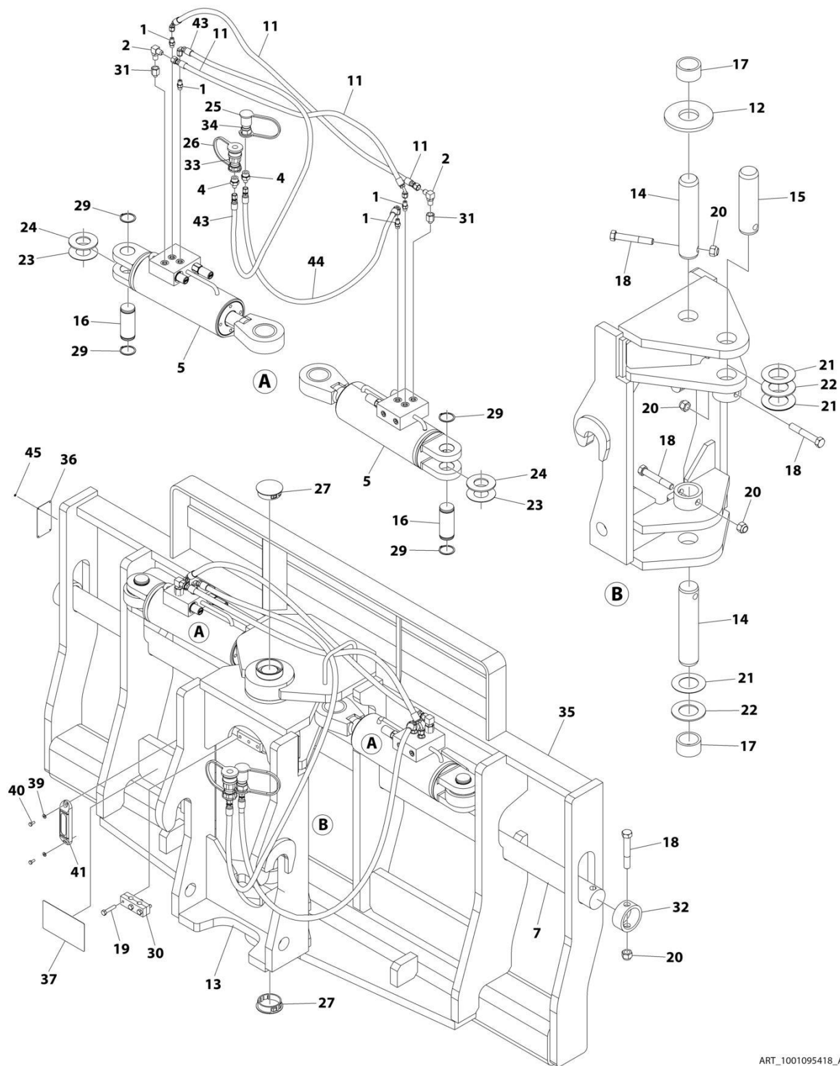
FIGURE 3-23. CARRIAGE ASSEMBLY - 72IN/10000# CAPACITY 90 DEGREE SWING
