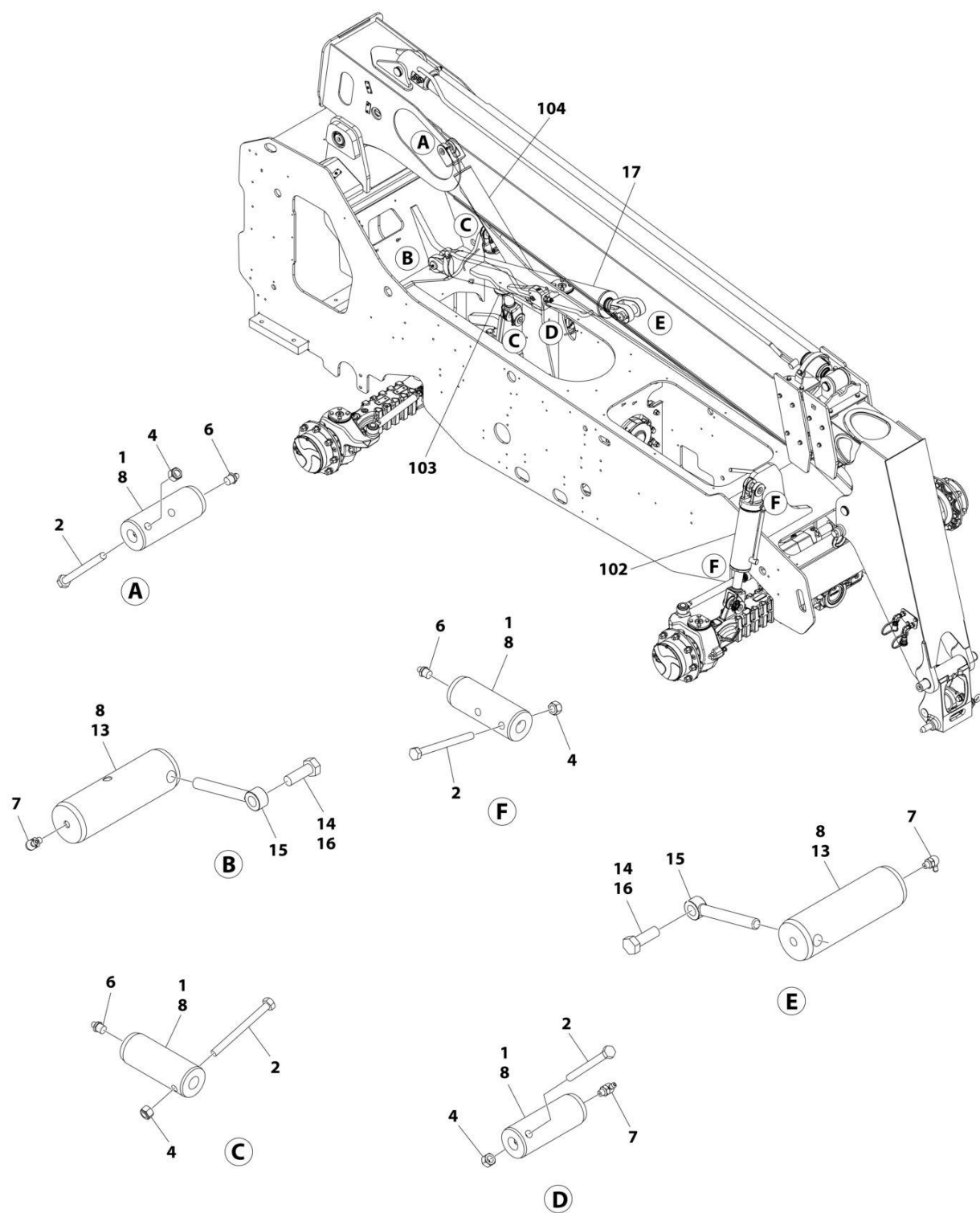
FIGURE 9-6. CYLINDERS INSTALLATION
