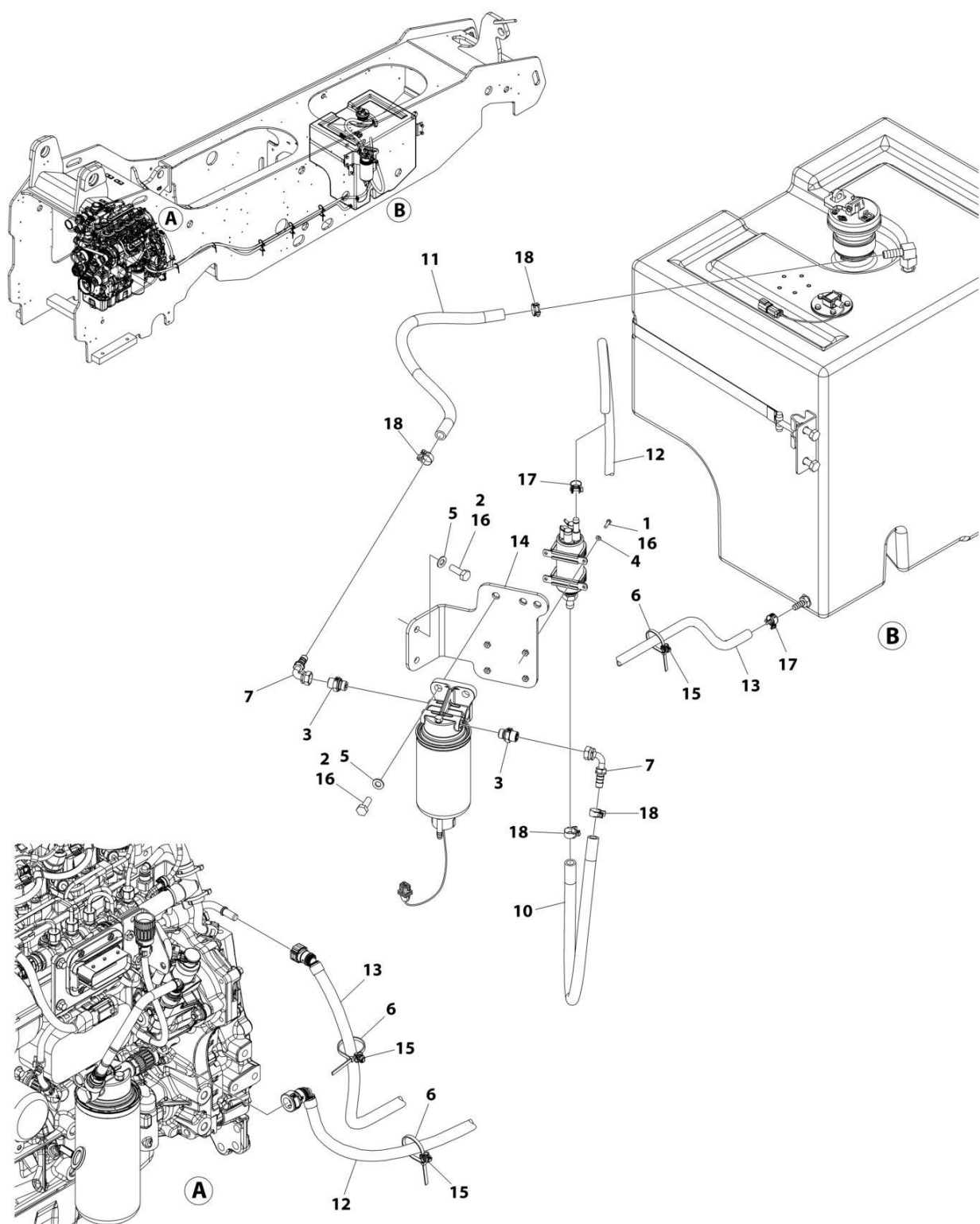
FIGURE 4-8. ENGINE FUEL SYSTEM INSTALLATION (HRC ENGINES)
