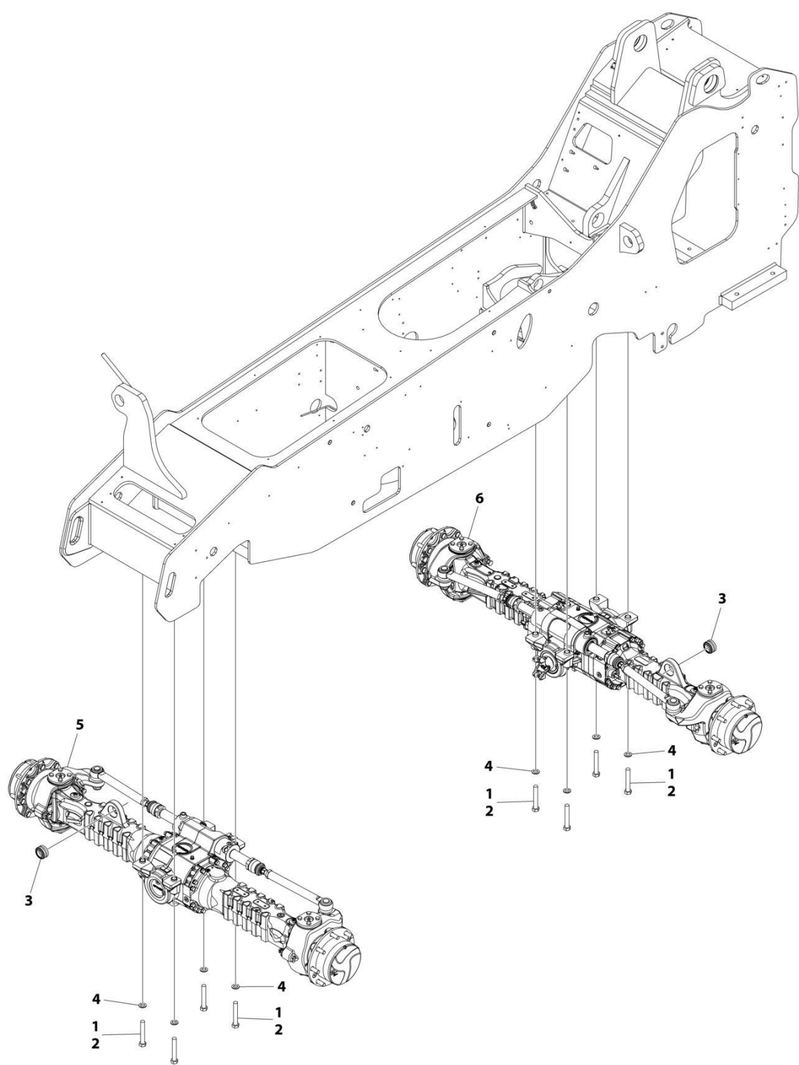
FIGURE 5-1. AXLES INSTALLATION
