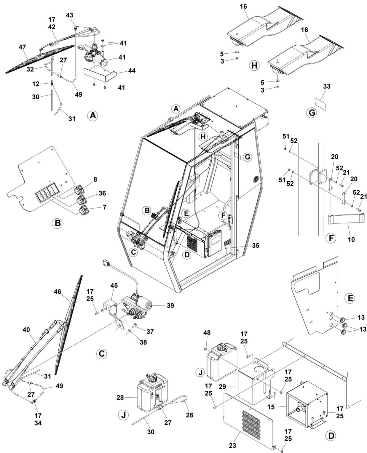
FIGURE 6-13. CAB HEATER INSTALLATION
