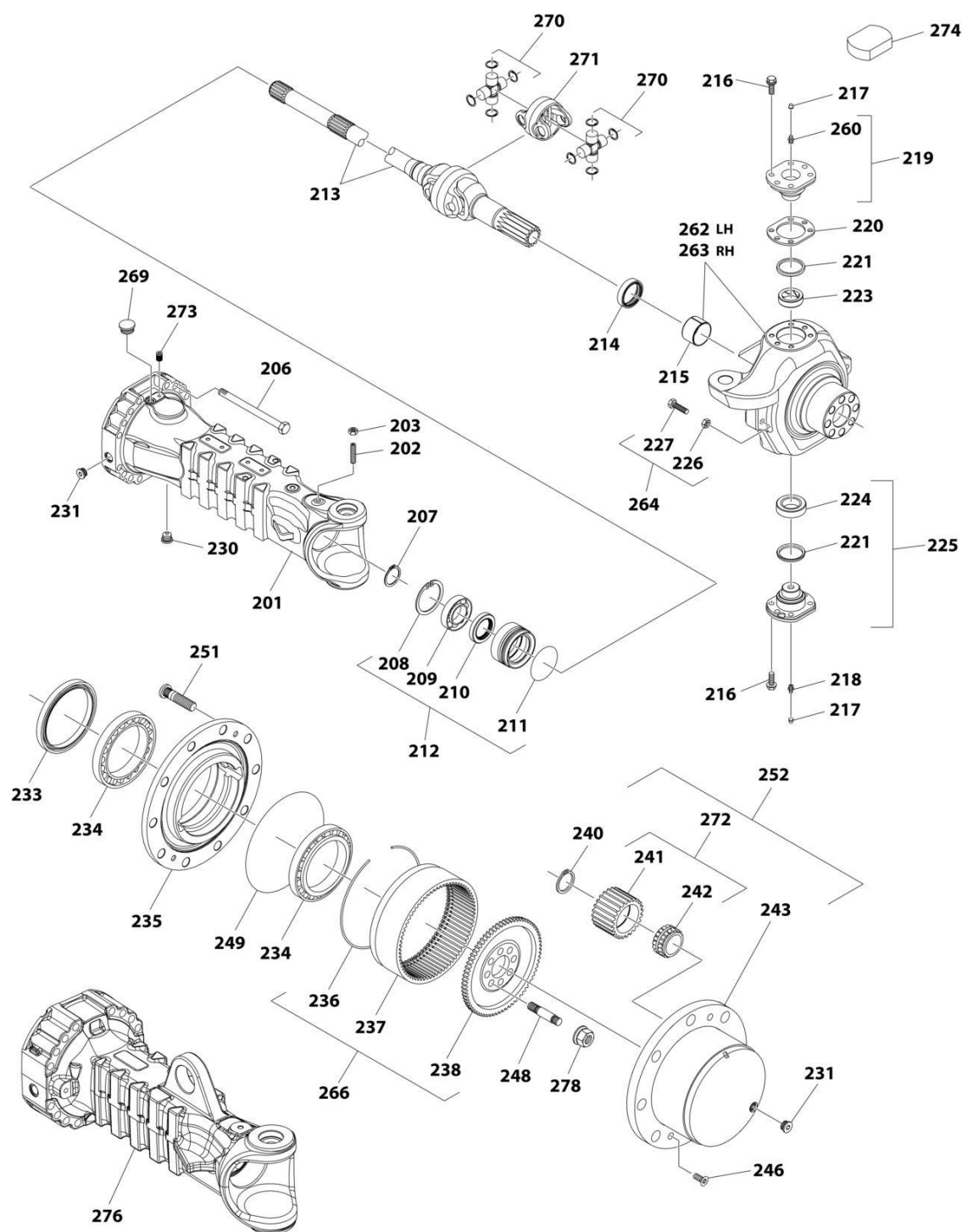
FIGURE 5-12. REAR AXLE ASSEMBLY - HUB REDUCTION
