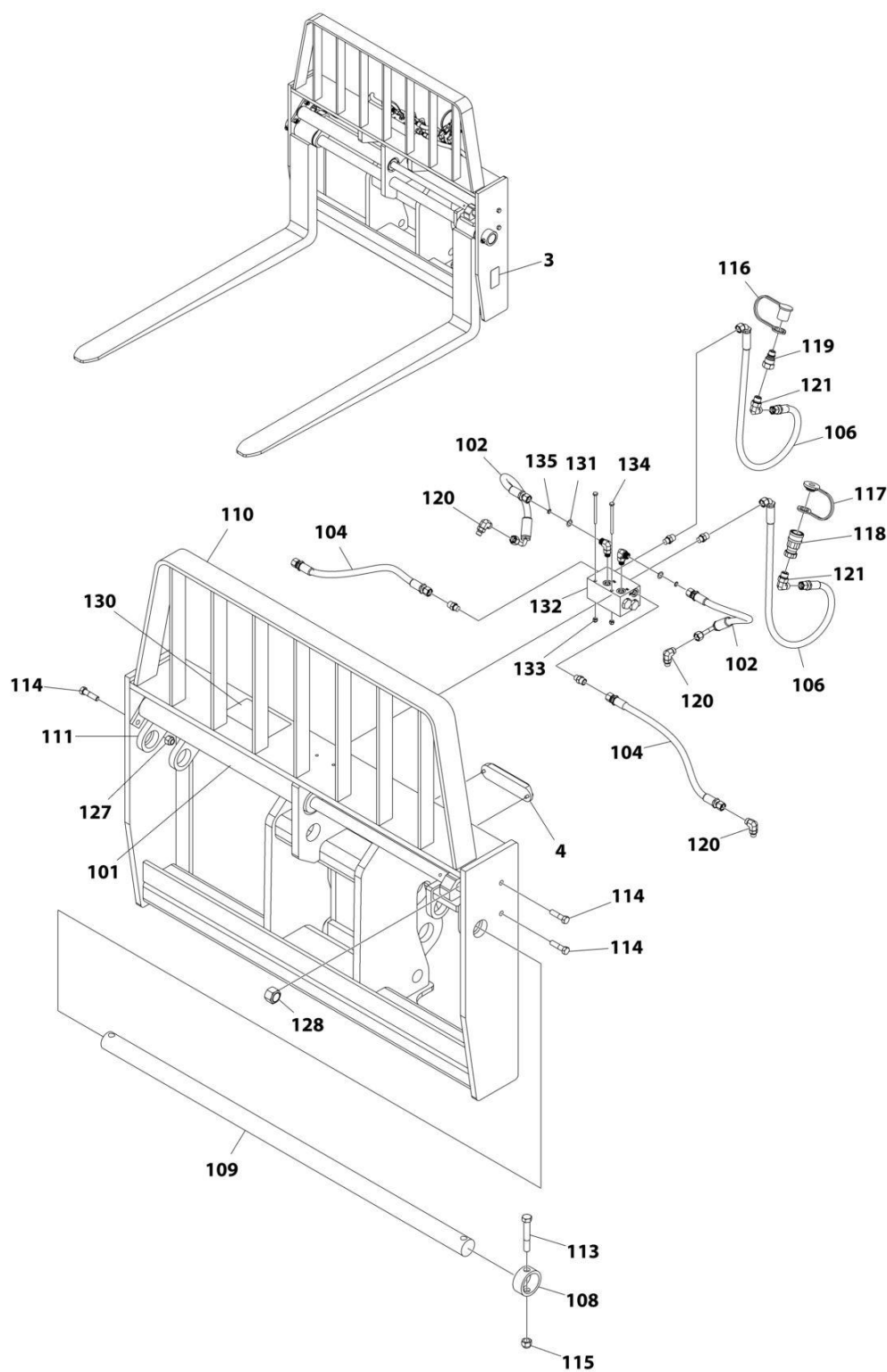
FIGURE 3-17. CARRIAGE ASSEMBLY - 50IN DUAL FORK POSITIONING
