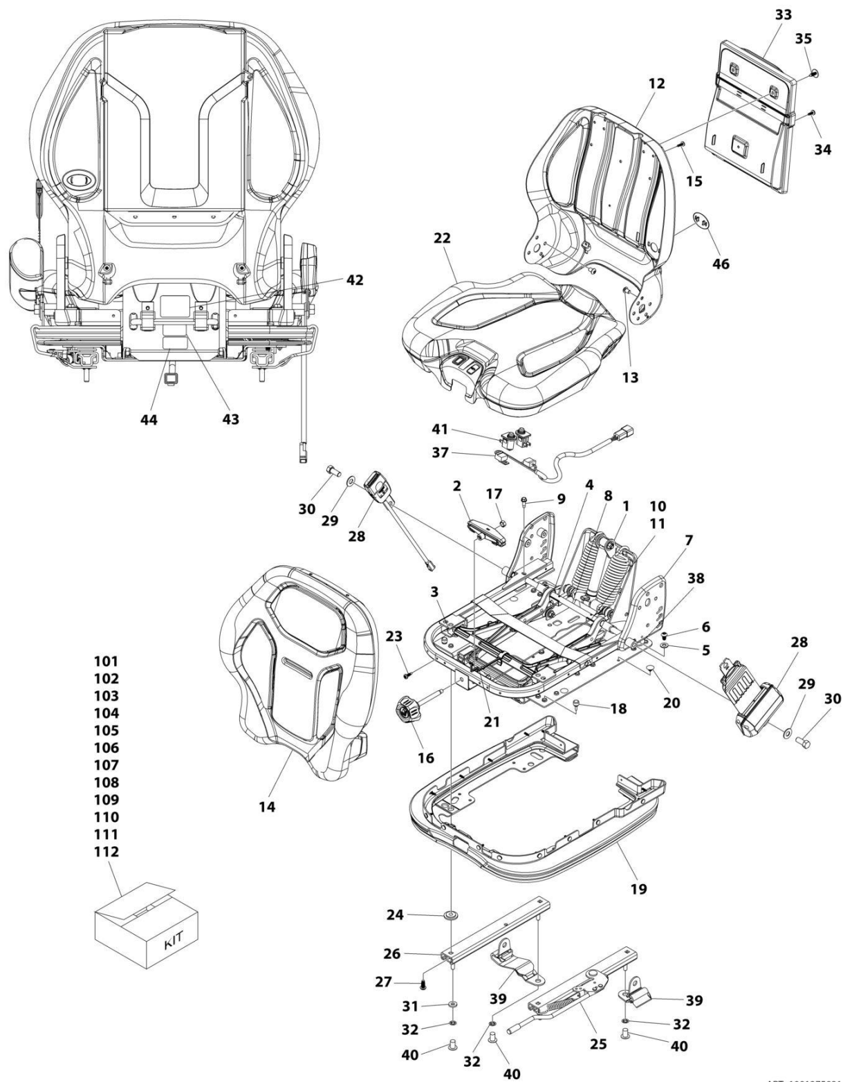
FIGURE 6-29. SEAT ASSEMBLY - VINYL
