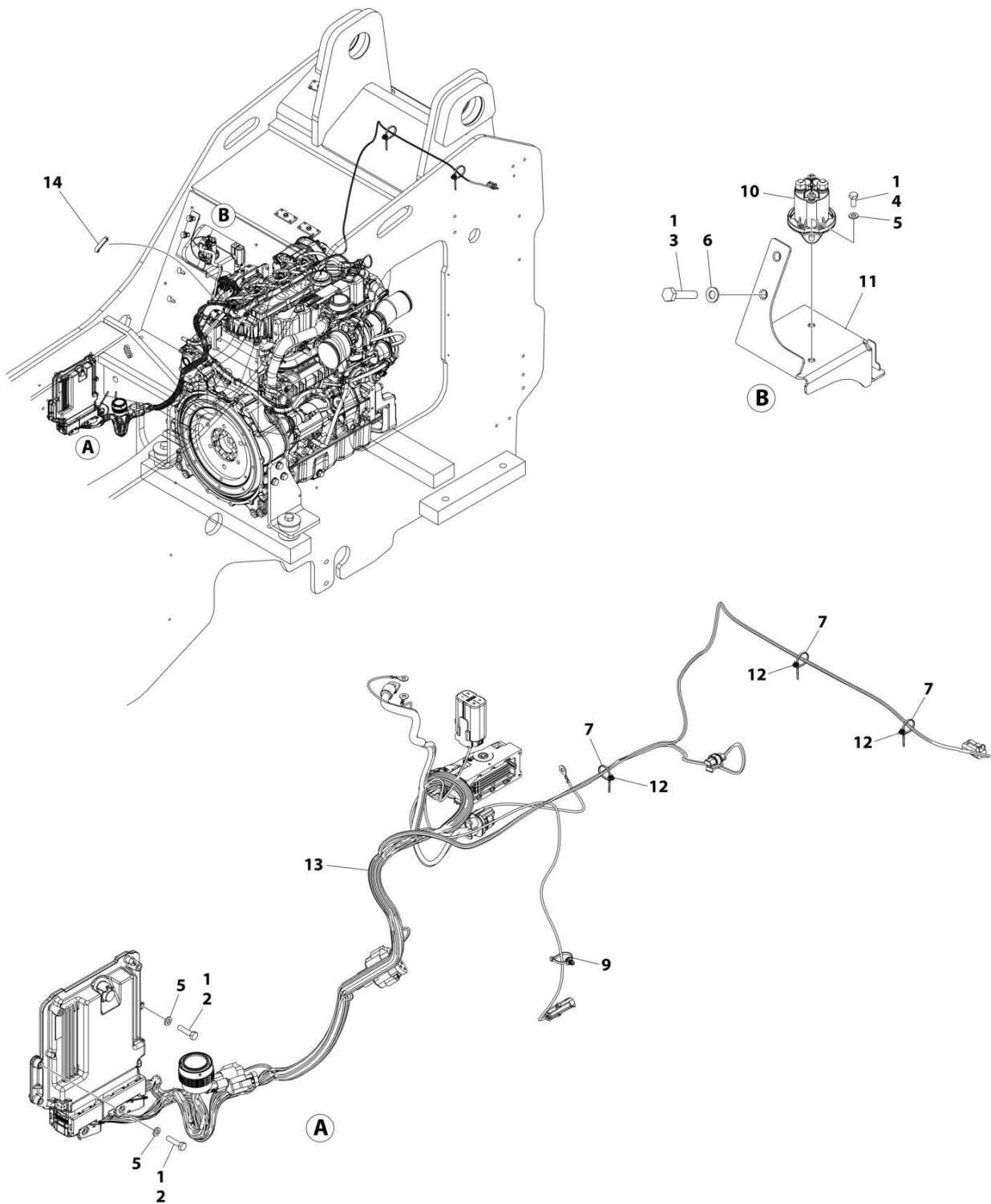
FIGURE 4-6. ENGINE ELECTRICAL INSTALLATION
