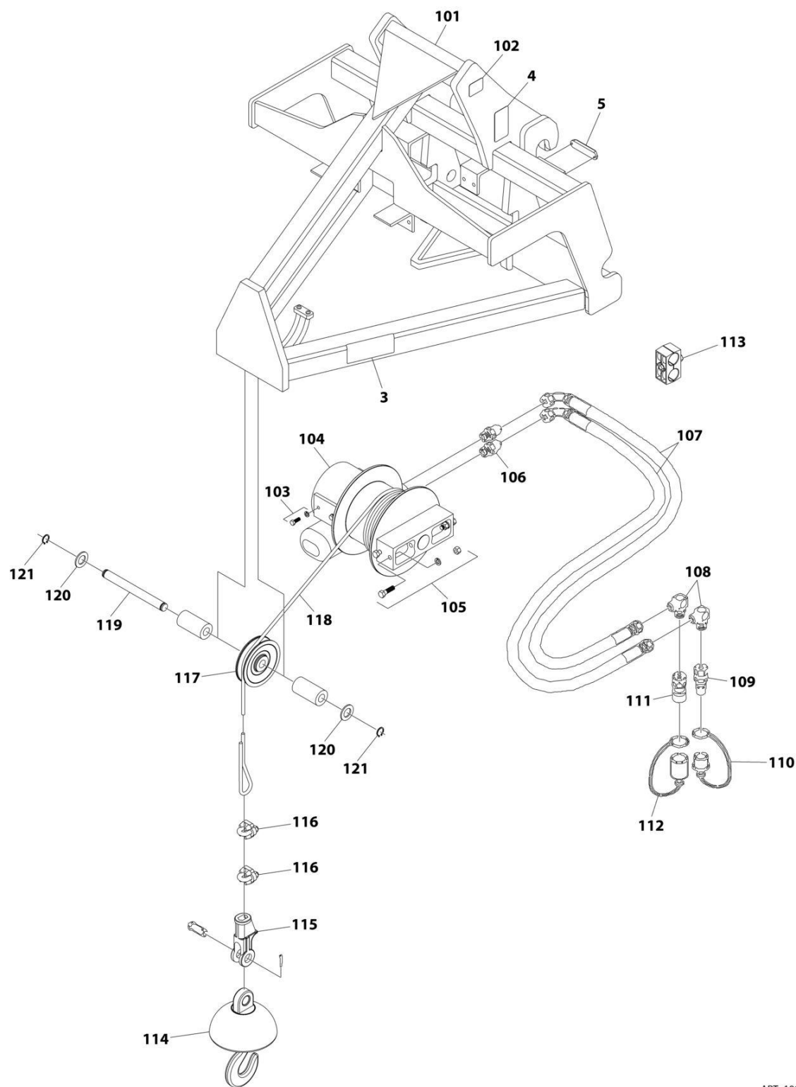
FIGURE 3-7. BOOM - 3 FOOT WITH WINCH
