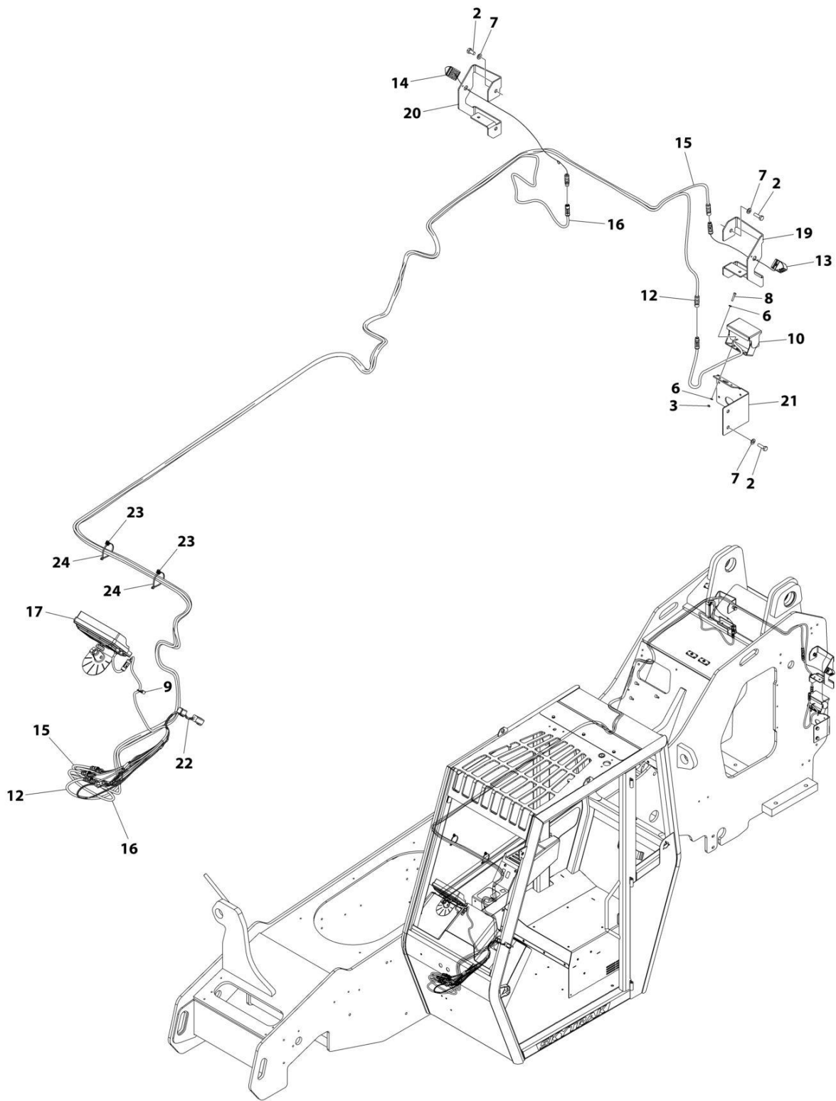
FIGURE 10-17. CAMERA INSTALLATION - BACK UP (WITHOUT LIGHTS)
