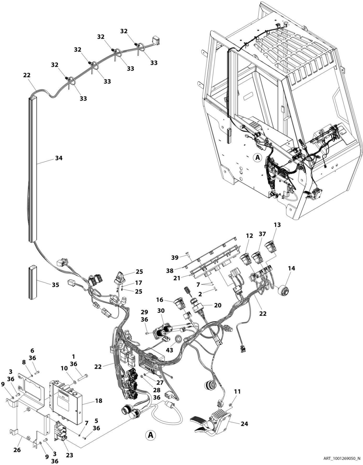
FIGURE 10-11. CAB ELECTRICAL INSTALLATION
