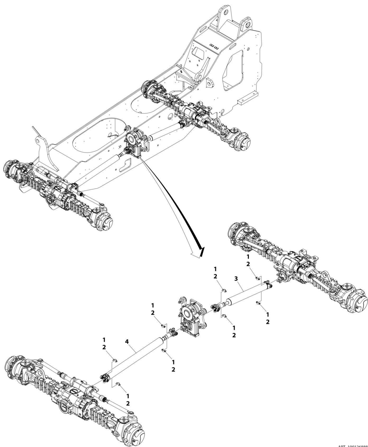
FIGURE 5-21. DRIVESHAFT INSTALLATION (Prior to SN 0160141773)
