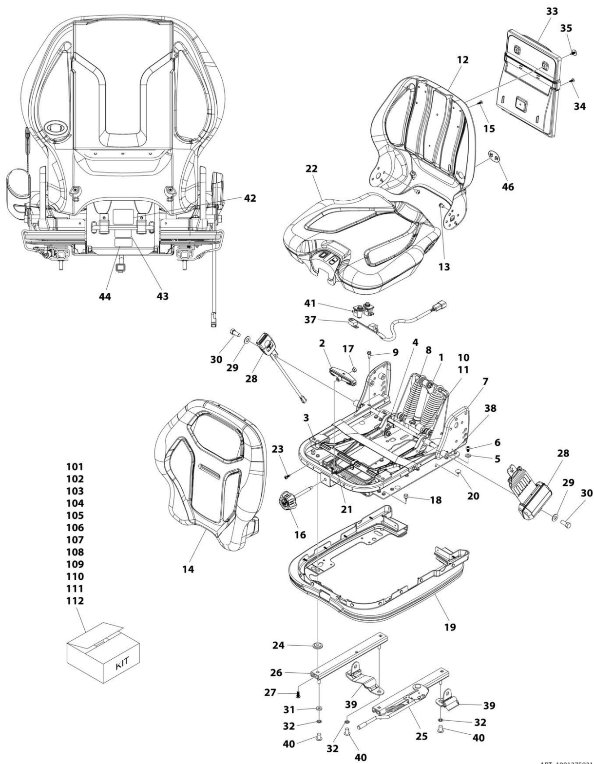
FIGURE 6-28. SEAT ASSEMBLY - VINYL
