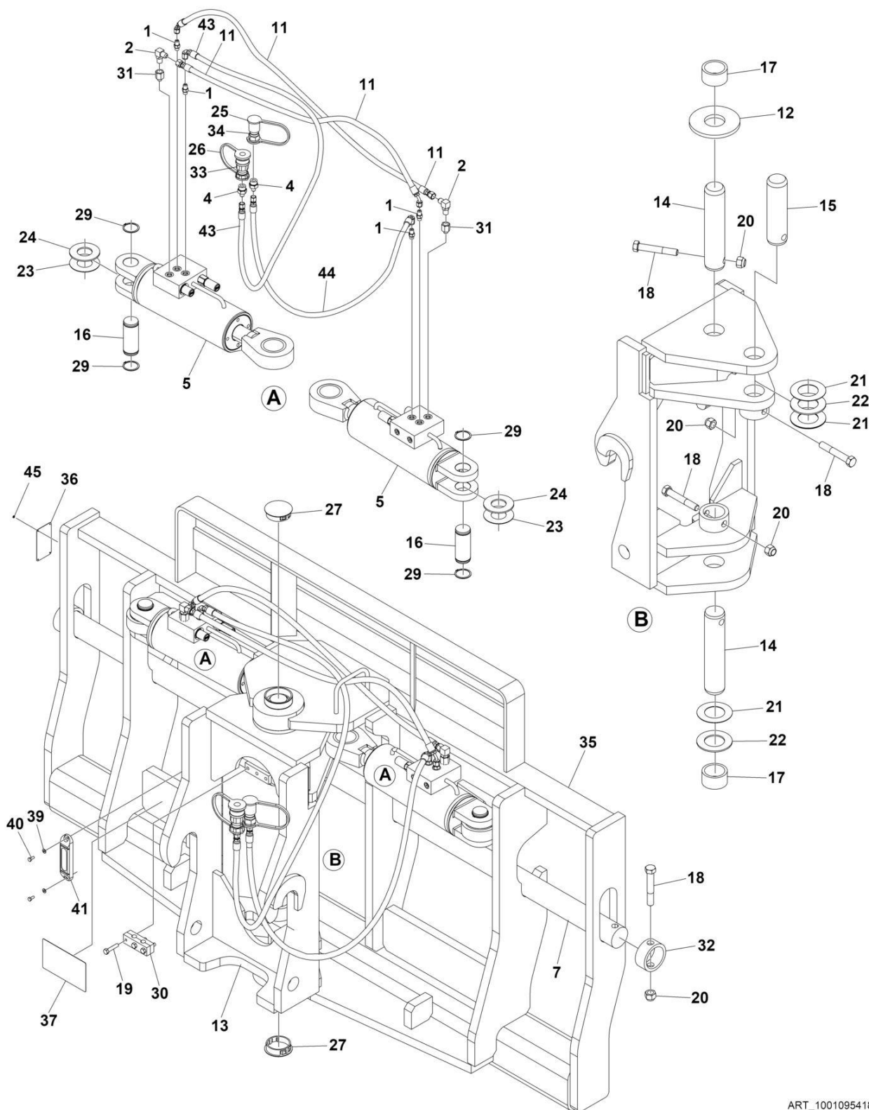
FIGURE 3-31. CARRIAGE ASSEMBLY - 72IN SWING (SN 0160149405 to Present)
