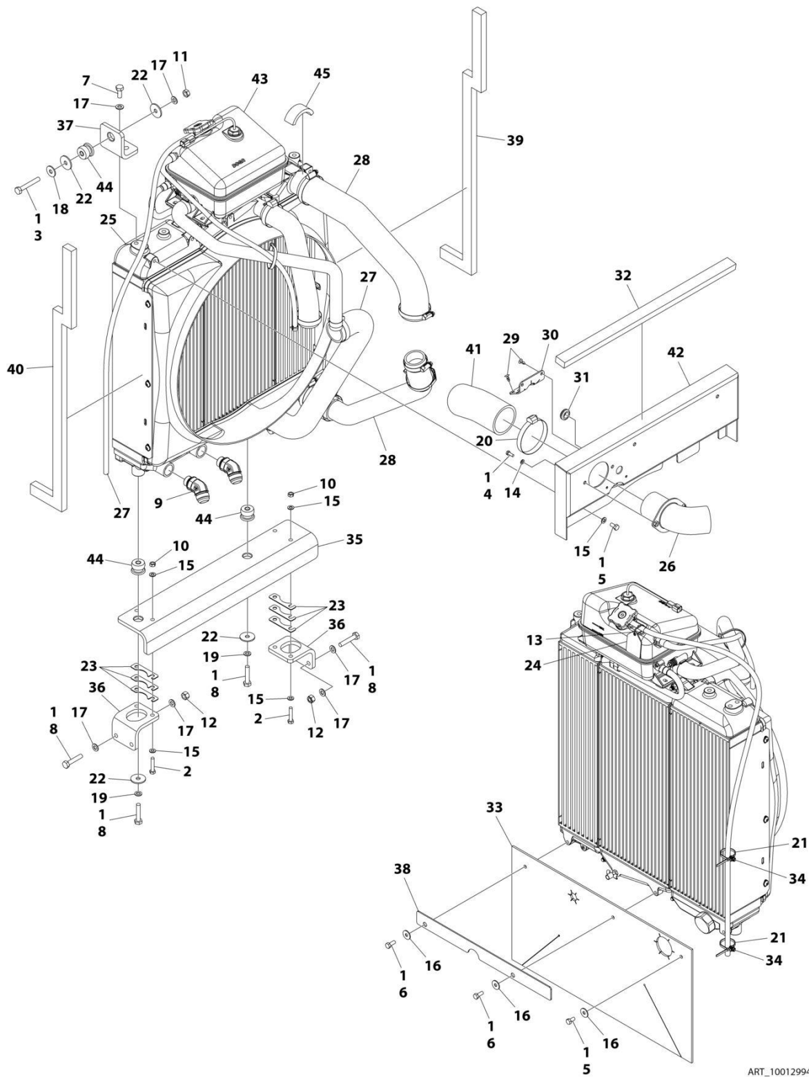
FIGURE 4-12. ENGINE COOLING SYSTEM INSTALLATION
