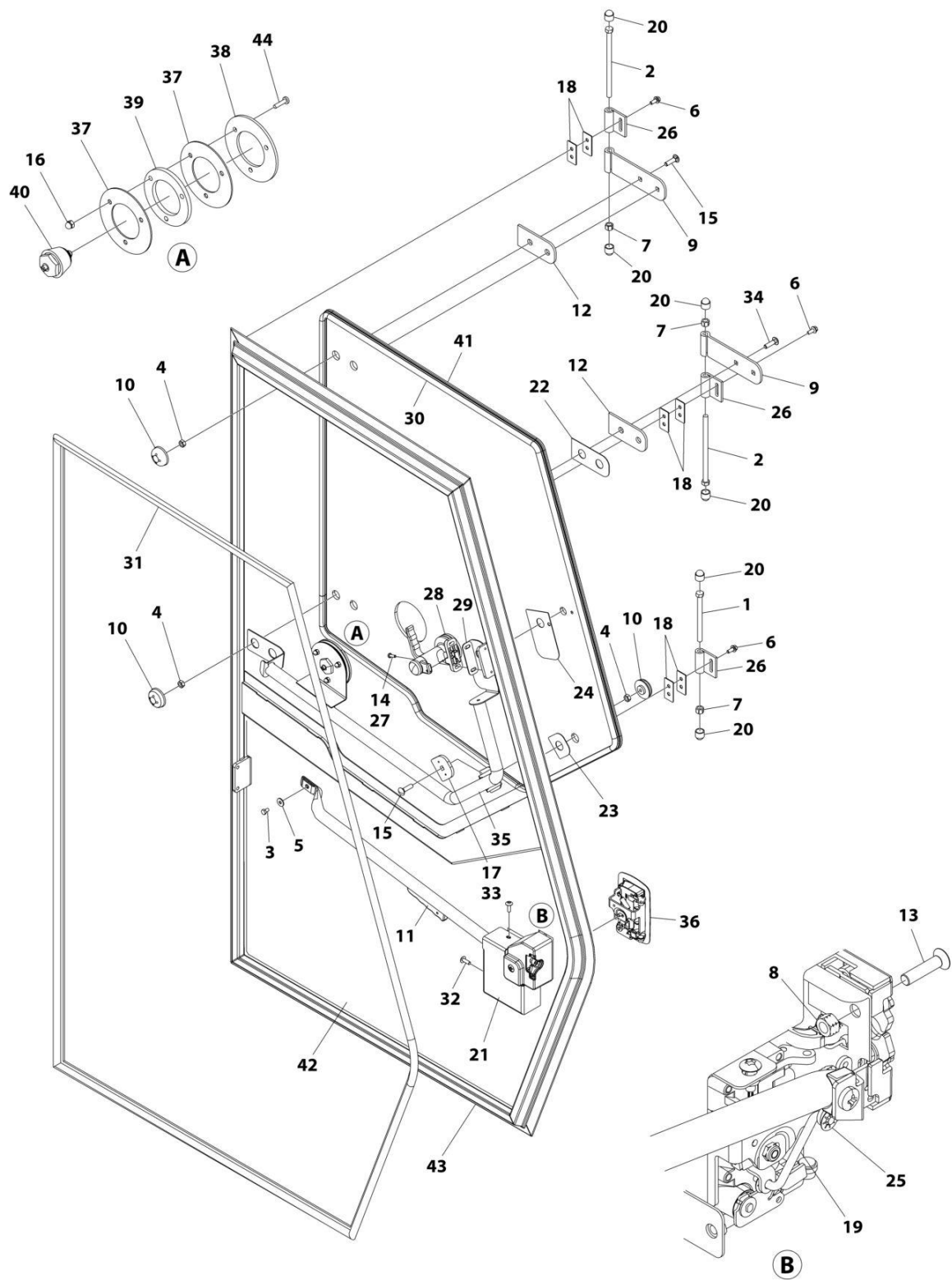
FIGURE 6-14. DOOR ASSEMBLY
