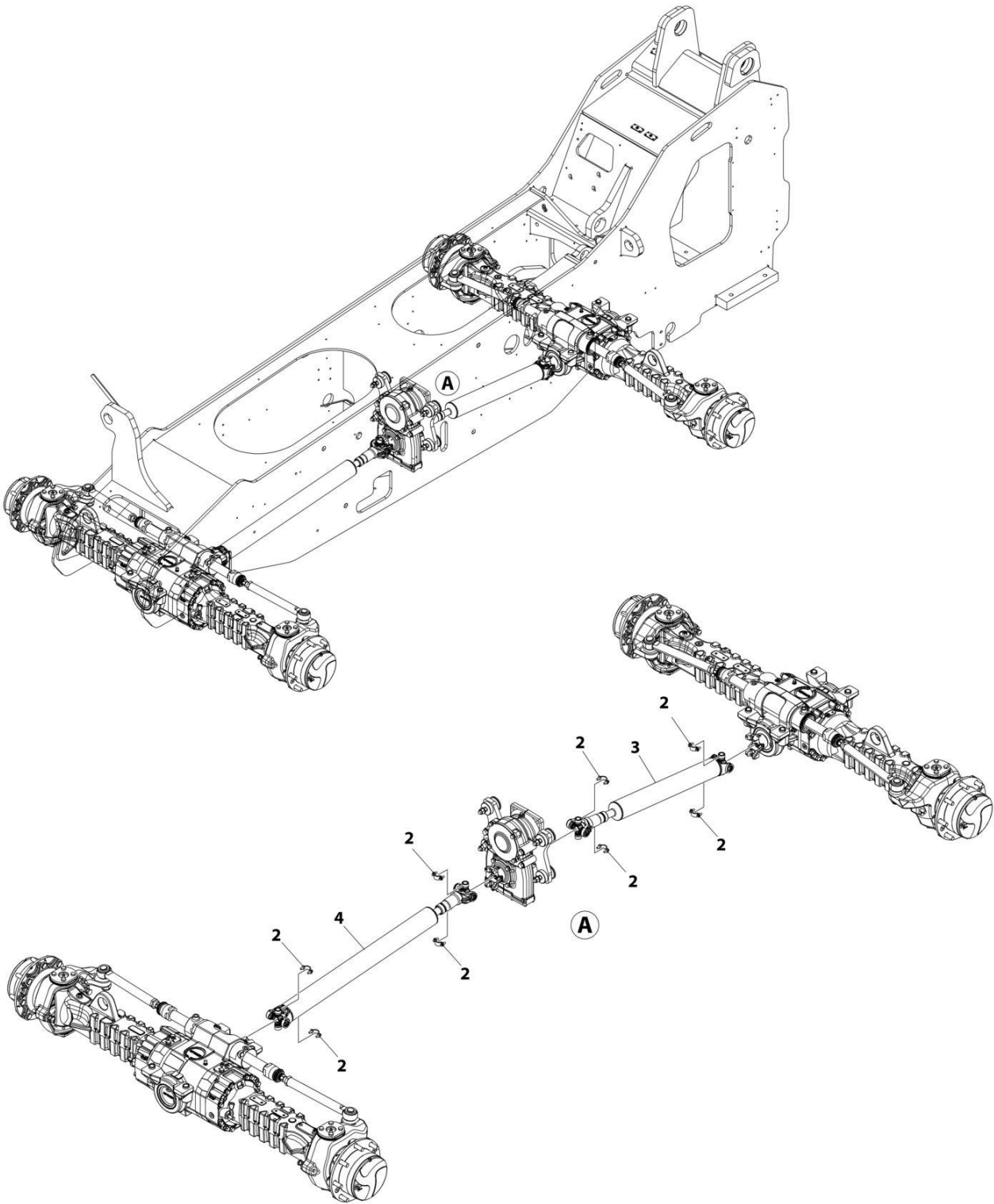
FIGURE 5-22. DRIVESHAFT INSTALLATION (SN 0160141774 to Present)
