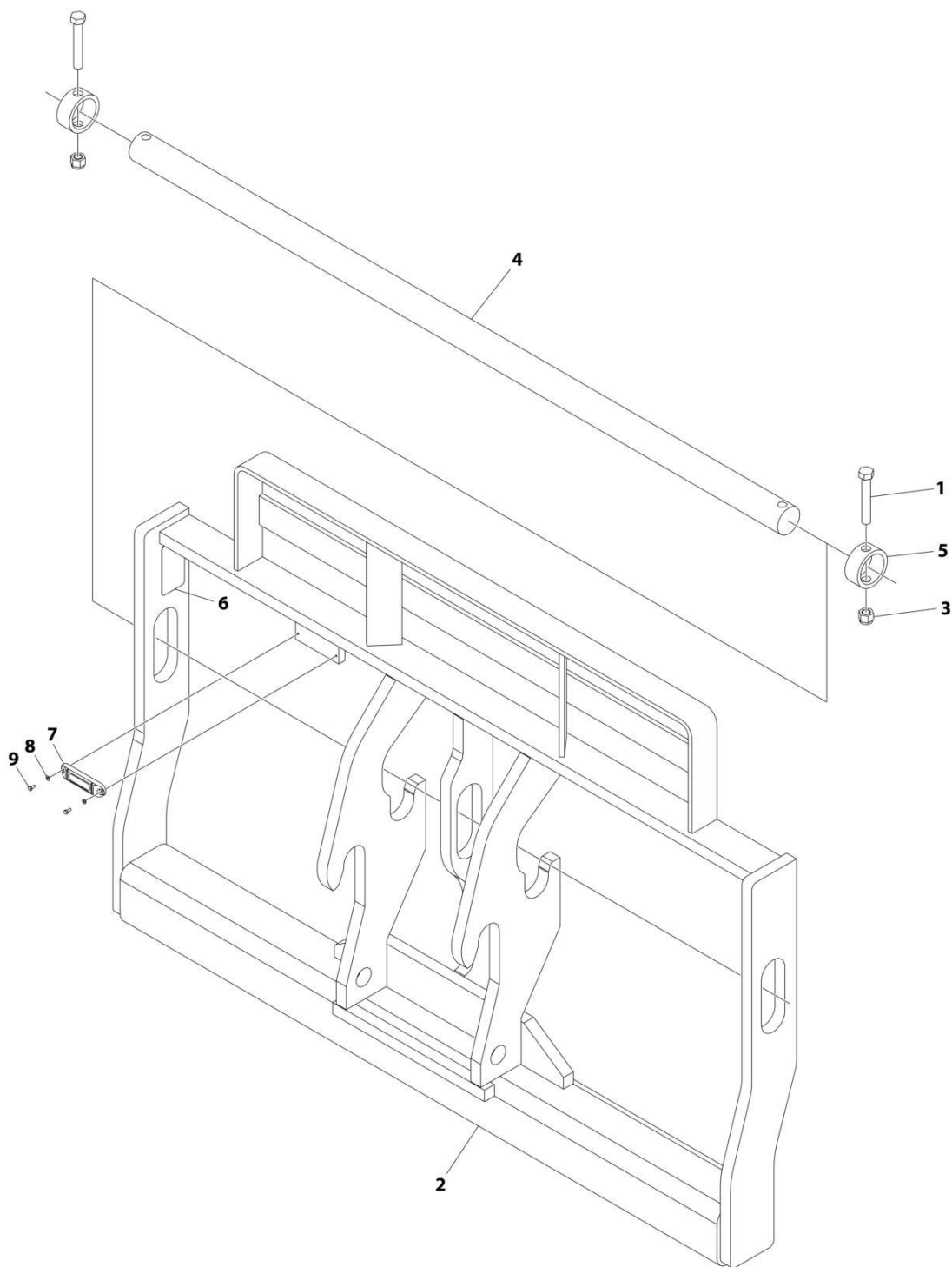
FIGURE 3-22. CARRIAGE ASSEMBLY - 60IN (Prior to SN 0160149404)
