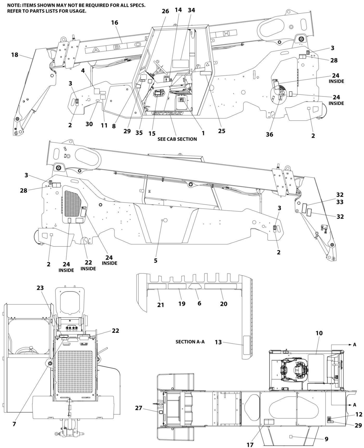
FIGURE 11-5. DECALS INSTALLATION (ENGLISH/FRENCH LANGUAGES) (Prior to SN 0160151503)
