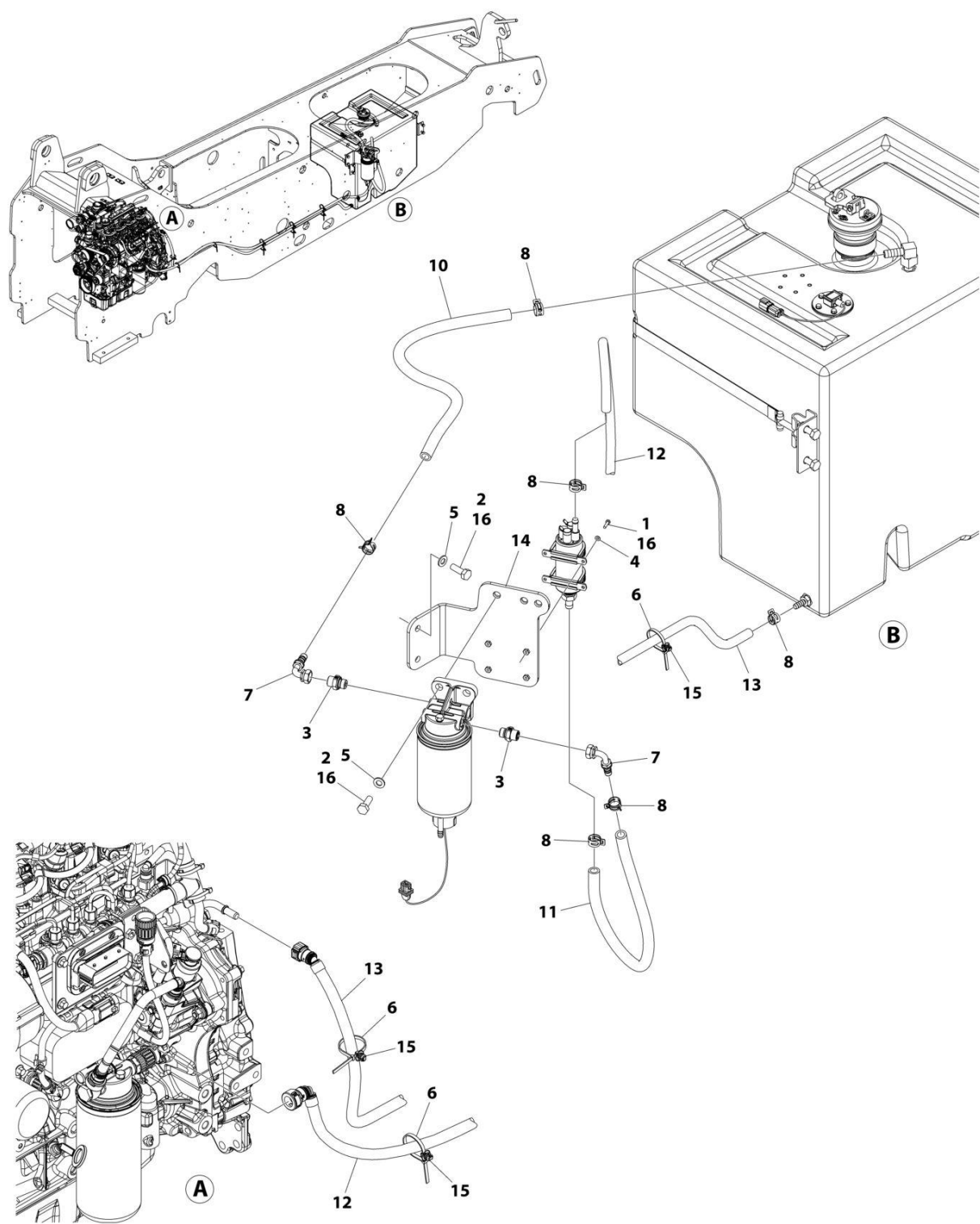
FIGURE 4-8. ENGINE FUEL SYSTEM INSTALLATION (HRC ENGINES) (Prior to SN 0160145923)
