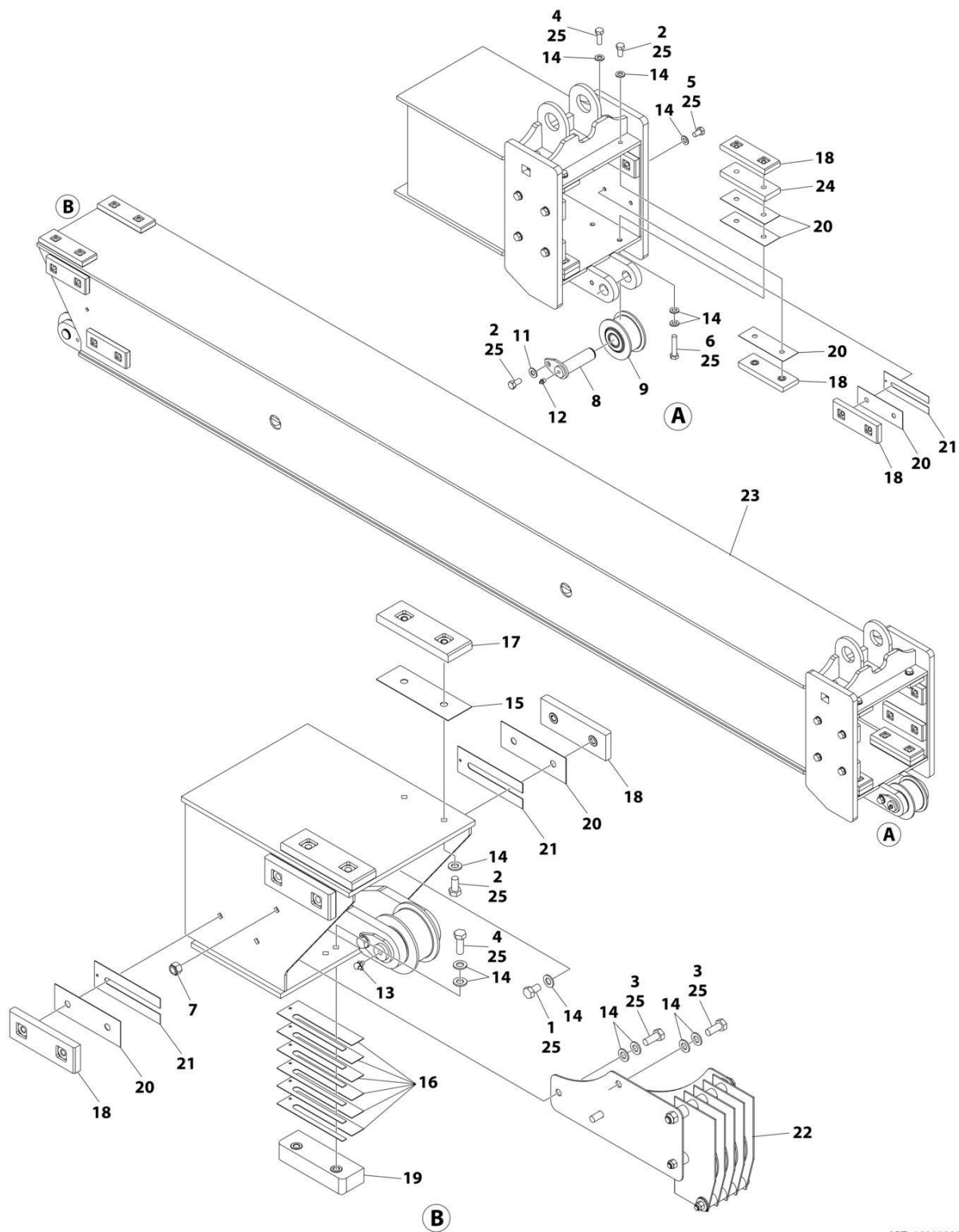
FIGURE 2-4. BOOM MID ASSEMBLY
