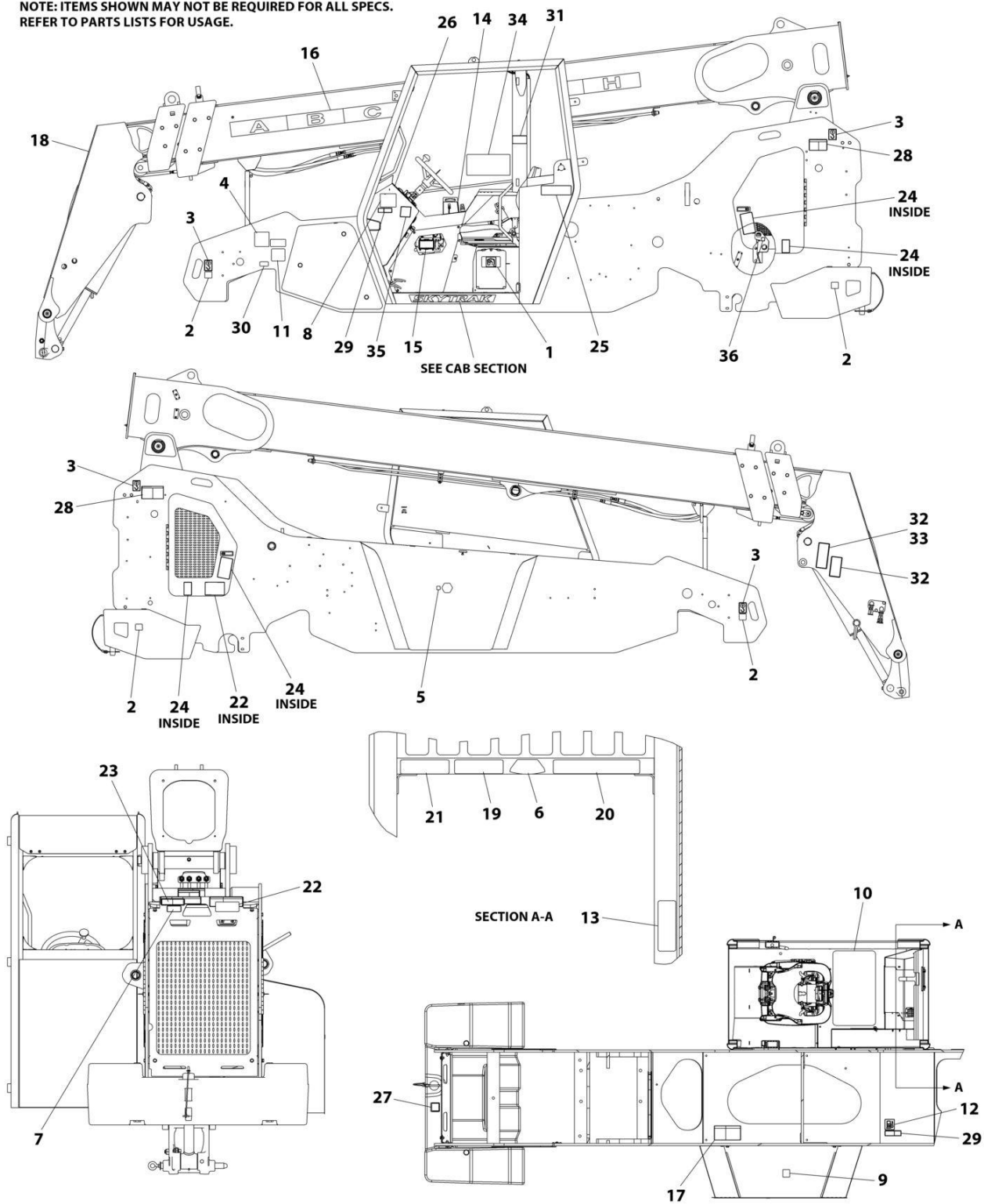
FIGURE 11-1. DECALS INSTALLATION (ANSI SPECS) (Prior to SN 0160151503)
