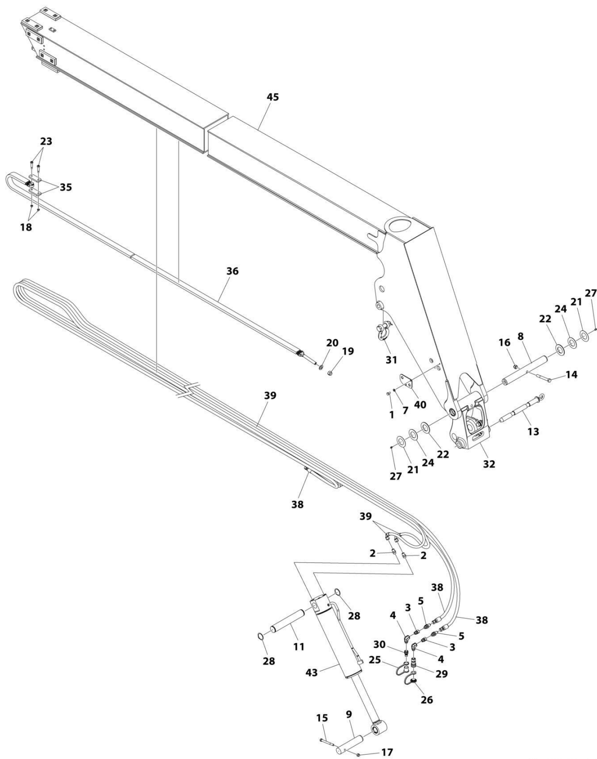
FIGURE 2-2. BOOM ASSEMBLY
