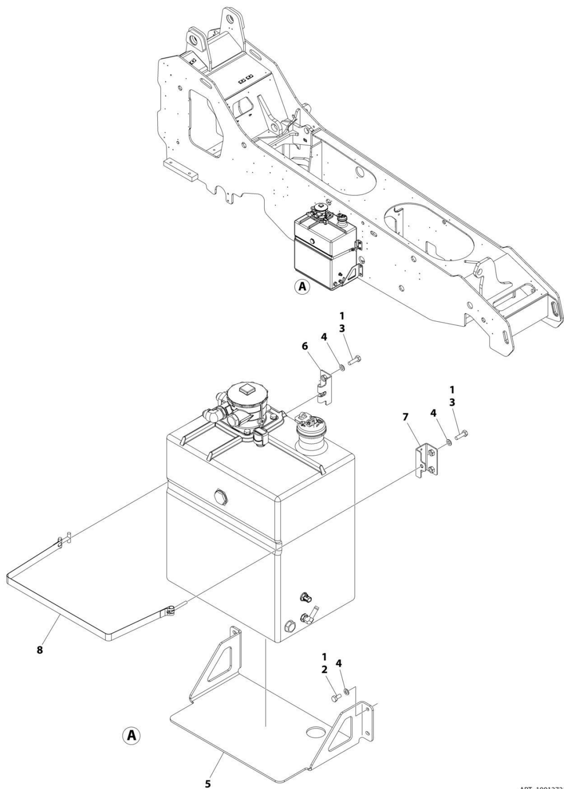
FIGURE 1-8. HYDRAULIC TANK MOUNTING INSTALLATION
