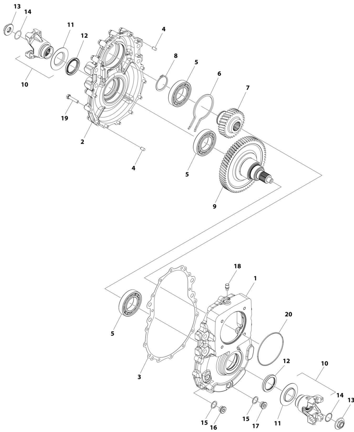
FIGURE 5-28. GEARBOX ASSEMBLY
