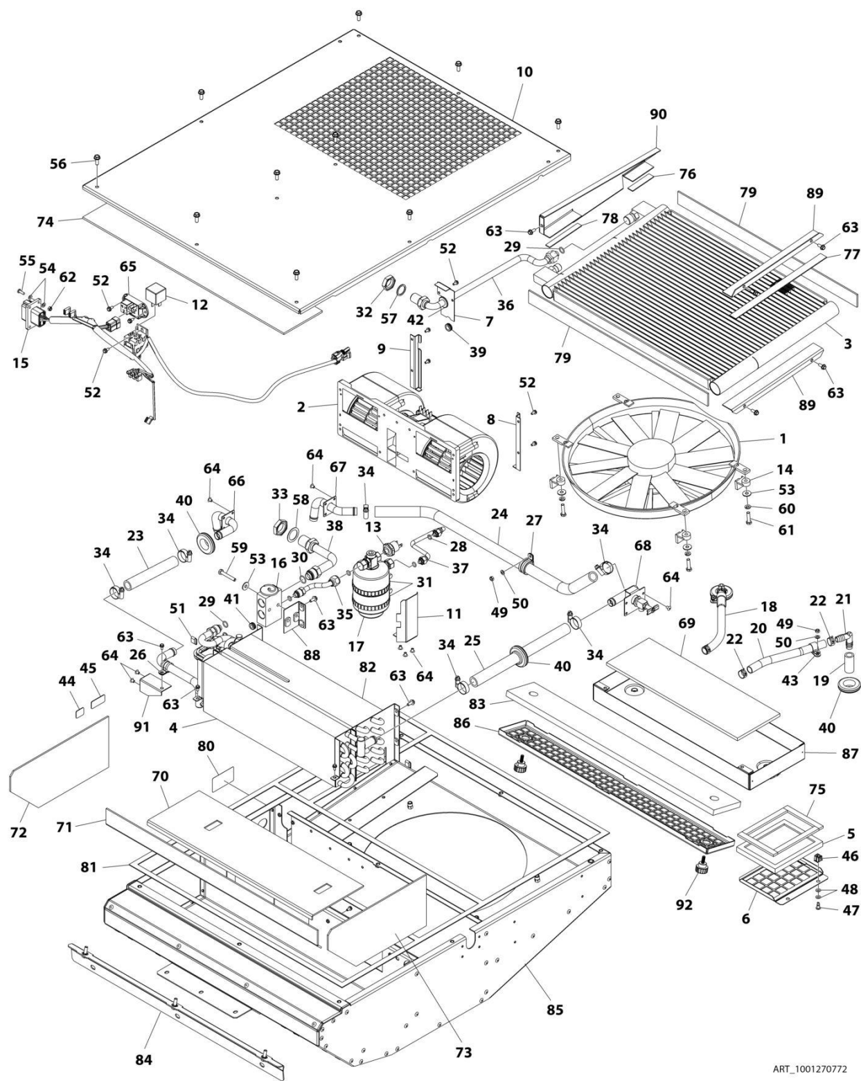
FIGURE 6-21. HVAC ASSEMBLY
