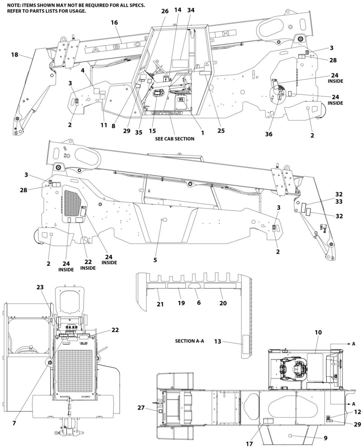
FIGURE 11-7. DECALS INSTALLATION (ENGLISH/SPANISH LANGUAGES) (Prior to SN 0160151503)
