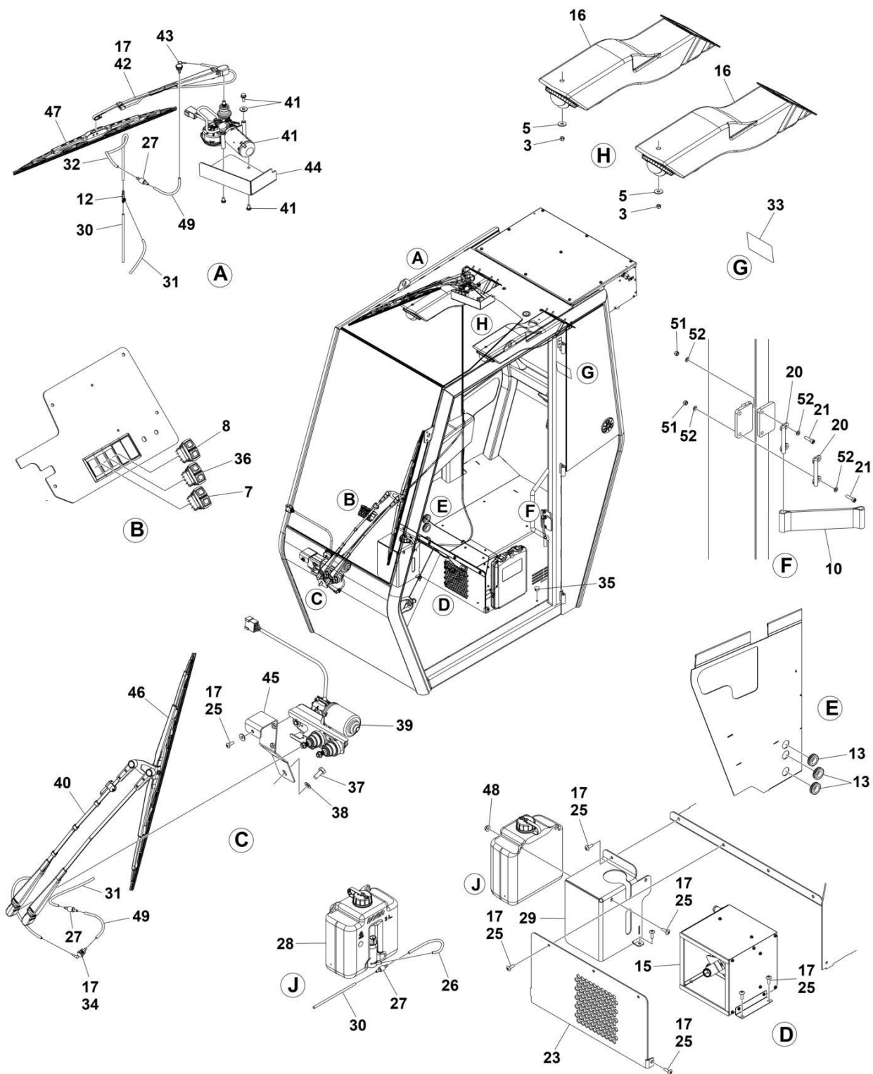
FIGURE 6-8. CAB HEATER INSTALLATION
