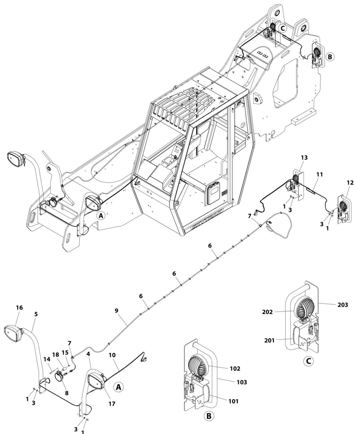
FIGURE 10-29. LIGHTS – ROADLIGHTS INSTALLATION
