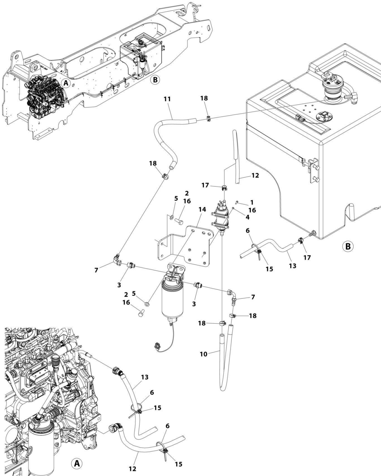
FIGURE 4-9. ENGINE FUEL SYSTEM INSTALLATION (HRC ENGINES) (SN 0160145924 to Present, SN 0160145554 through 0160145555, SN 0160145713 through 0160145715, SN 0160145718 through 0160145721, SN 0160145723 through 0160145724, SN 0160145731 through 0160145735, SN 0160145739 through 0160145747, SN 0160145749 through 0160145753, SN 0160145759 through 0160145760, SN 0160145768 through 0160145772, SN 0160145777 through 0160145778)
