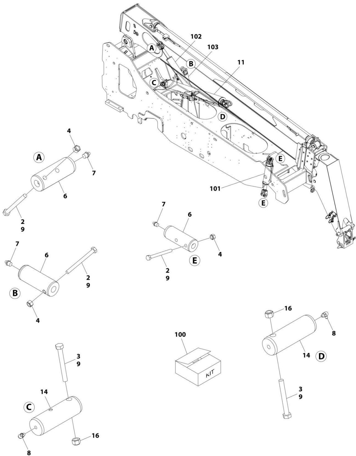
FIGURE 9-6. CYLINDER INSTALLATION
