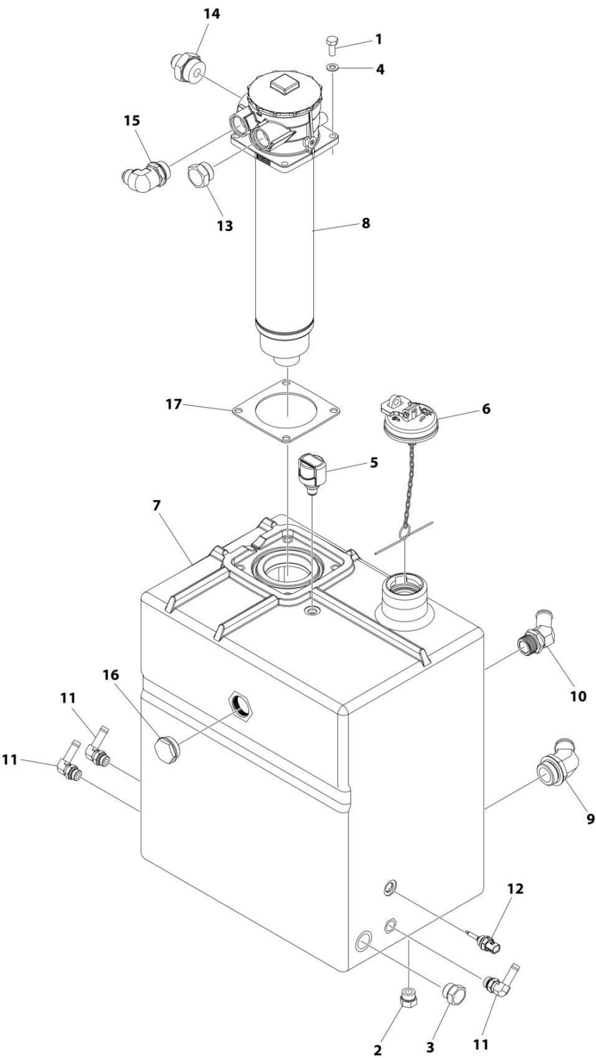
FIGURE 1-5. HYDRAULIC TANK ASSEMBLY (Prior to SN 0160147318)
