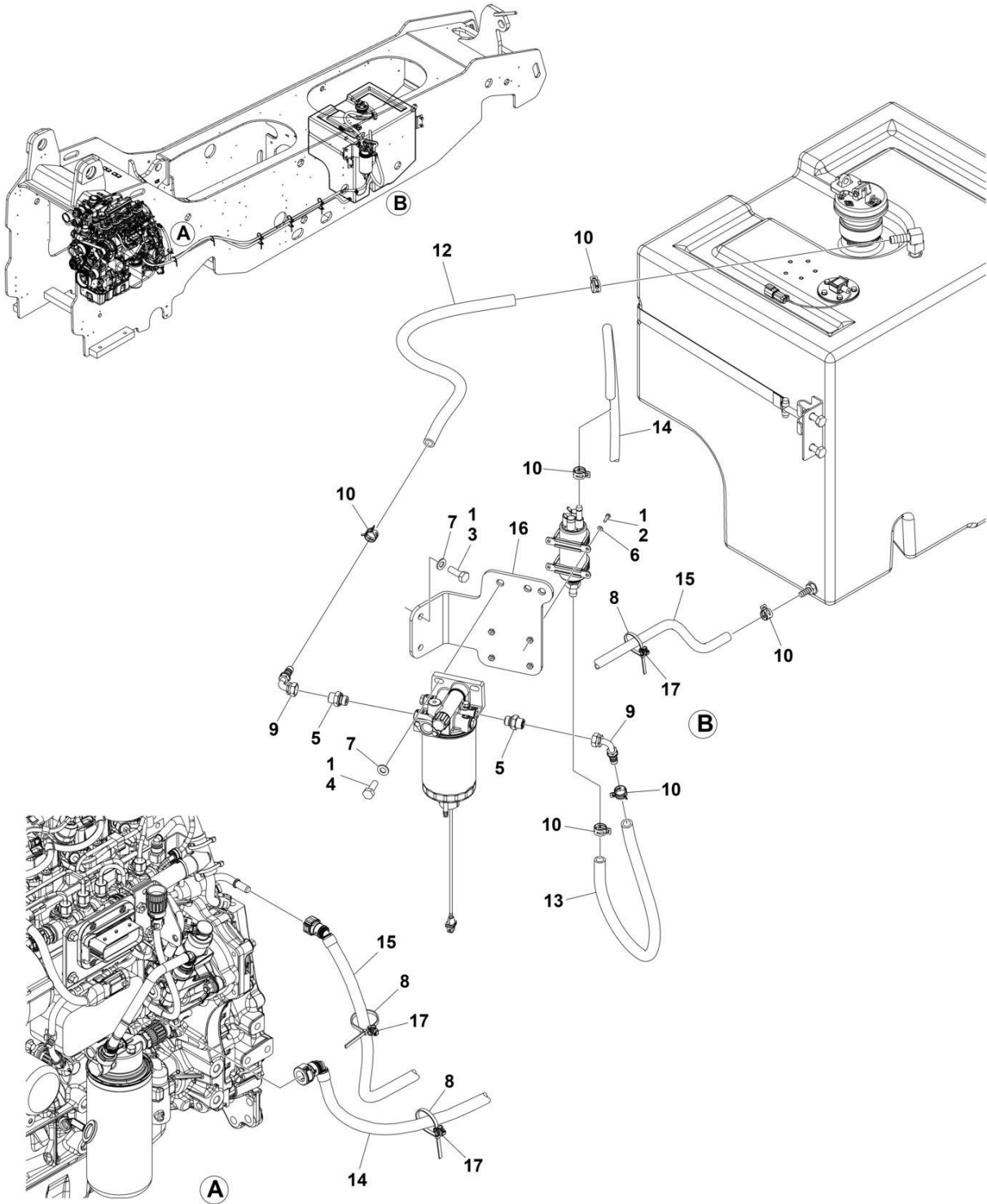
FIGURE 4-10. ENGINE FUEL SYSTEM INSTALLATION (LRC ENGINES)
