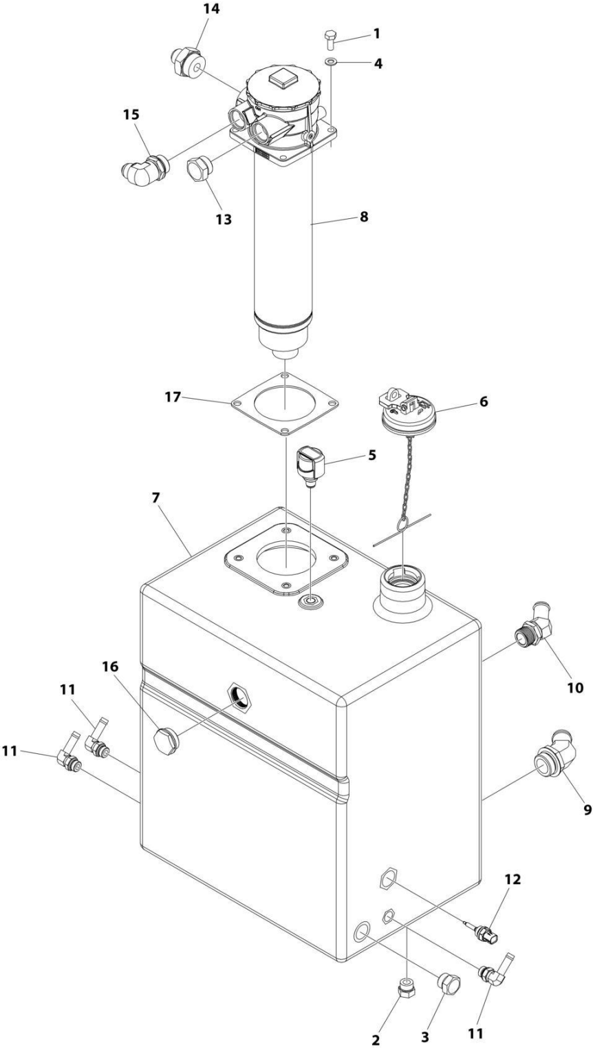
FIGURE 1-6. HYDRAULIC TANK ASSEMBLY (SN 0160147319 to Present)
