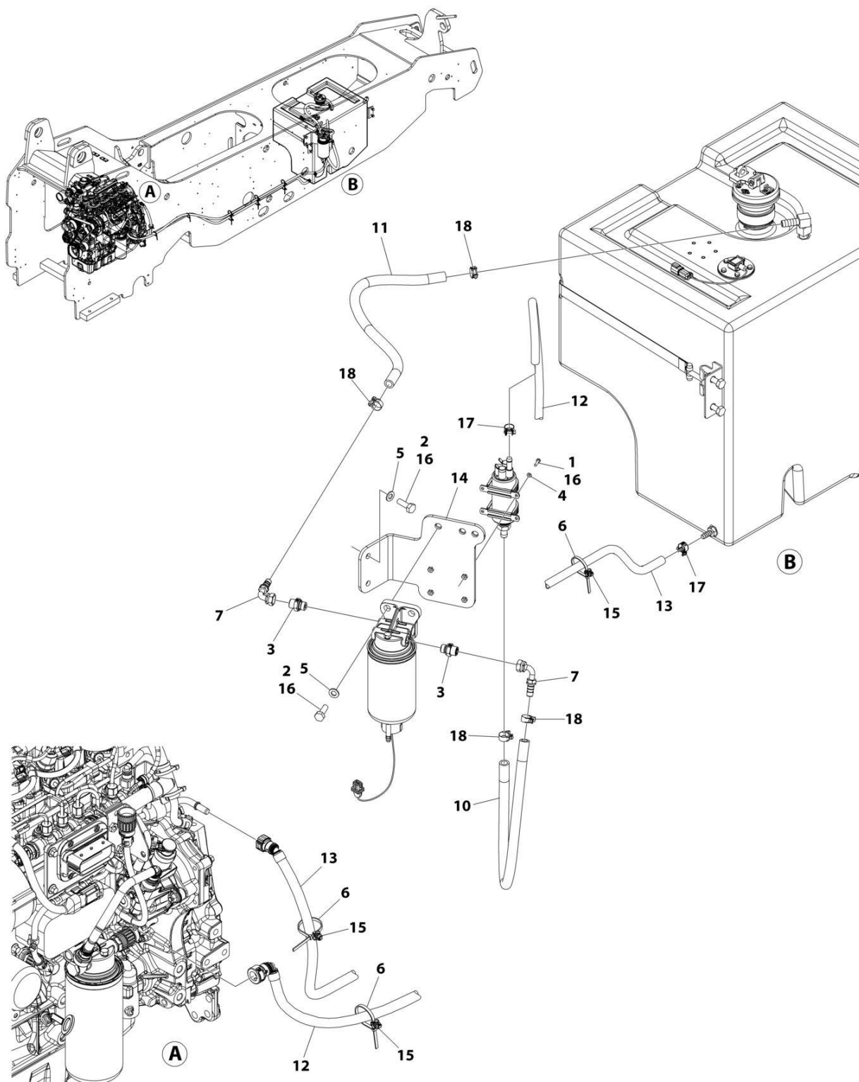
FIGURE 4-9. ENGINE FUEL SYSTEM INSTALLATION (HRC ENGINES) (SN 0160145806 to Present, SN 0160145789 through 0160145795)
