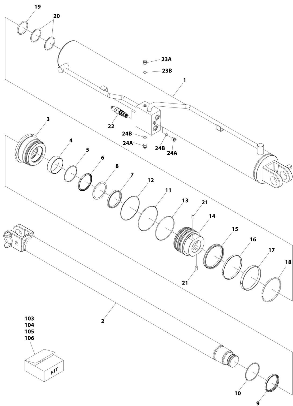
FIGURE 9-7. CYLINDER - LIFT
