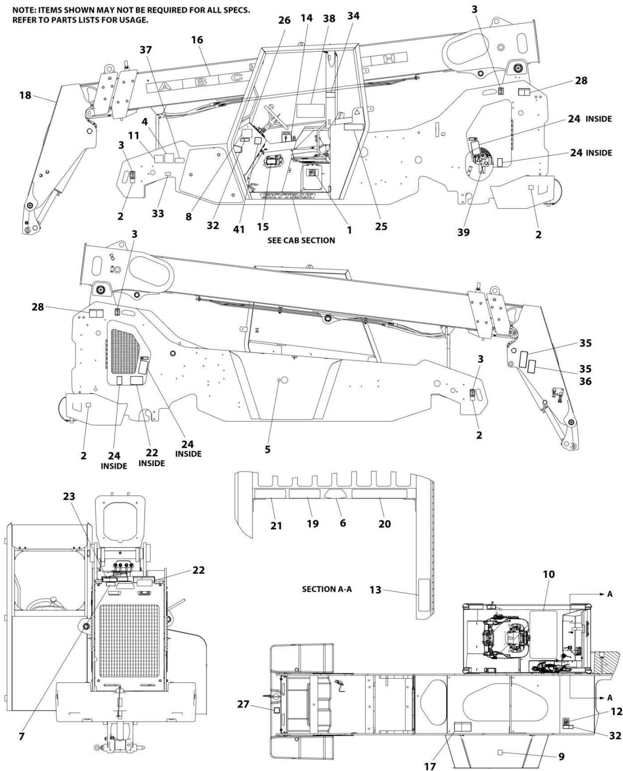
FIGURE 11-1. DECALS INSTALLATION (ANSI SPECS) (Prior to SN 0160151578)
