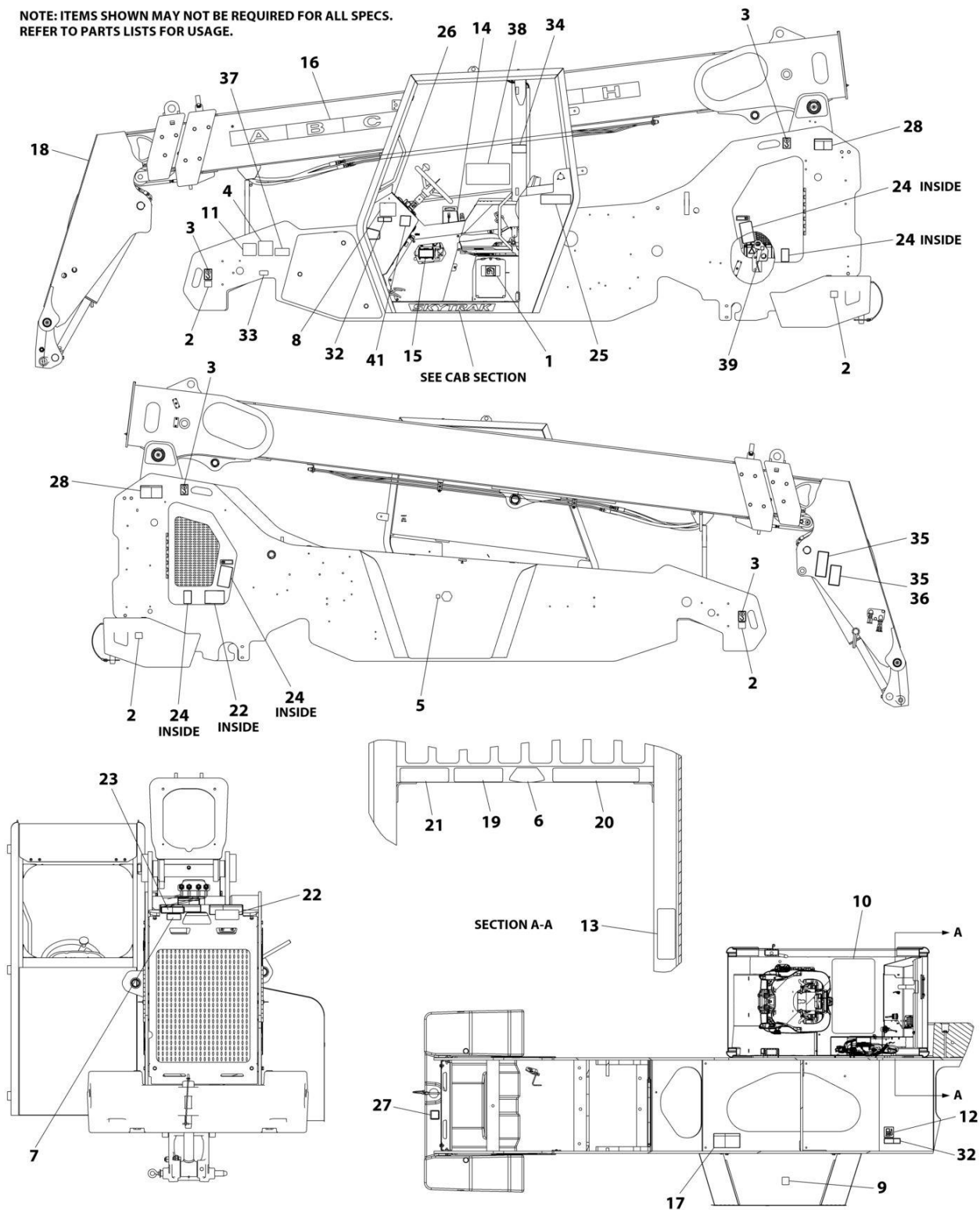
FIGURE 11-3. DECALS INSTALLATION (ISO SPECS) (Prior to SN 0160151578)
