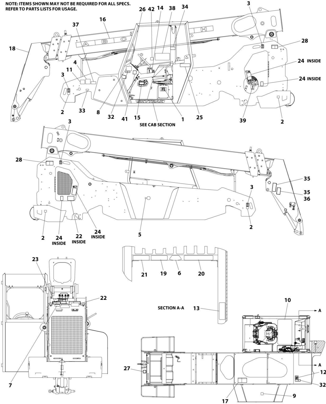
FIGURE 11-2. DECALS INSTALLATION (ANSI SPECS) (SN 0160151579 to Present)
