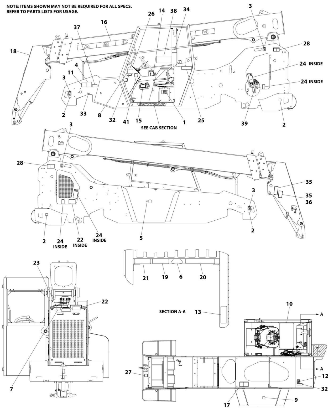
FIGURE 11-5. DECALS INSTALLATION (ENGLISH/FRENCH LANGUAGES) (Prior to SN 0160151578)
