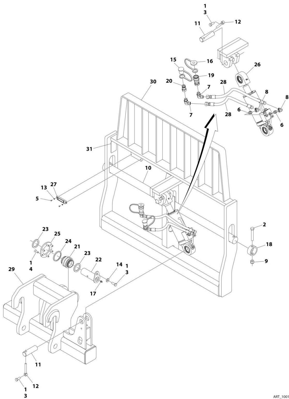
FIGURE 3-22. CARRIAGE ASSEMBLY - 50IN/12000# CAPICITY SIDE TILT (Prior to SN 0160149471)
