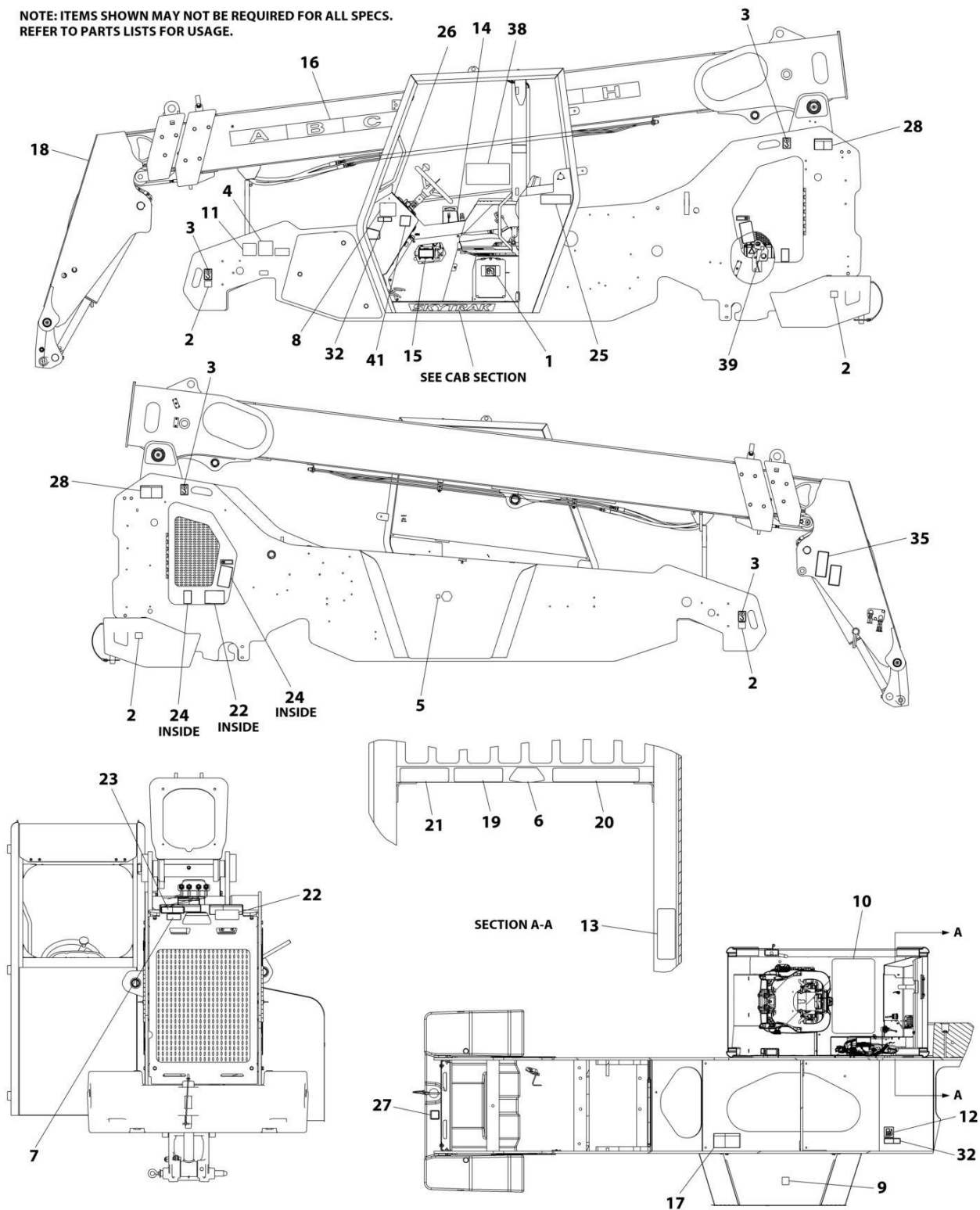
FIGURE 11-9. DECALS INSTALLATIONS (ISO) (HRC) (Prior to SN 0160151578)
