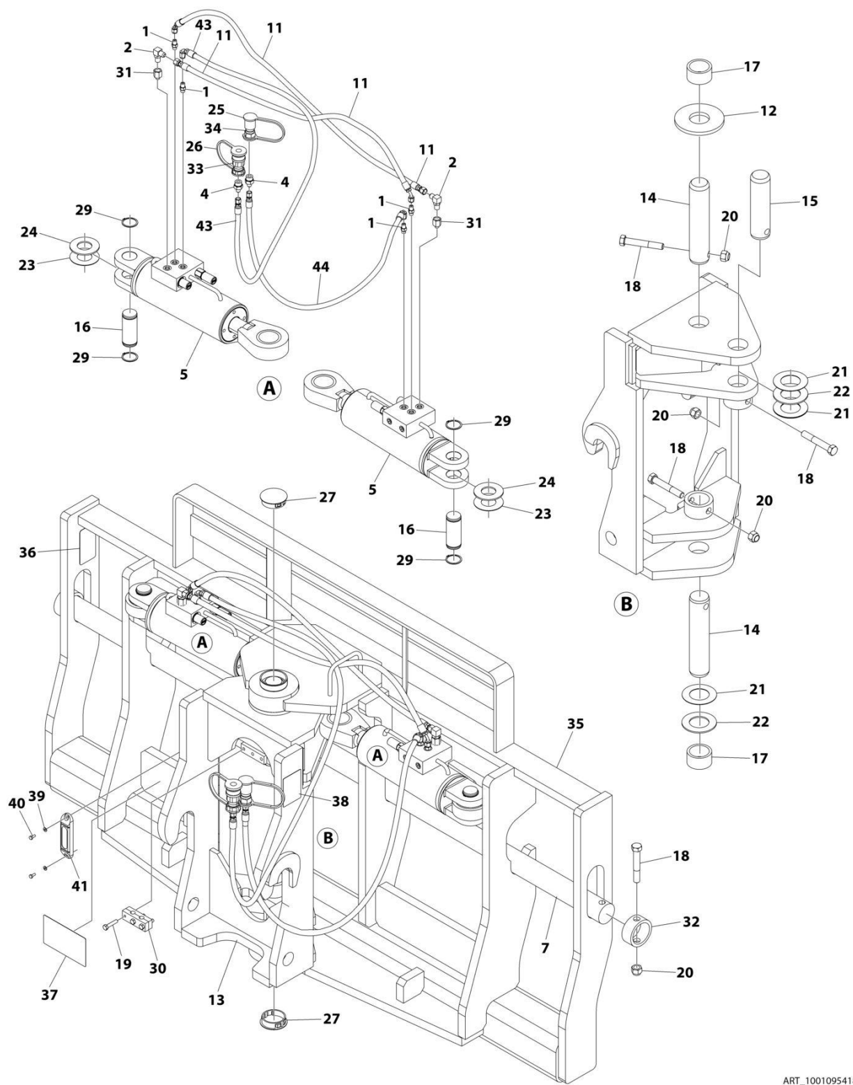
FIGURE 3-32. CARRIAGE ASSEMBLY - 72IN/10000# CAPACITY 90 DEGREE SWING (Prior to SN 0160149471)
