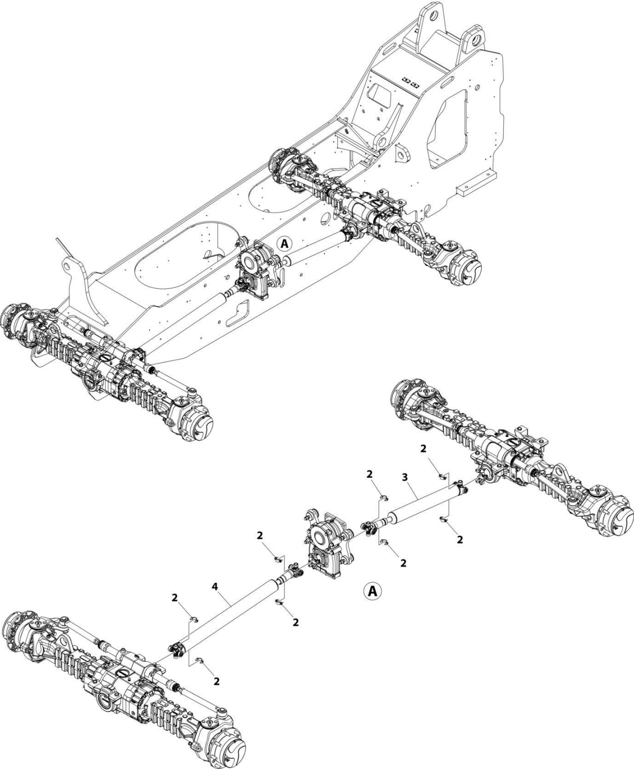
FIGURE 5-17. DRIVESHAFT INSTALLATION (SN 0160141868 to Present, SN 0160141853 through 0160141860, SN 0160141862 through 0160141864)
