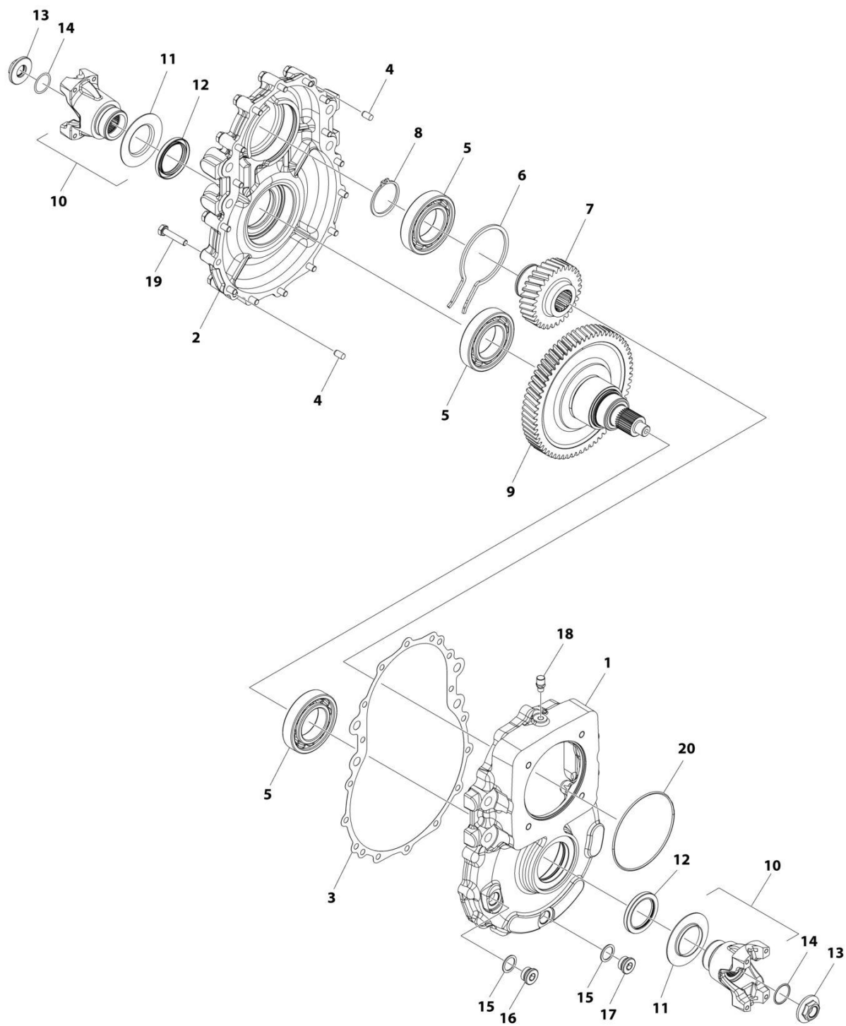
FIGURE 5-22. GEARBOX ASSEMBLY
