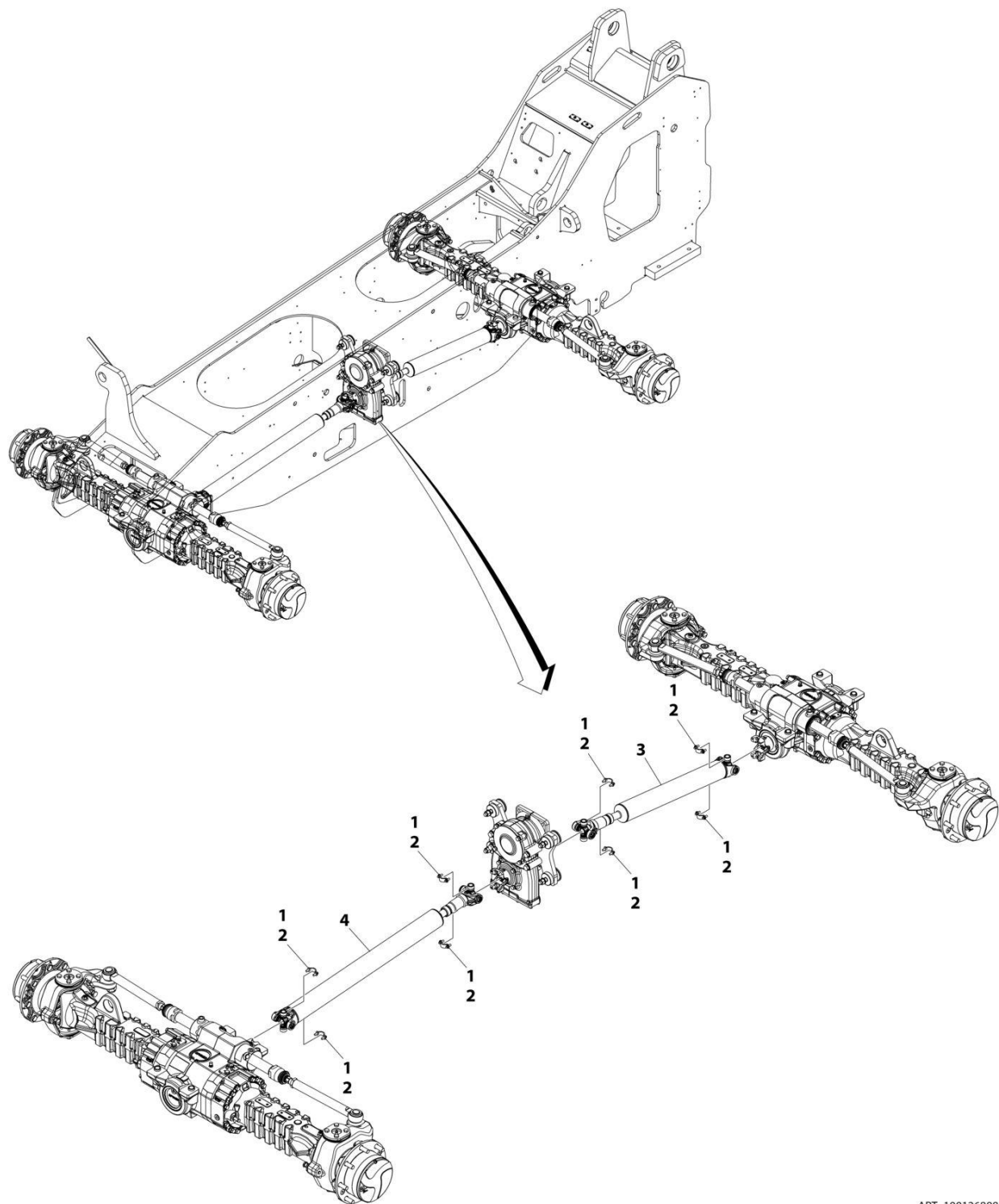
FIGURE 5-16. DRIVESHAFT INSTALLATION (Prior to SN 0160141867)
