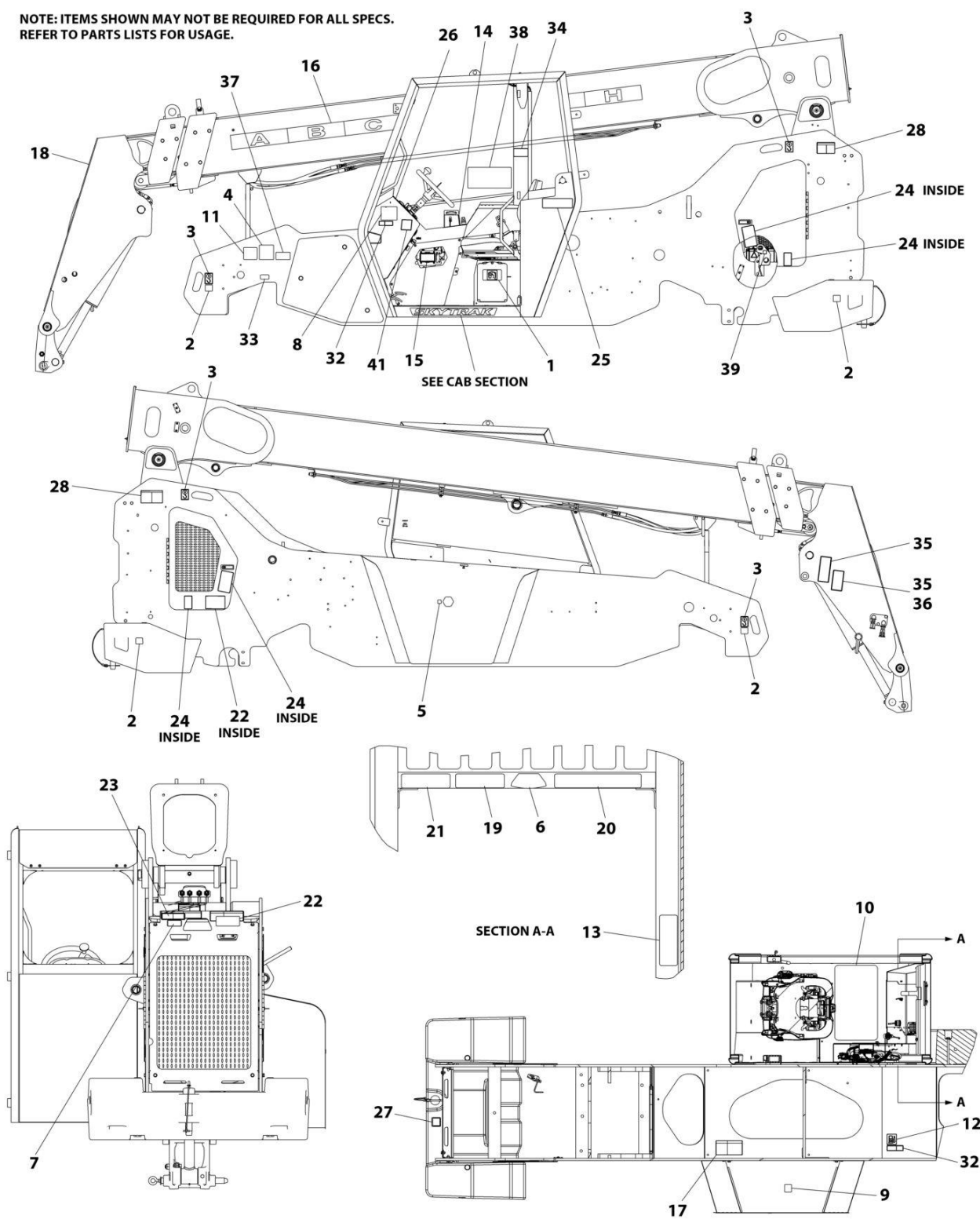
FIGURE 11-7. DECALS INSTALLATION (ENGLISH/SPANISH LANGUAGES) (Prior to SN 0160151578)
