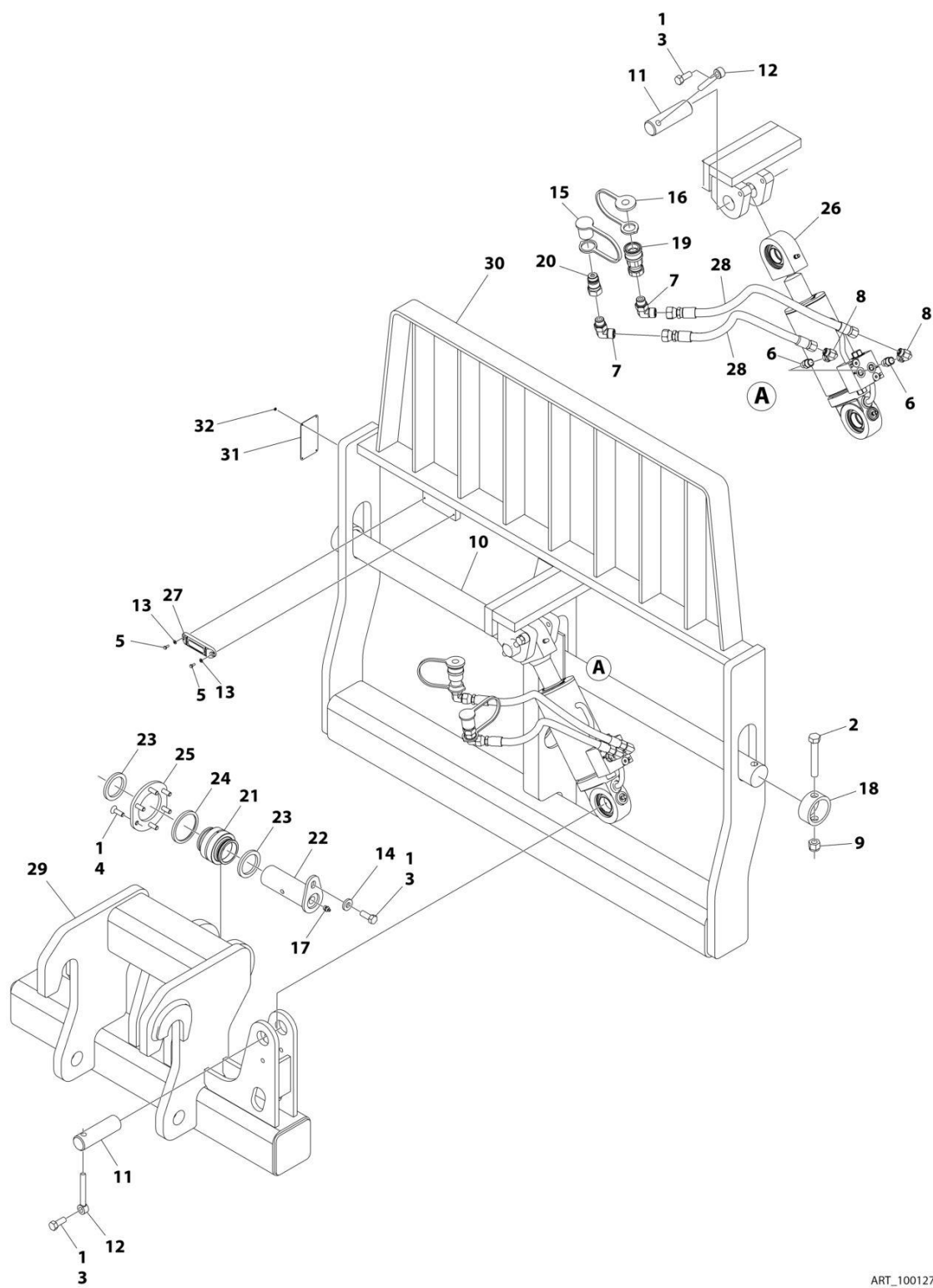
FIGURE 3-23. CARRIAGE ASSEMBLY - 50IN/12000# CAPICITY SIDE TILT (SN 0160149472 to Present)
