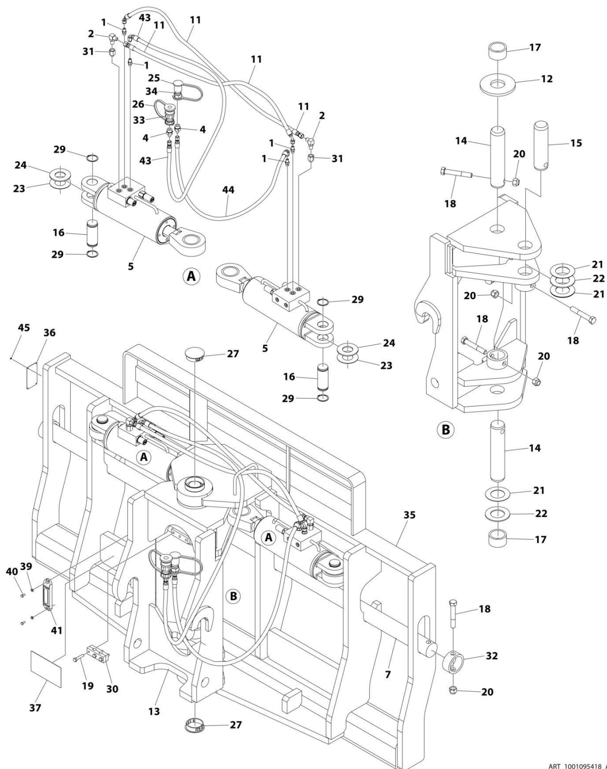
FIGURE 3-33. CARRIAGE ASSEMBLY - 72IN/10000# CAPACITY 90 DEGREE SWING (SN 0160149469 to Present)
