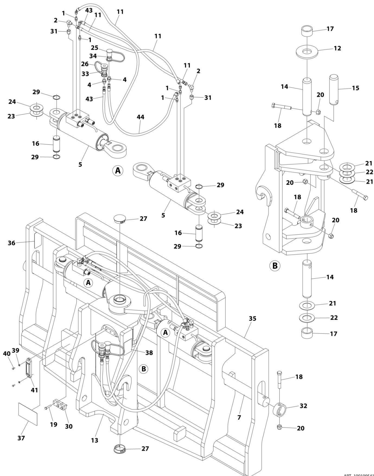
FIGURE 3-32. CARRIAGE ASSEMBLY - 72IN/10000# CAPACITY 90 DEGREE SWING (Prior to SN 0160149468)
