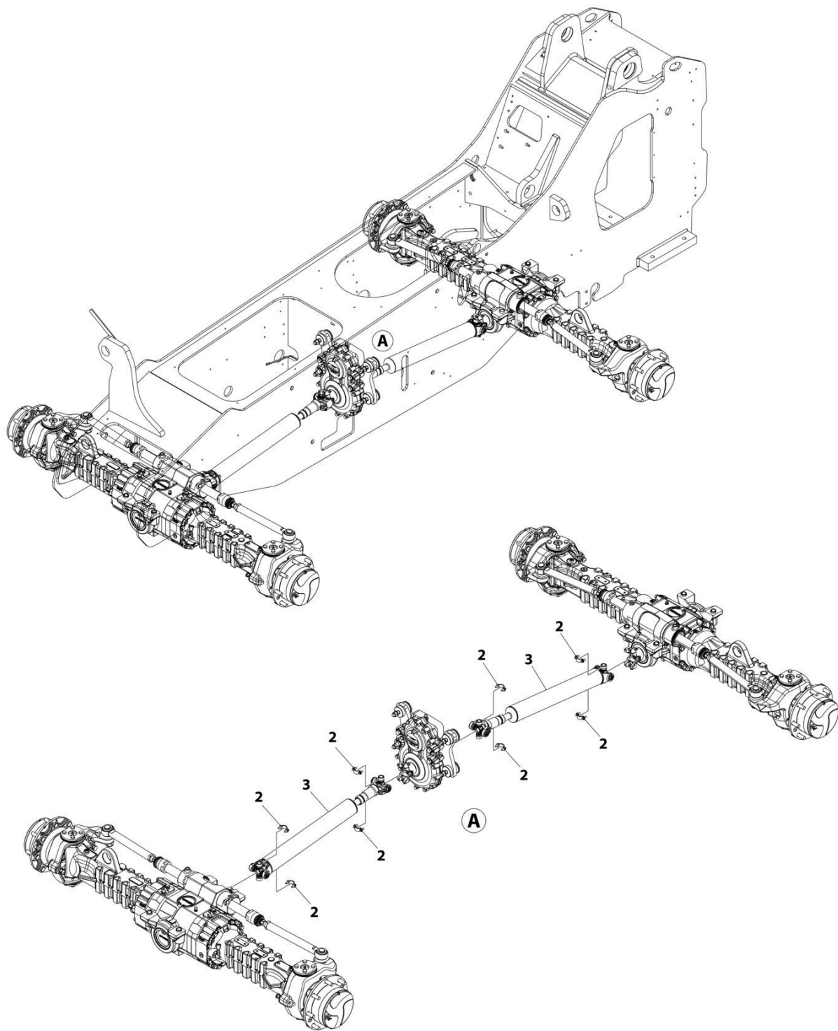
FIGURE 5-19. DRIVESHAFT INSTALLATION (SN 0160141848 to Present, SN 0160141839 through 0160141841, SN 0160141843 through 0160141846)
