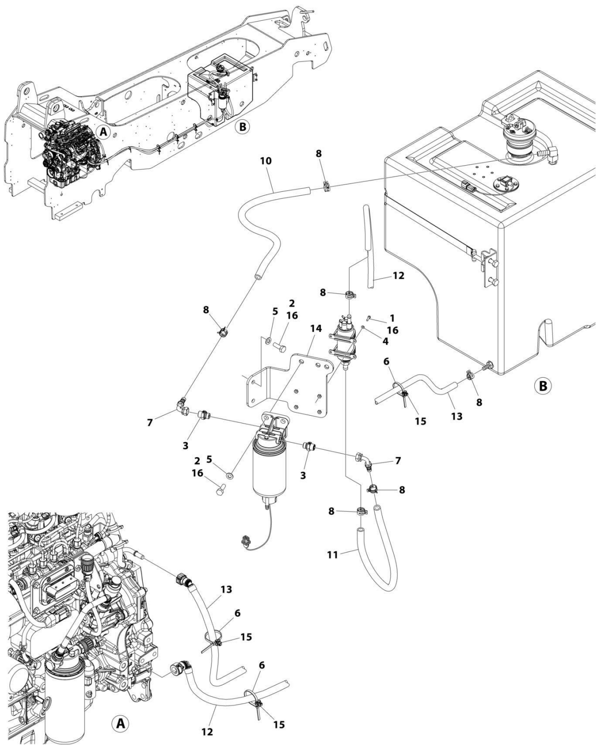
FIGURE 4-8. ENGINE FUEL SYSTEM INSTALLATION (HRC ENGINES) (Prior to SN 0160145805)
