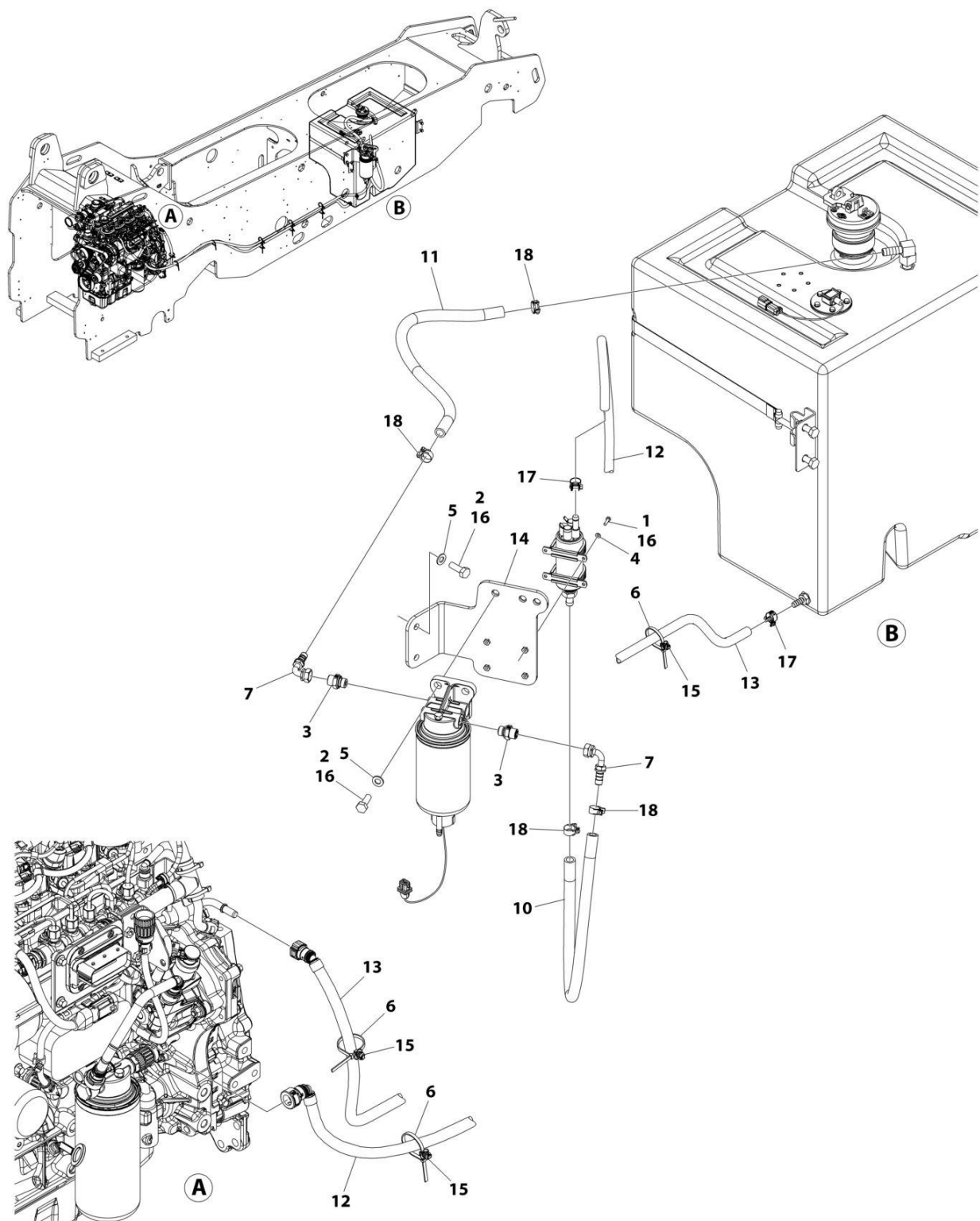
FIGURE 4-9. ENGINE FUEL SYSTEM INSTALLATION (HRC ENGINES) (SN 0160145806 to Present, SN 0160145789 through 0160145795)
