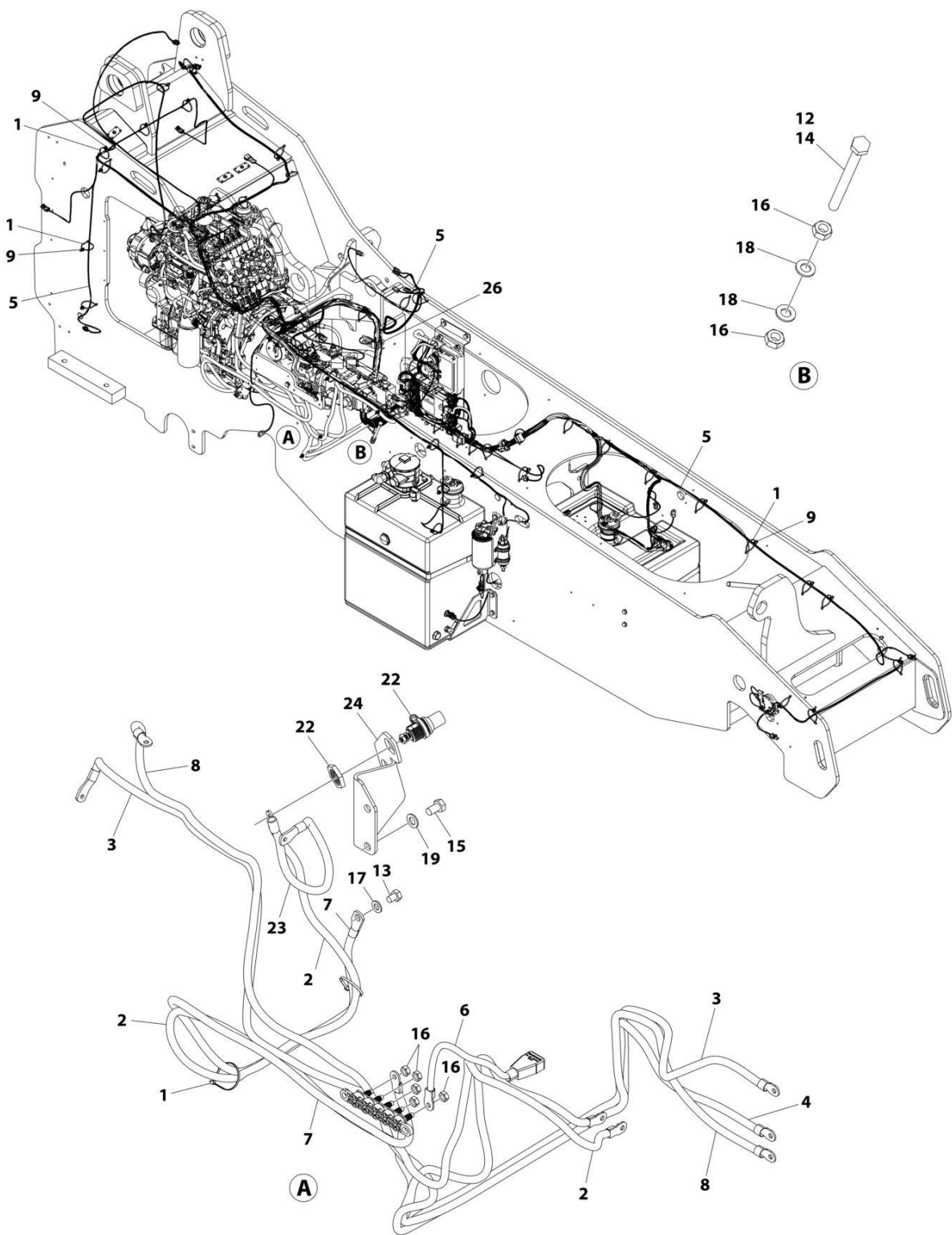
FIGURE 10-22. FRAME HARNESS INSTALLATION
