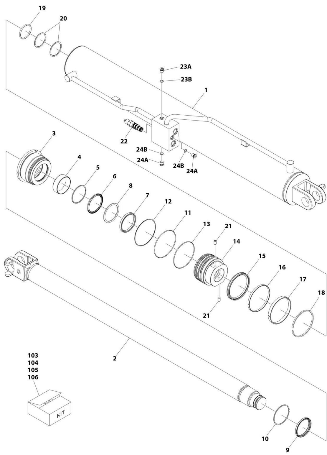
FIGURE 9-7. CYLINDER - LIFT
