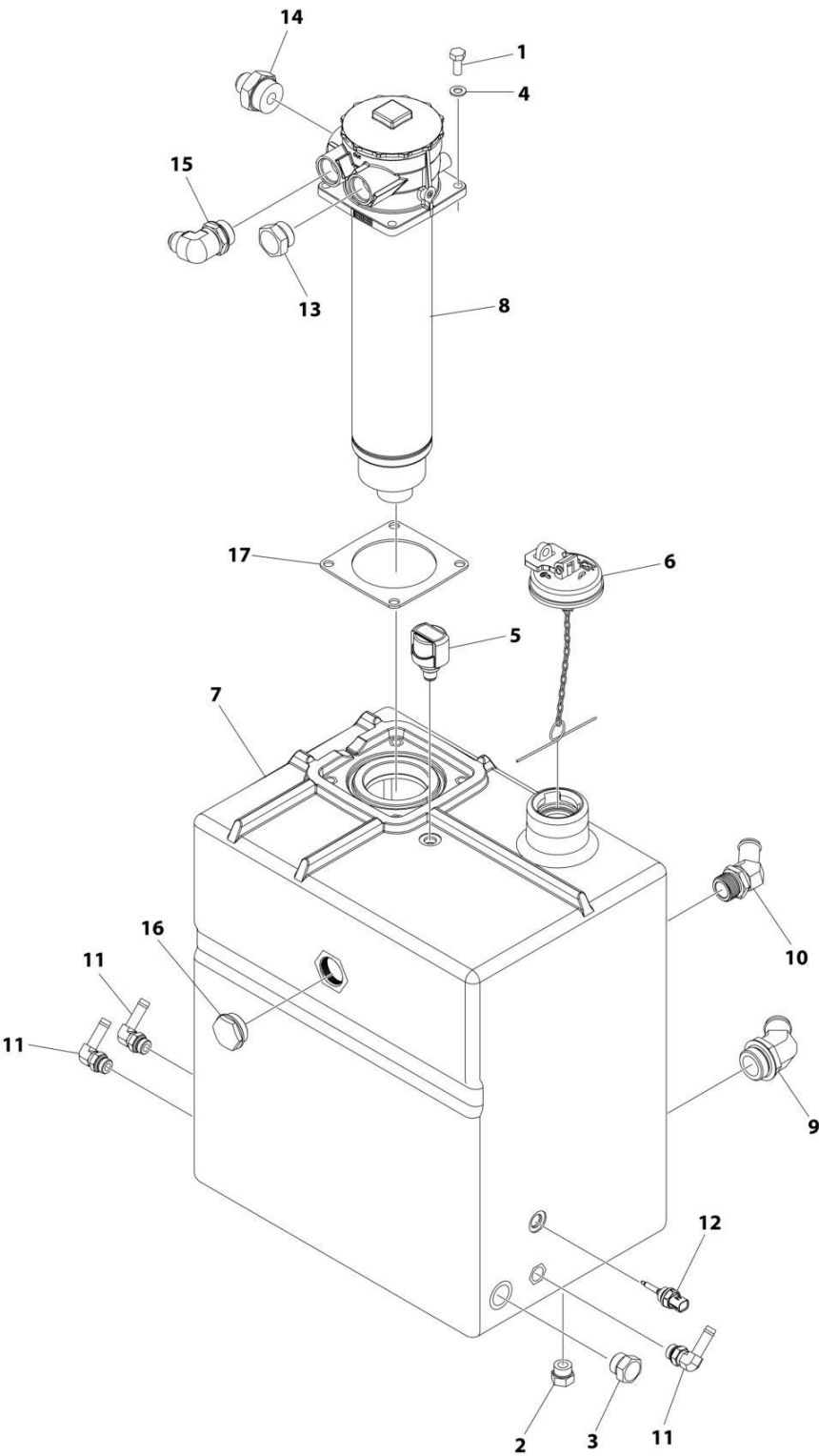
FIGURE 1-5. HYDRAULIC TANK ASSEMBLY (Prior to SN 0160147335)
