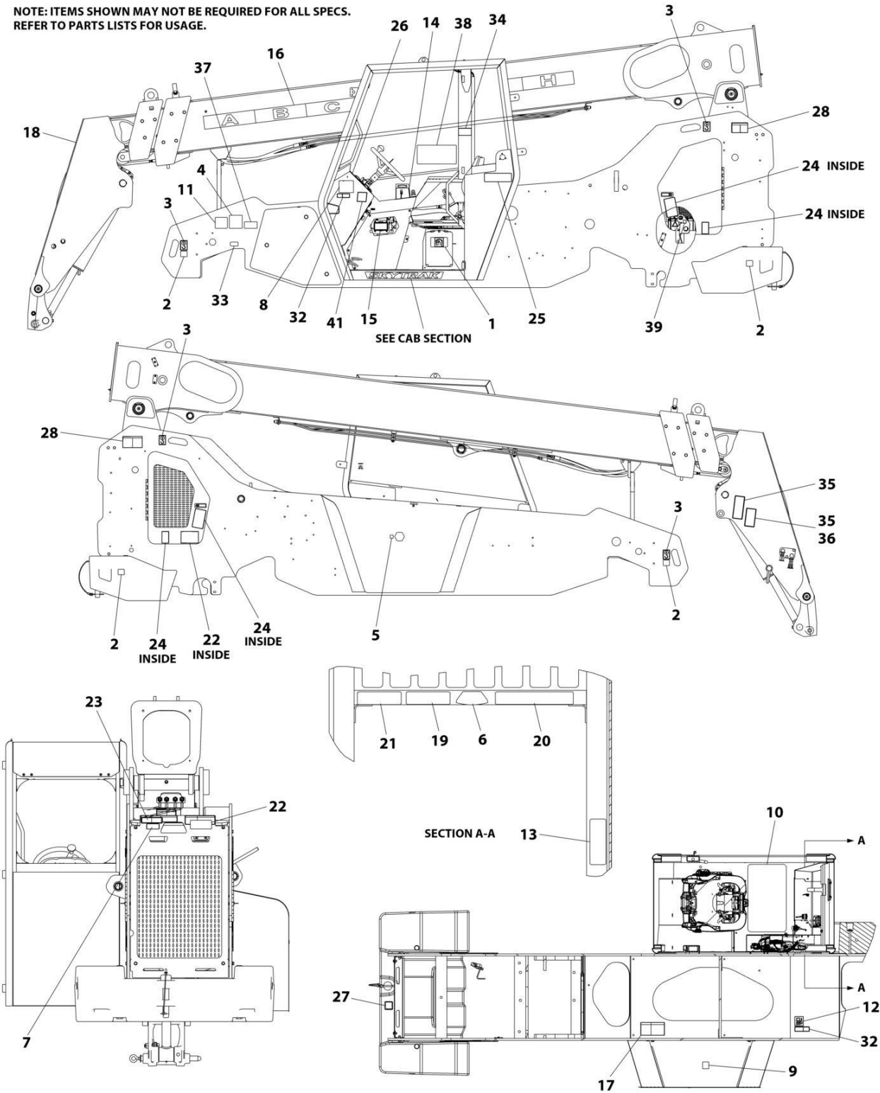
FIGURE 11-2. DECALS INSTALLATION (ISO SPECS)
