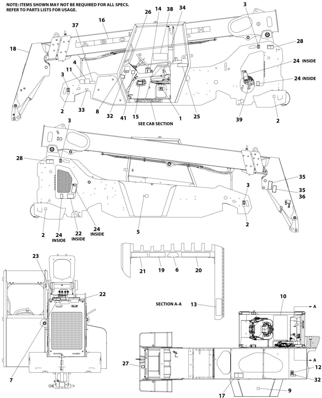
FIGURE 11-3. DECALS INSTALLATION (ENGLISH/FRENCH LANGUAGES)
