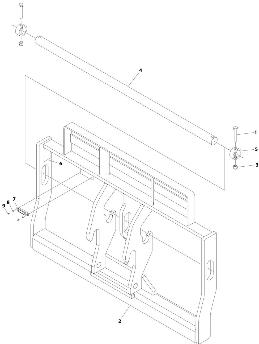
FIGURE 3-19. CARRIAGE ASSEMBLY - 60IN
