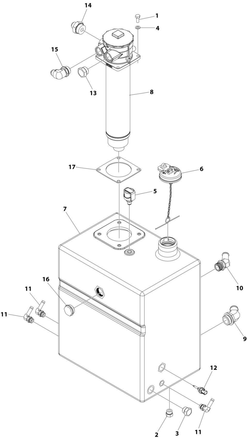
FIGURE 1-6. HYDRAULIC TANK ASSEMBLY (SN 0160147334 to Present)
