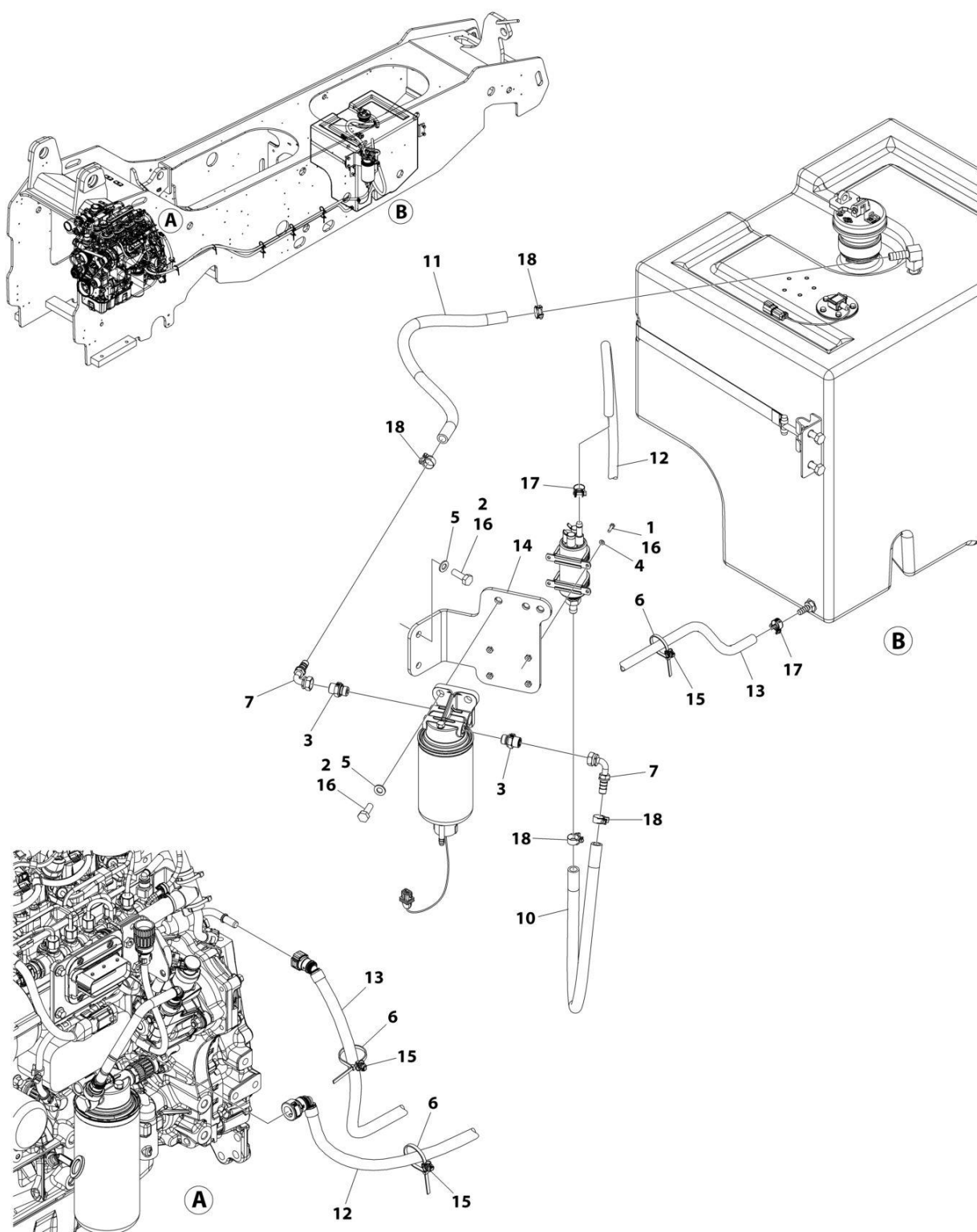
FIGURE 4-9. ENGINE FUEL SYSTEM INSTALLATION (HRC ENGINES) (SN 0160145788 to Present)
