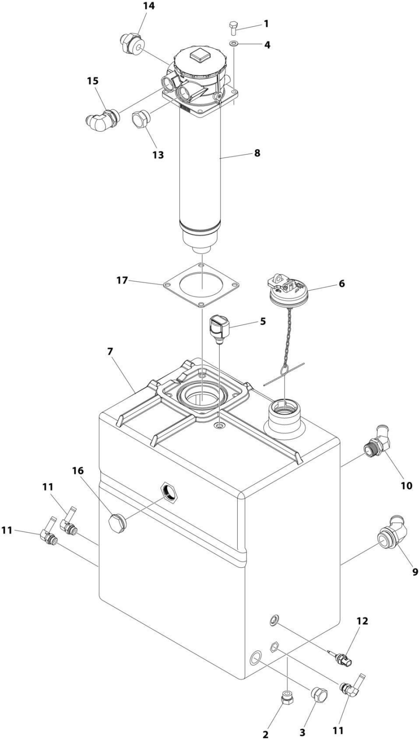
FIGURE 1-5. HYDRAULIC TANK ASSEMBLY (Prior to SN 0160147333)
