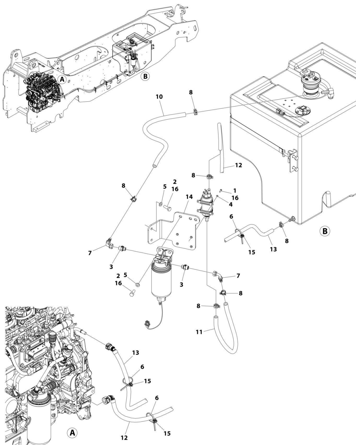
FIGURE 4-8. ENGINE FUEL SYSTEM INSTALLATION (HRC ENGINES) (Prior to SN 0160145787)
