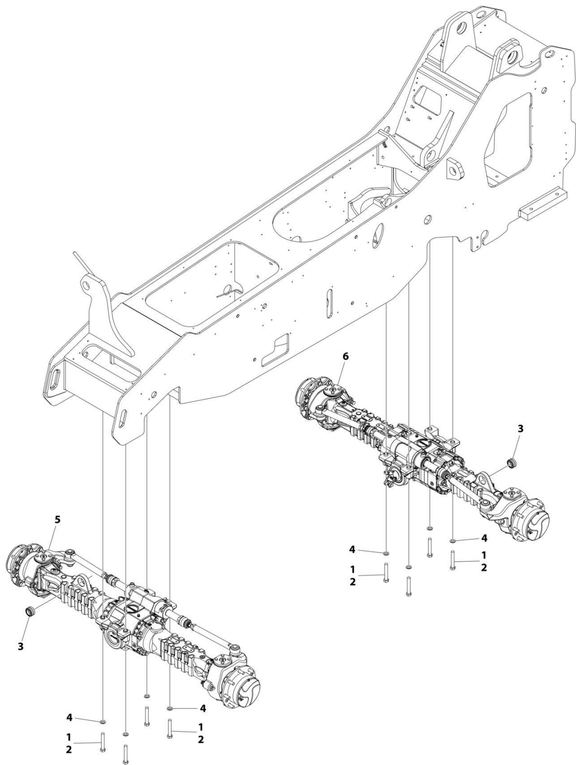
FIGURE 5-1. AXLES INSTALLATION
