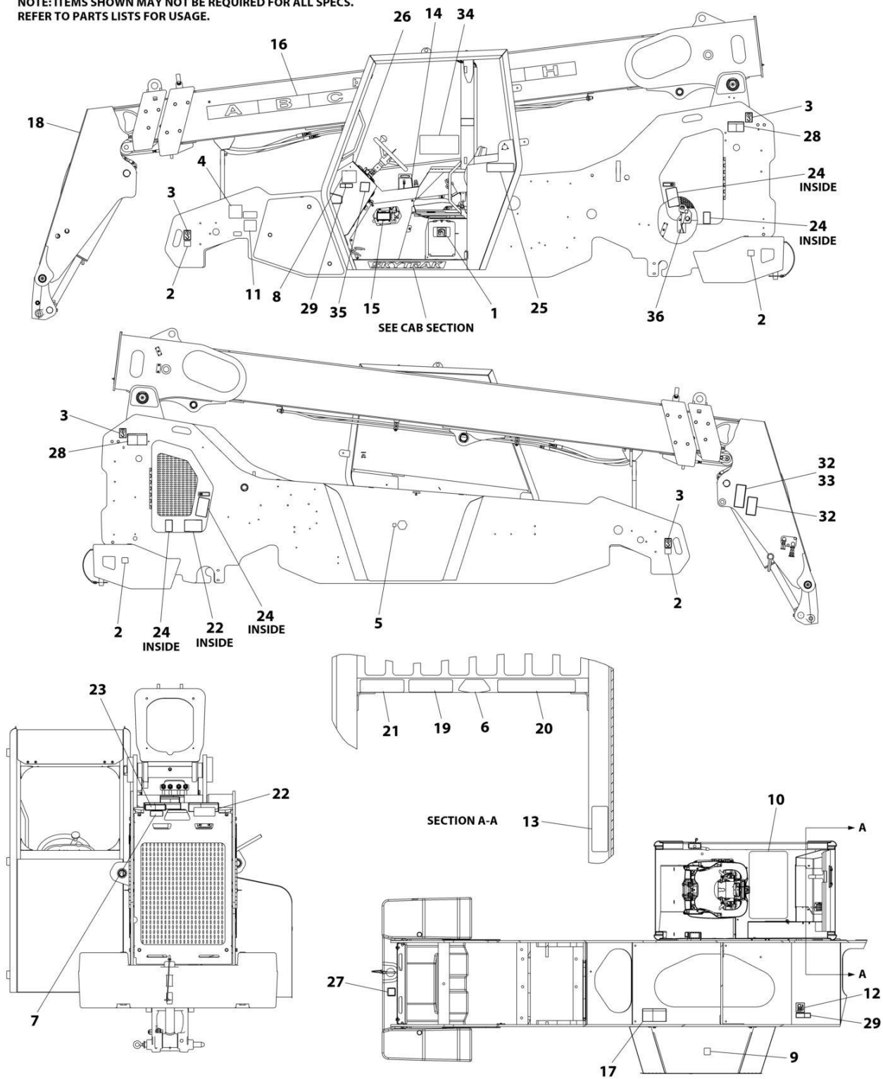
FIGURE 11-5. DECALS INSTALLATIONS (ISO) (HRC)
