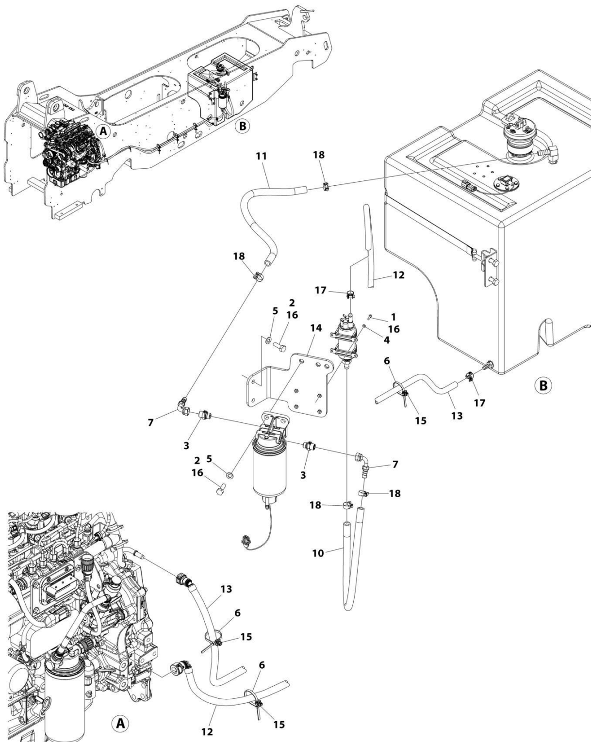
FIGURE 4-9. ENGINE FUEL SYSTEM INSTALLATION (HRC ENGINES) (SN 0160145924 to Present, SN 0160145554 through 0160145555, SN 0160145713 through 0160145715, SN 0160145718 through 0160145721, SN 0160145723 through 0160145724, SN 0160145731 through 0160145735, SN 0160145739 through 0160145747, SN 0160145749 through 0160145753, SN 0160145759 through 0160145760, SN 0160145768 through 0160145772, SN 0160145777 through 0160145778)
