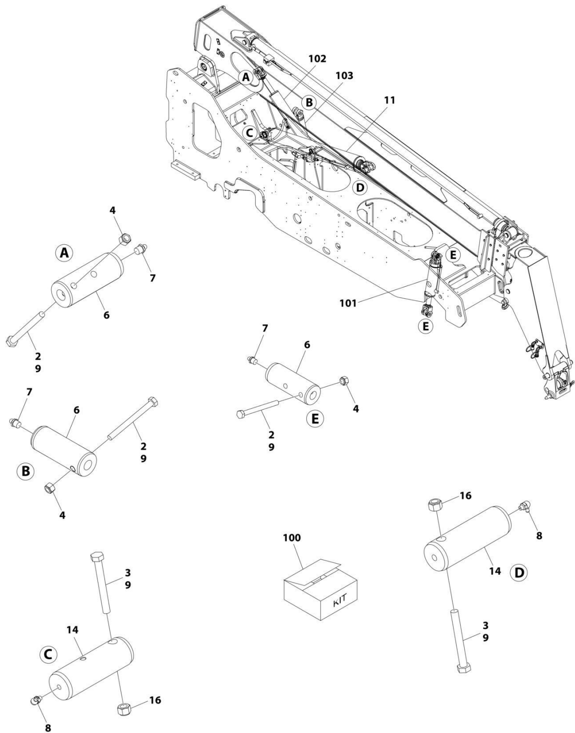
FIGURE 9-6. CYLINDER INSTALLATION
