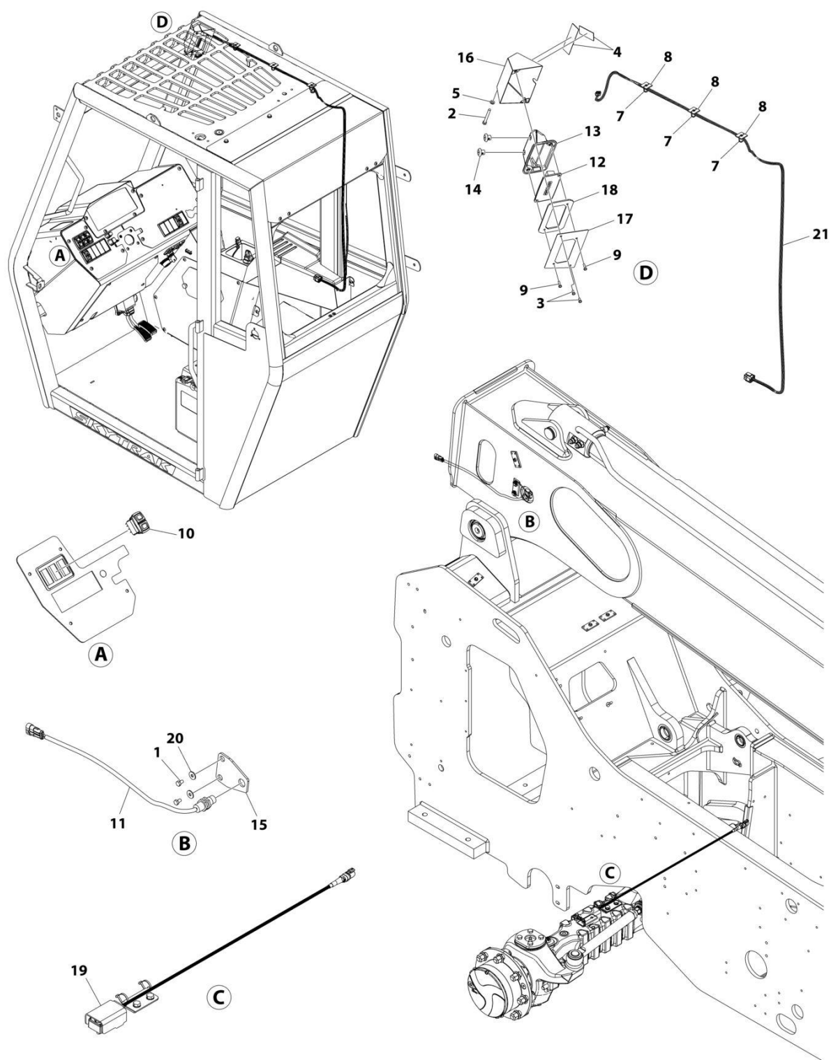
FIGURE 10-34. LOAD SENSE INDICATOR (LSI) SYSTEM INSTALLATION - CAB
