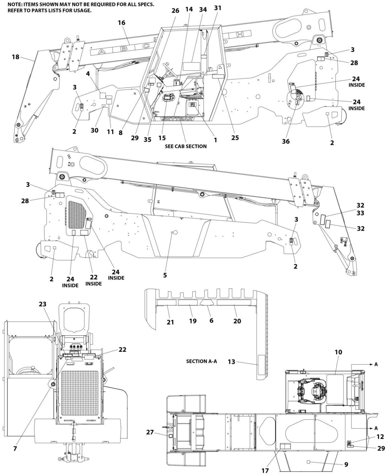
FIGURE 11-1. DECALS INSTALLATION (ANSI SPECS)
