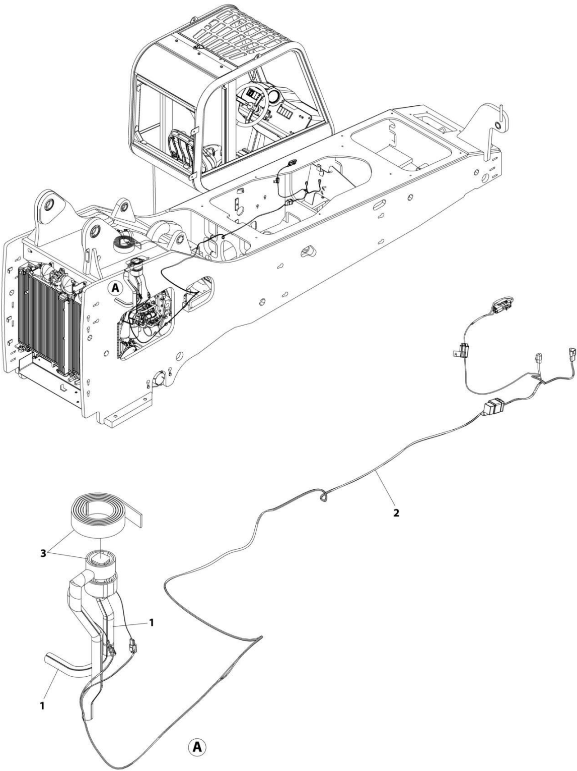
FIGURE 4-38. HEATER BREATHER (SN 0160144023 to Present)
