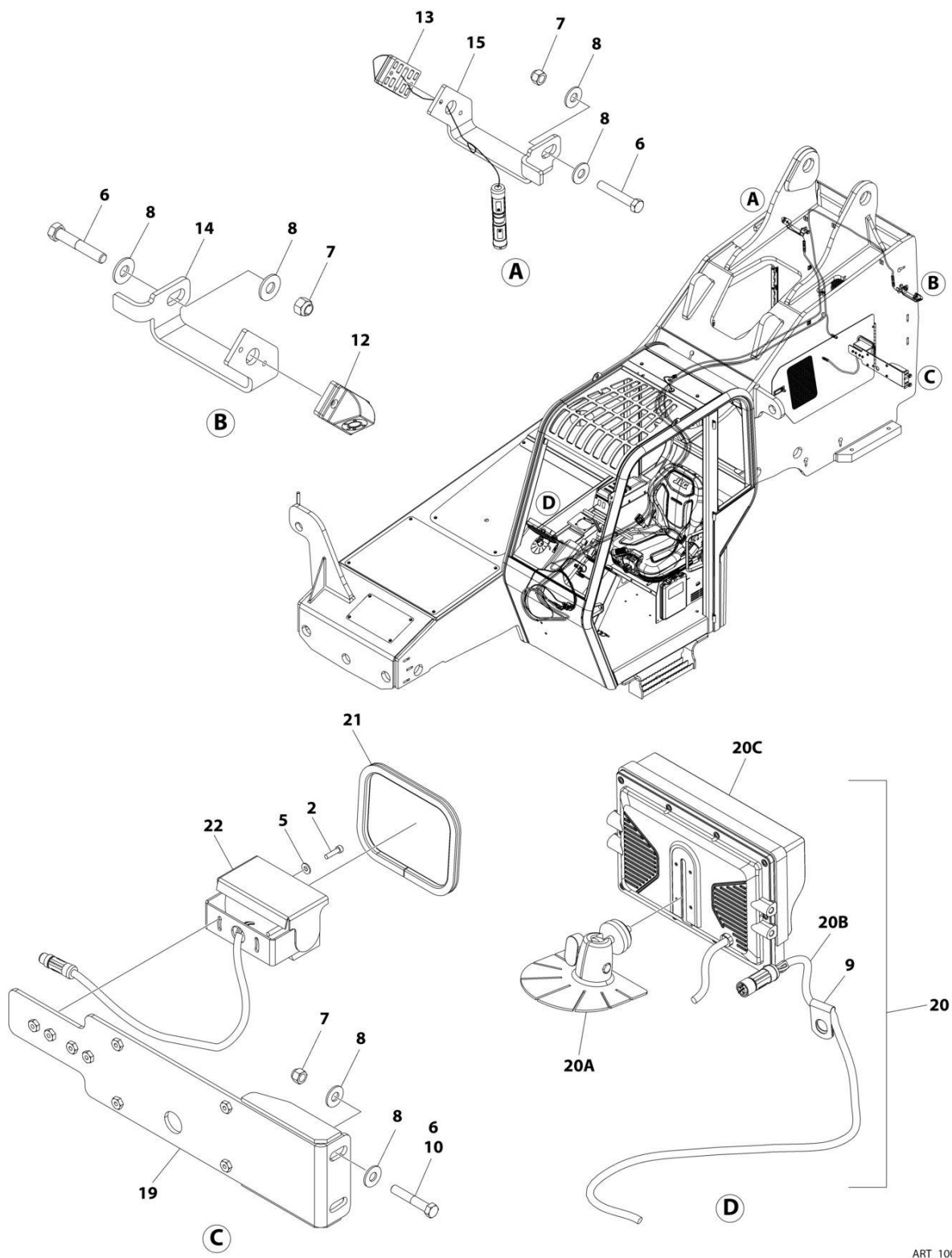
FIGURE 10-42. MULTI VIEW CAMERA INSTALLATION
