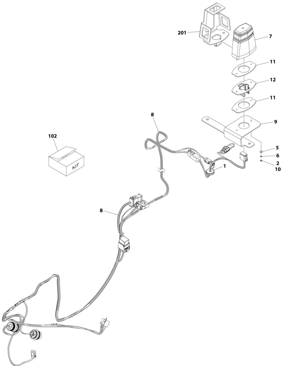
FIGURE 10-14. CLEARSKY CS550 BEACON INSTALLATION (CLOSED CAB)
