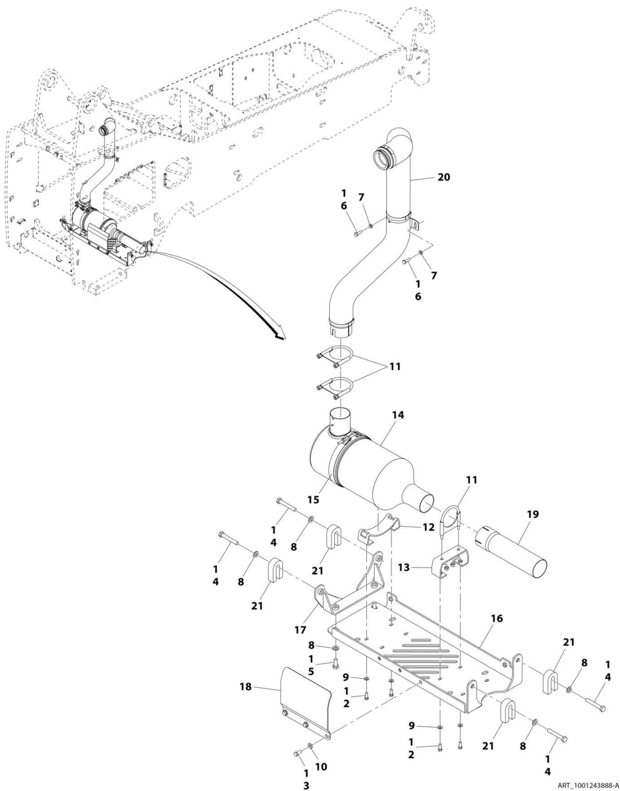
FIGURE 4-27. EXHAUST INSTALLATION (74HP)
