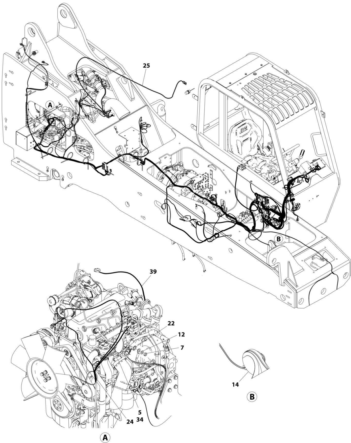
FIGURE 10-1. ELECTRICAL INSTALLATION (74HP) (LS)
