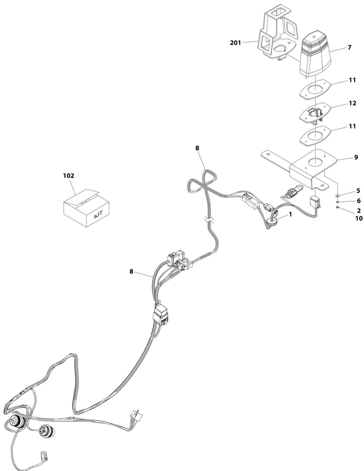
FIGURE 10-19. CLEARSKY CS550 BEACON INSTALLATION (CLOSED CAB)
