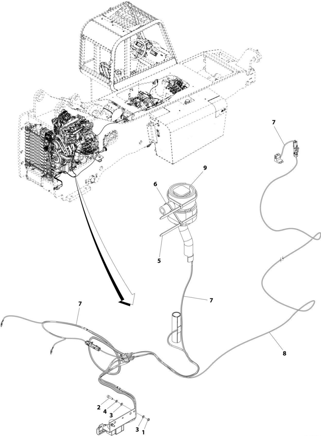
FIGURE 4-33. BREATHER HEATER INSTALLATION - 74HP
