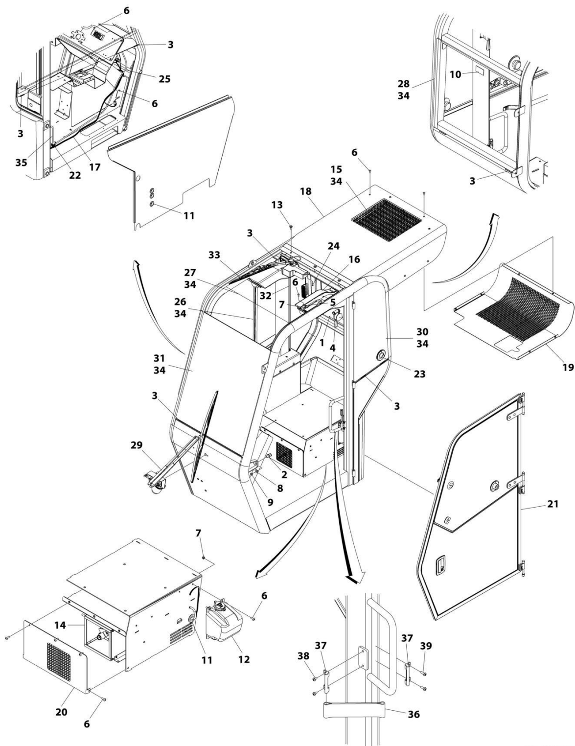
FIGURE 6-15. CAB ENCLOSURE WITH HEATER & AC
