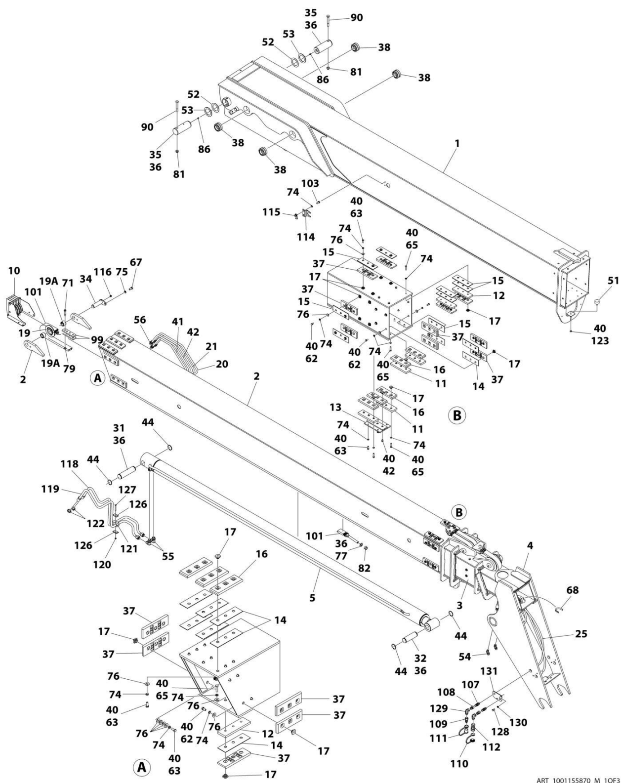
FIGURE 2-1. BOOM INSTALLATION
