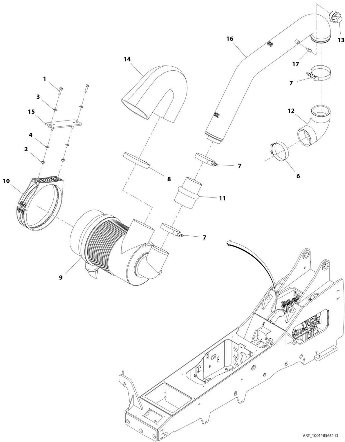
FIGURE 4-9. AIR CLEANER INSTALLATION - 110HP (LS)
