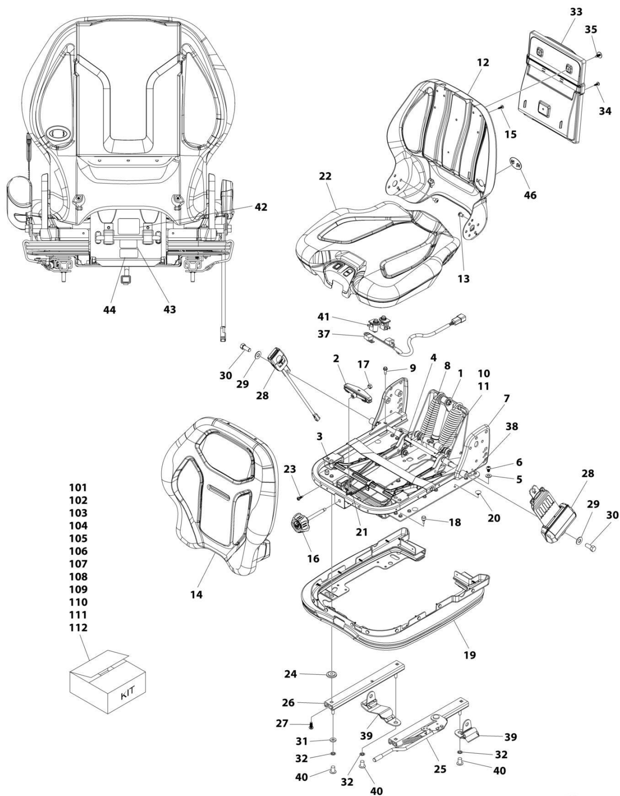
FIGURE 6-21. SEAT ASSEMBLY - VINYL
