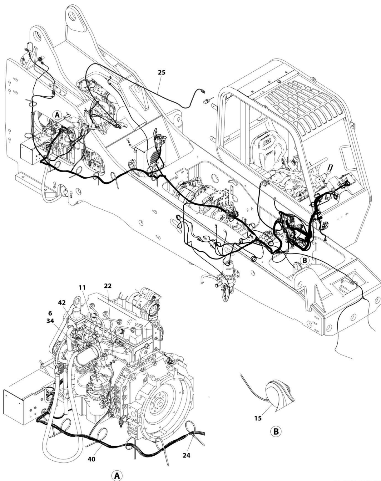
FIGURE 10-3. ELECTRICAL INSTALLATION (110HP) (LS)
