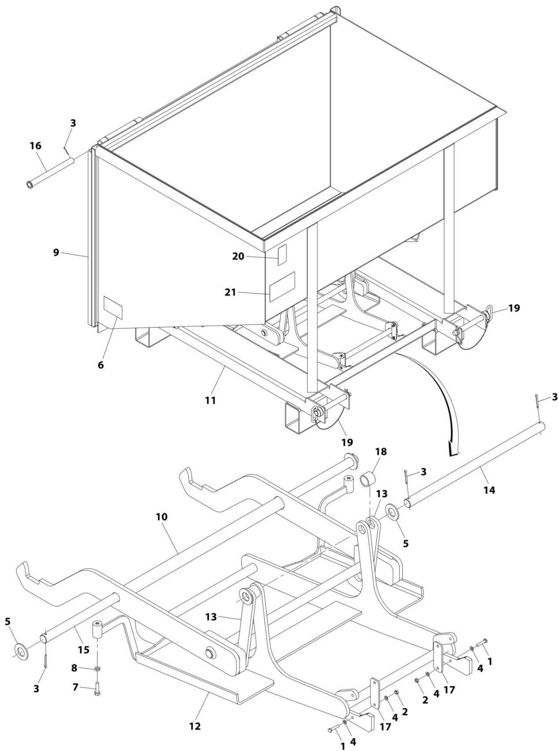
FIGURE 3-55. TRASHER HOPPER
