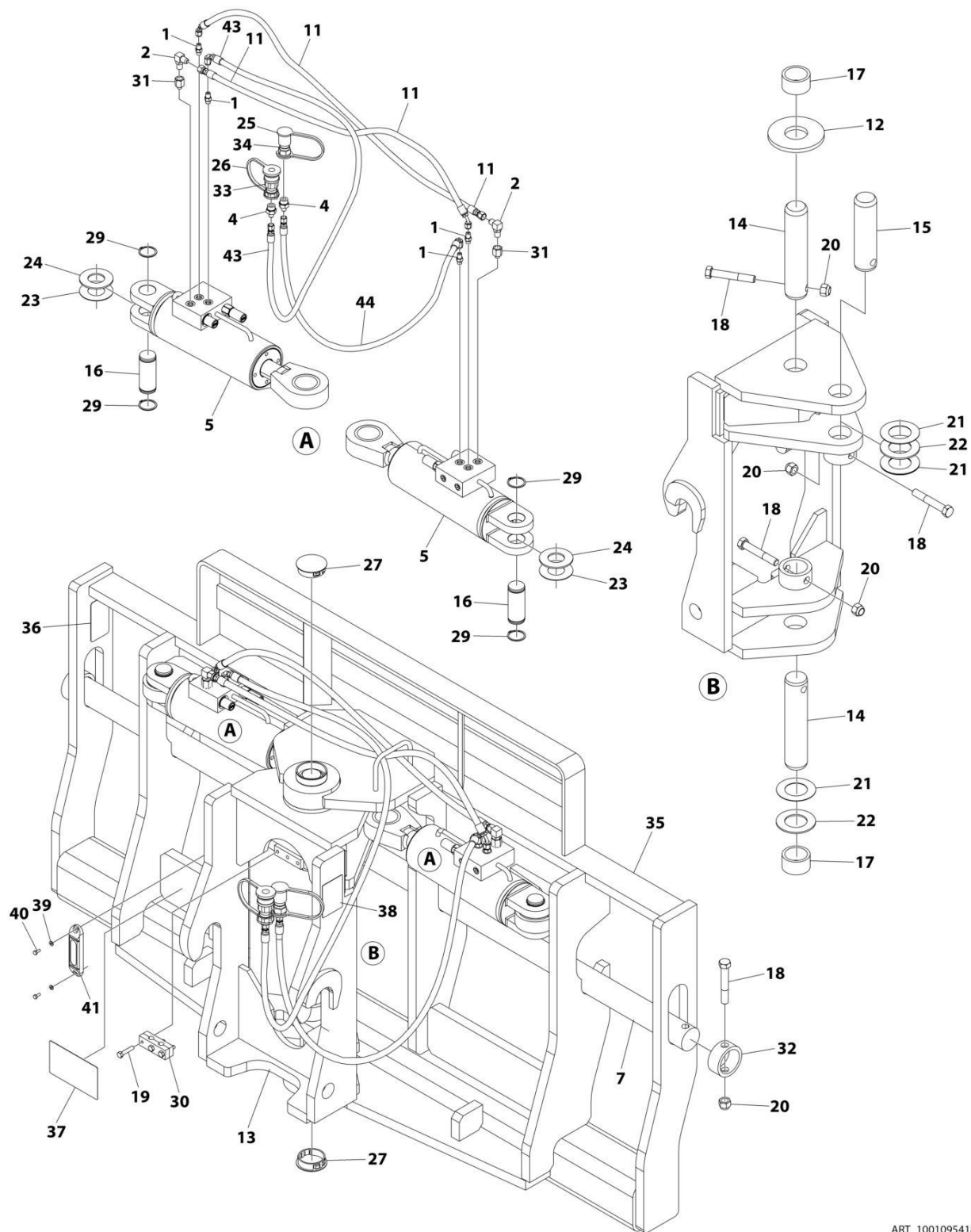
FIGURE 3-24. CARRIAGE ASSEMBLY - 72IN/10000# CAPACITY 90 DEGREE SWING
