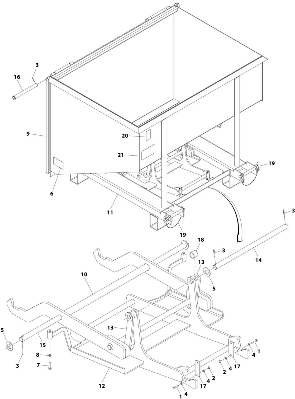
FIGURE 3-1. TRASHER HOPPER
