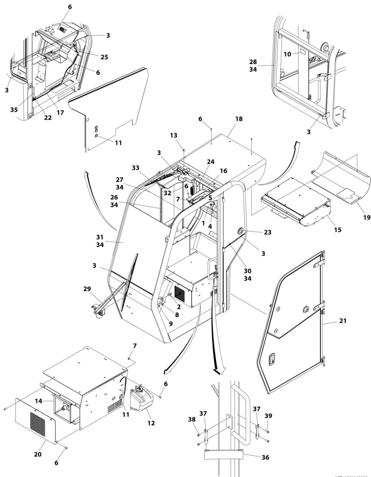
FIGURE 6-9. CAB ENCLOSURE WITH HEATER
