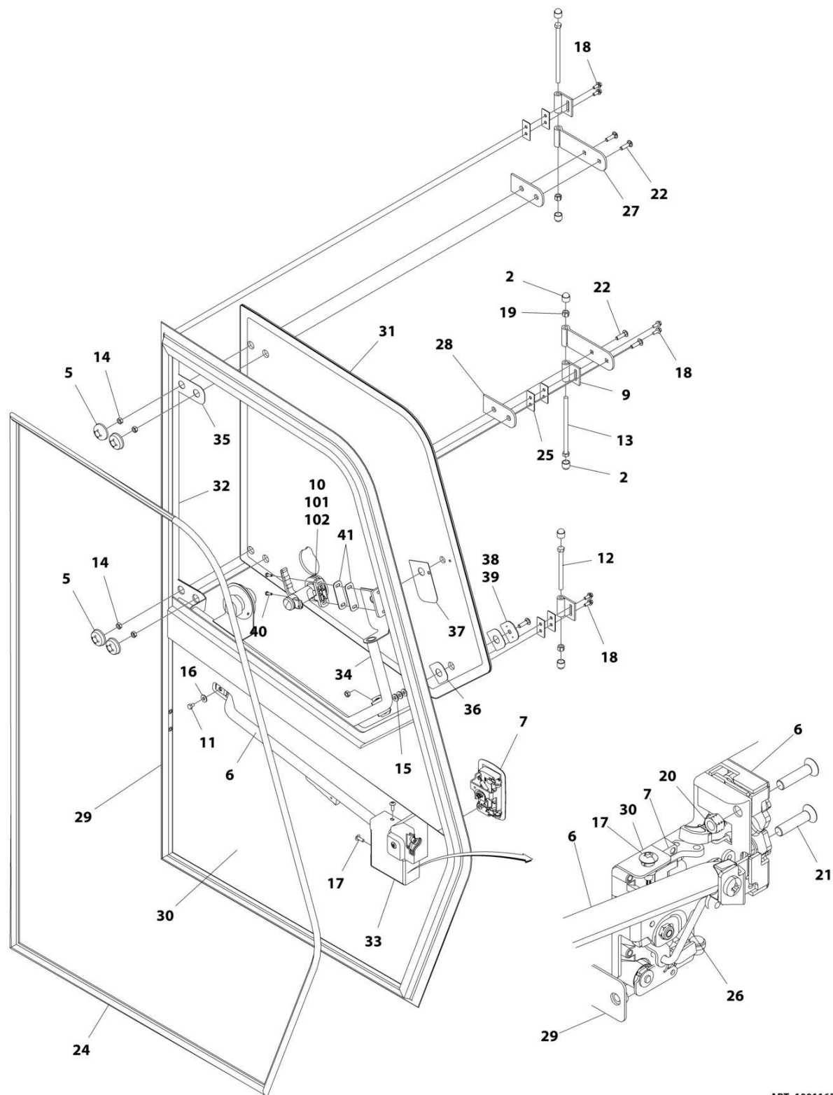
FIGURE 6-15. CAB DOOR ASSEMBLY
