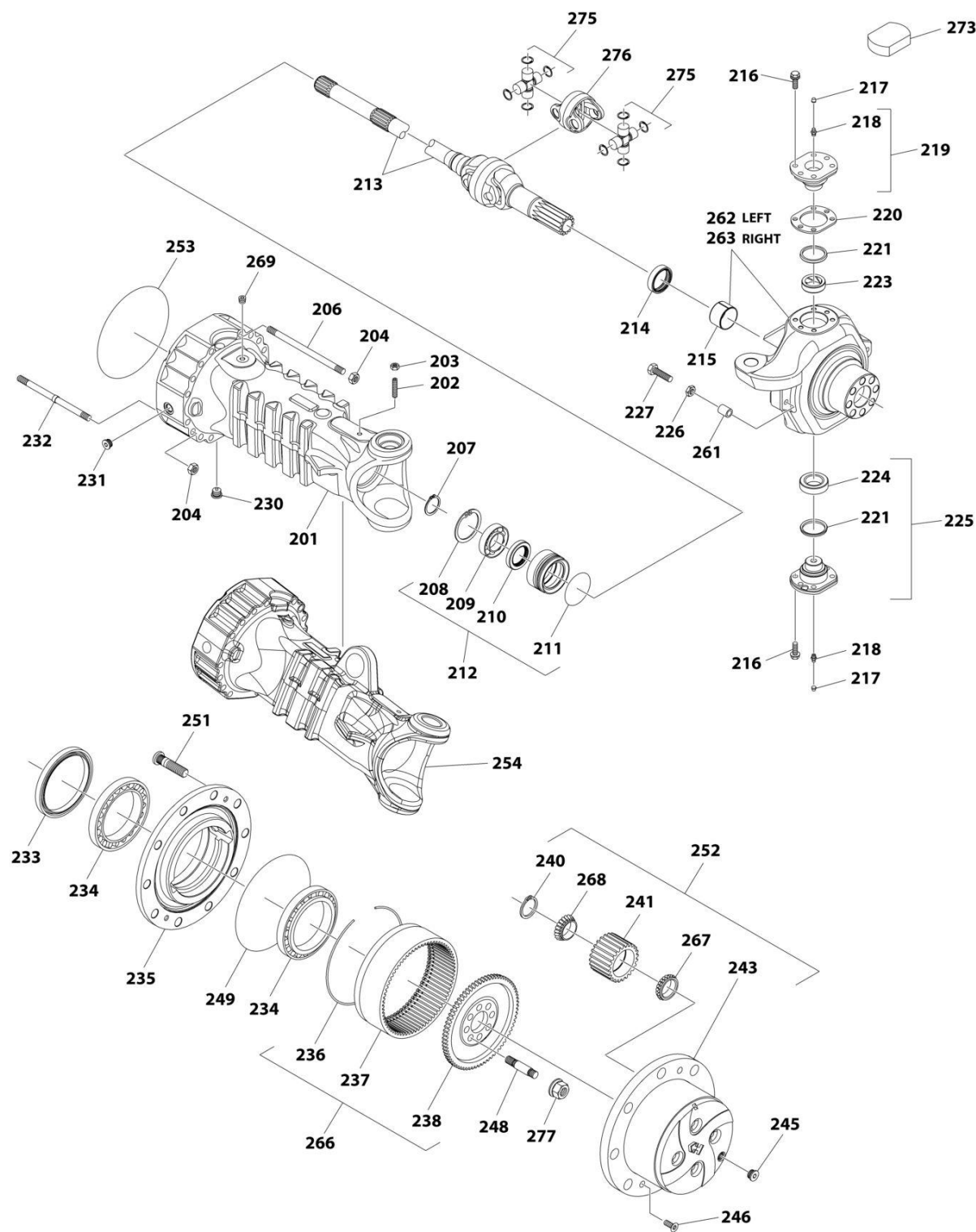
FIGURE 5-25. FRONT (74HP) AXLE ASSEMBLY - HUB REDUCTION
