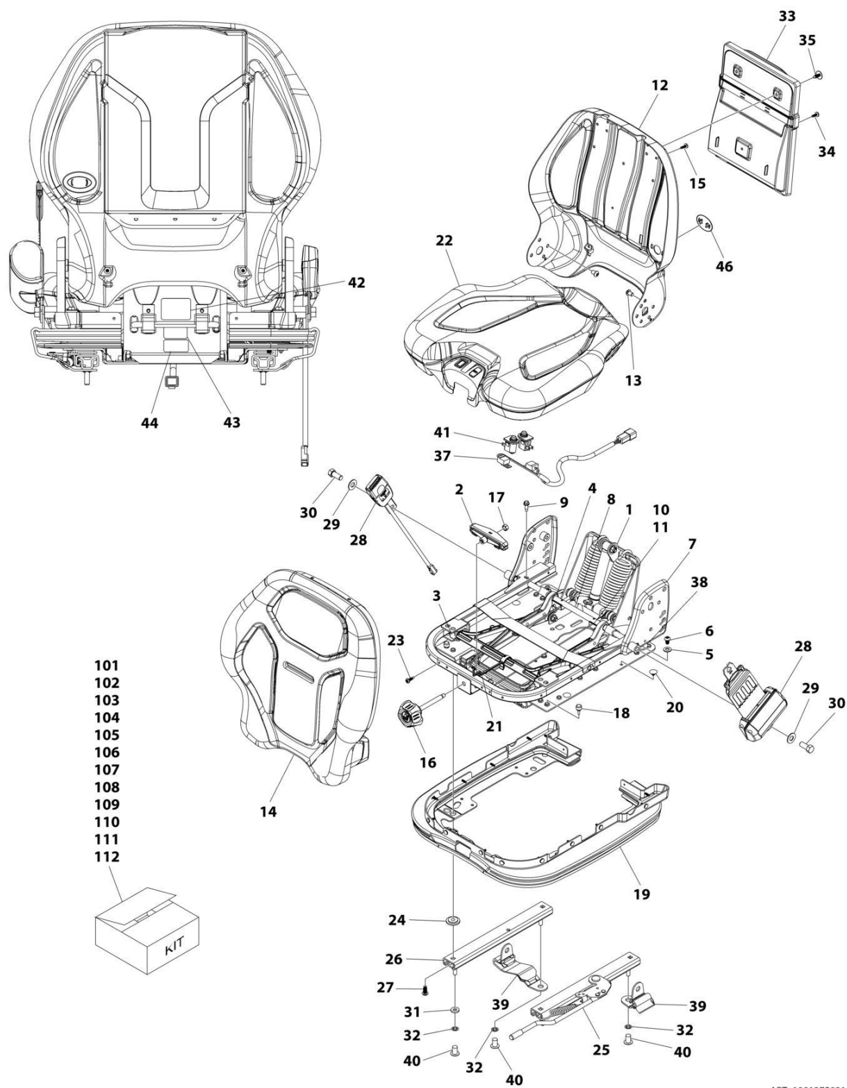
FIGURE 6-20. SEAT ASSEMBLY - VINYL
