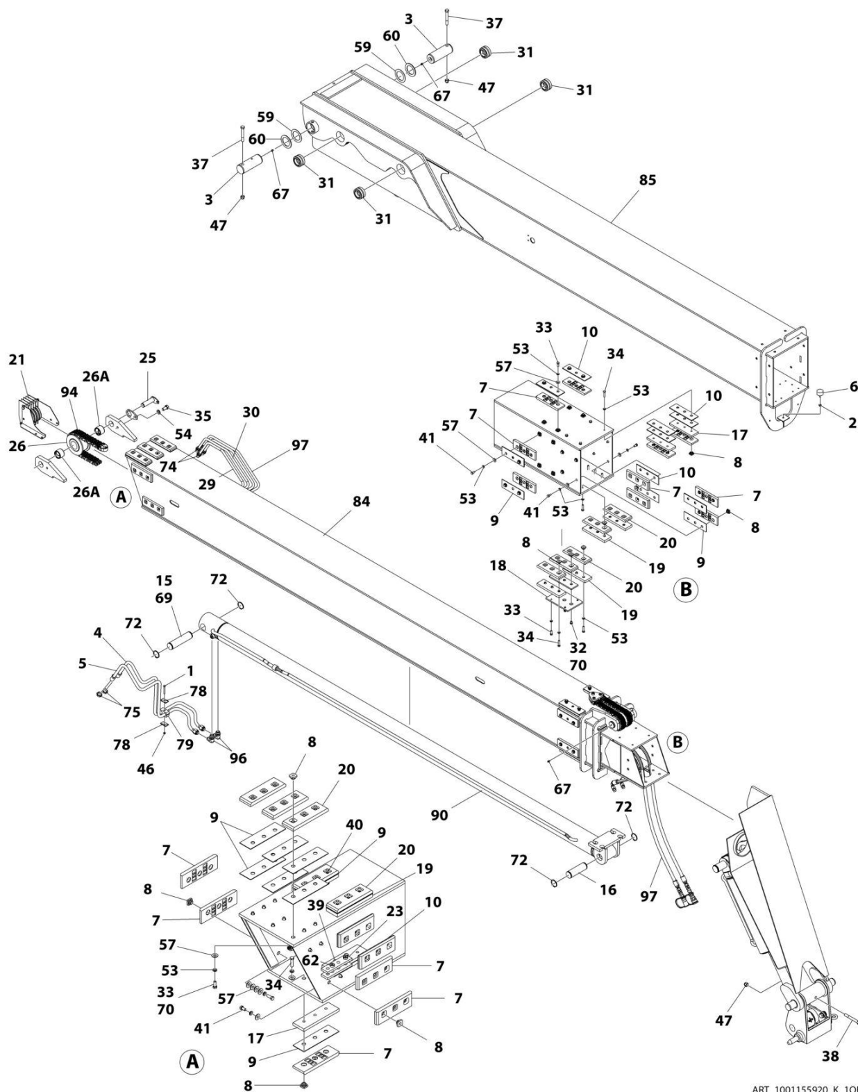
FIGURE 2-1. BOOM INSTALLATION
