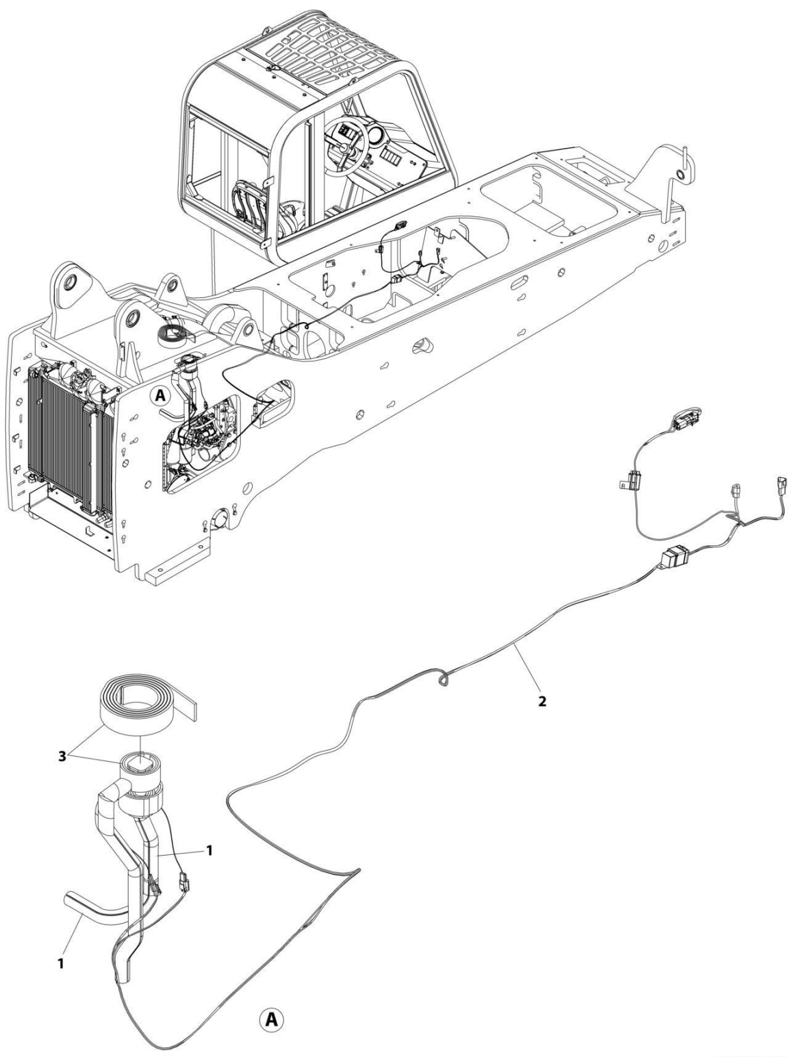
FIGURE 4-15. BREATHER HEATER INSTALLATION (SN 0160143871 to Present)
