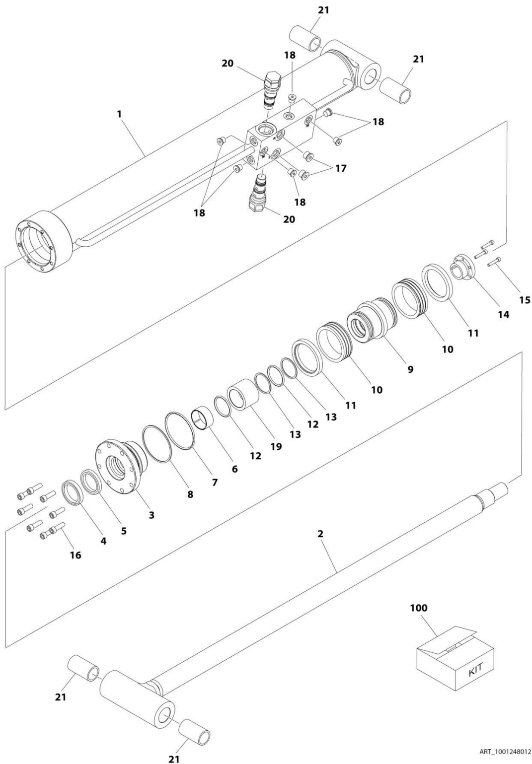
FIGURE 5-3. ARTICULATING JIB LIFT CYLINDER ASSEMBLY (SERVICE REPLACEMENT) (660SJC)
