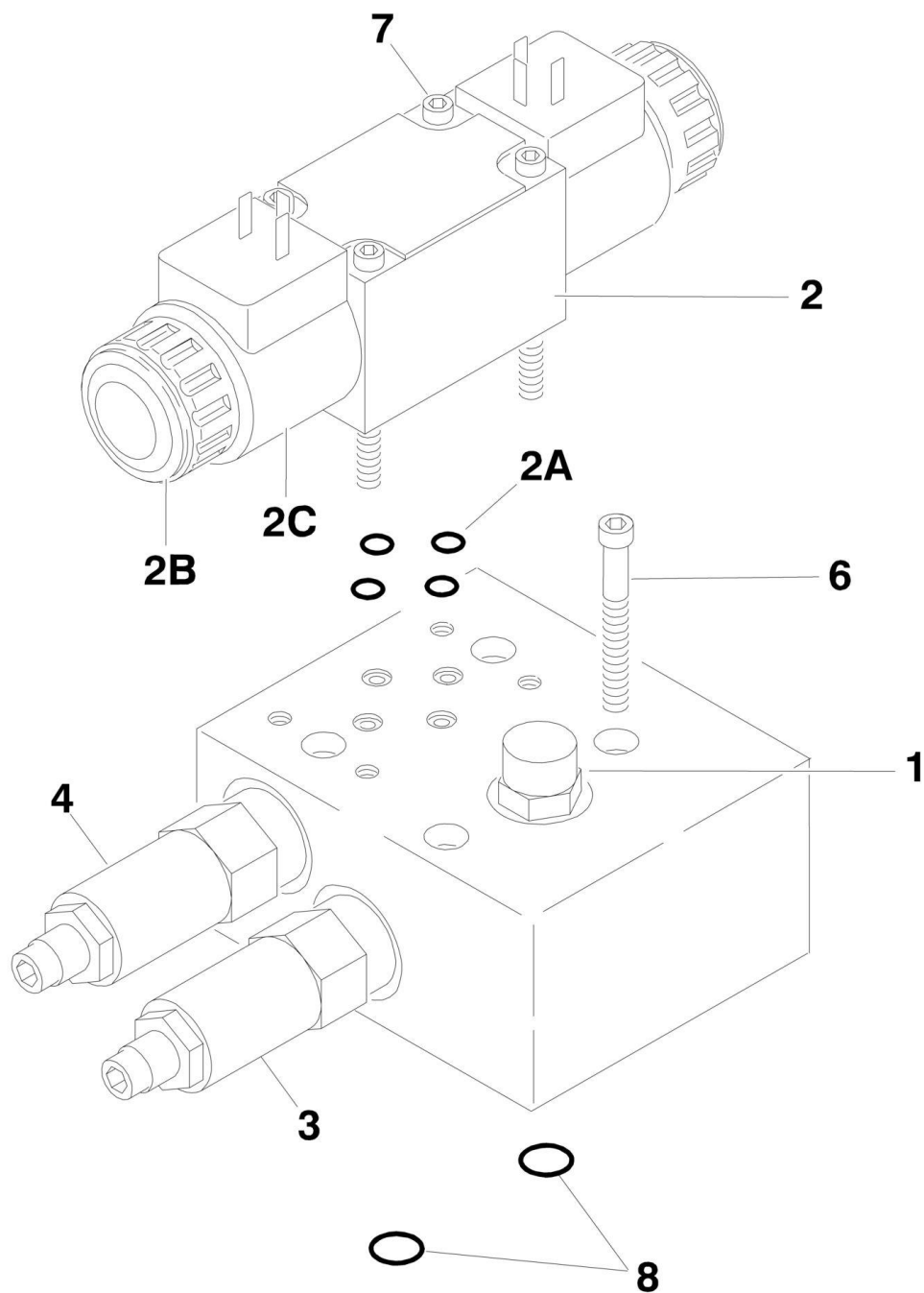
FIGURE 2-3. ARTICULATING JIB VALVE ASSEMBLY (660SJC)
