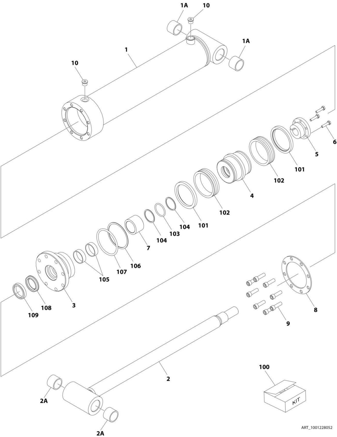
FIGURE 5-13. MASTER CYLINDER ASSEMBLY (SERVICE REPAACEMENT) (660SJC)
