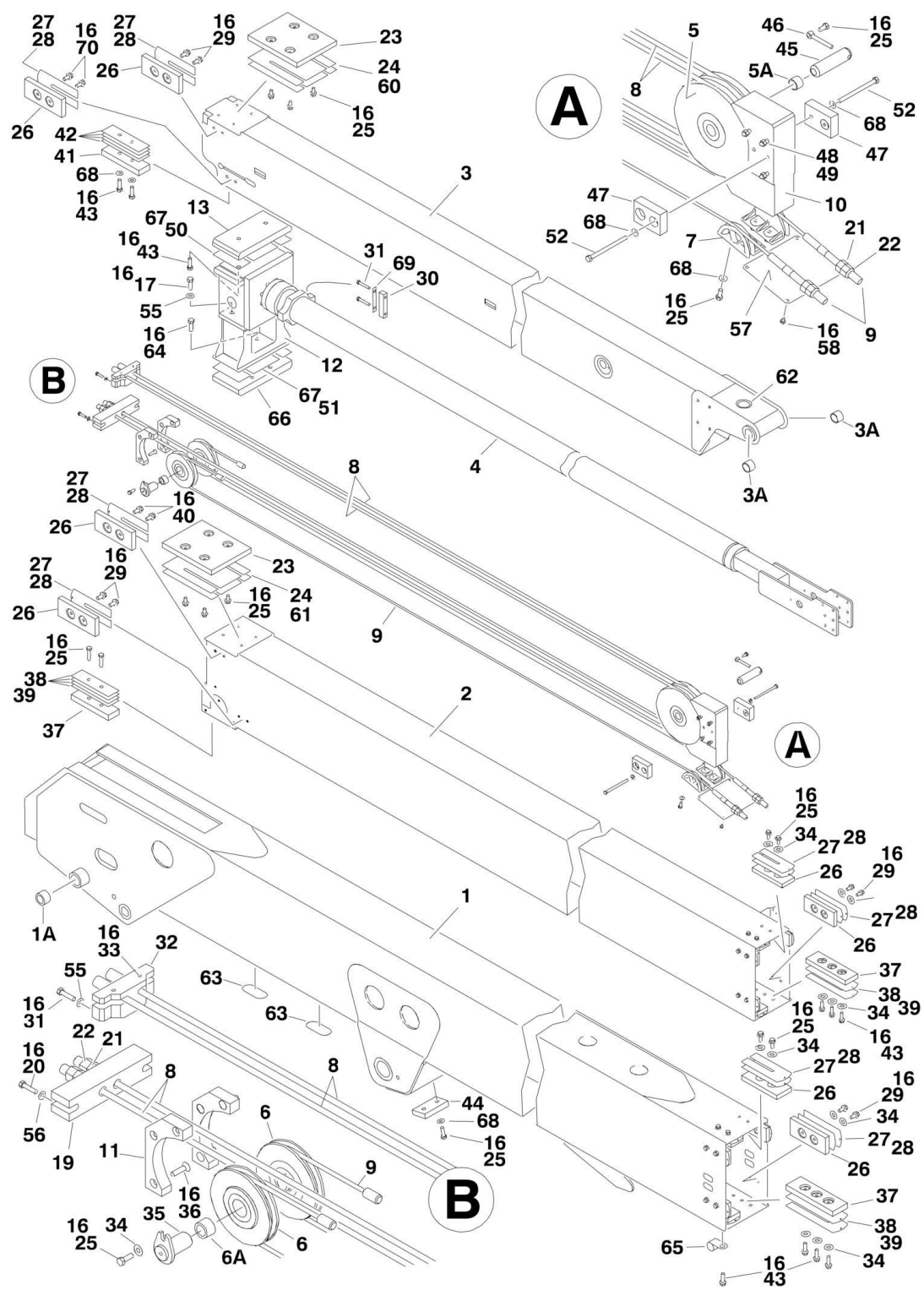
FIGURE 3-3. MAIN BOOM ASSEMBLIES - ANSI AND ANSI EXPORT SPECS
