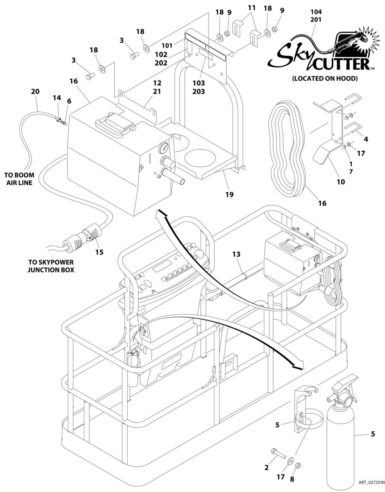
FIGURE 4-8. SKYCUTTER INSTALLATION
