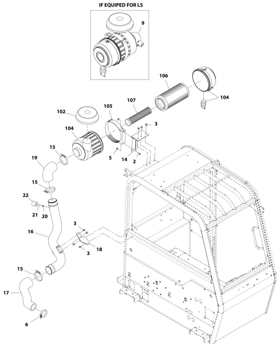
FIGURE 4-54. AIR CLEANER INSTALLATION
