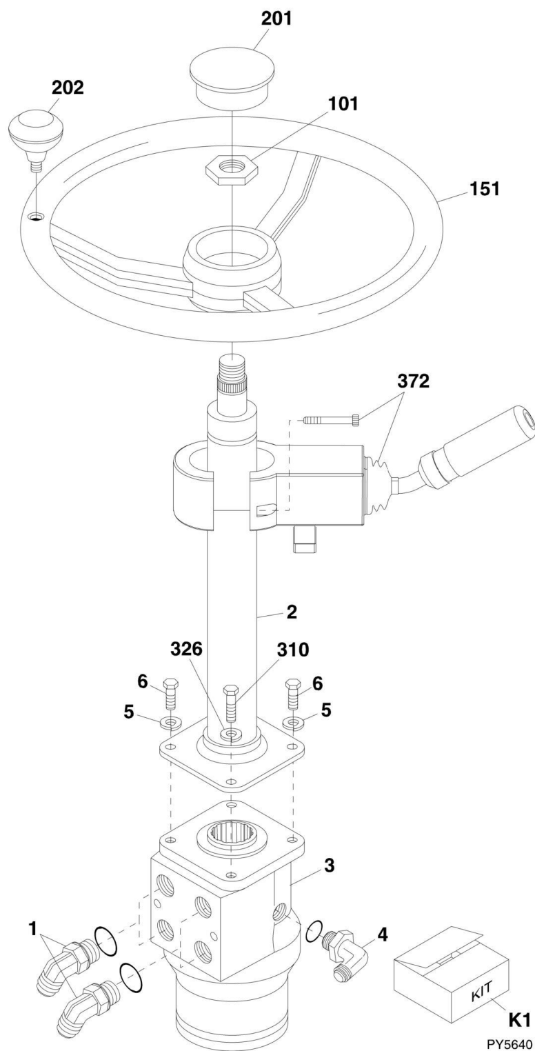
FIGURE 7-9. STEERING COLUMN AND ATTACHING PARTS (SN 0160040675 to Present, Including 0160040468 and 0160040672)
