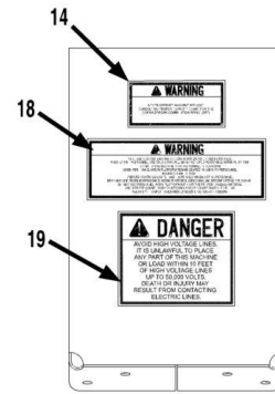
VIEW B-B
