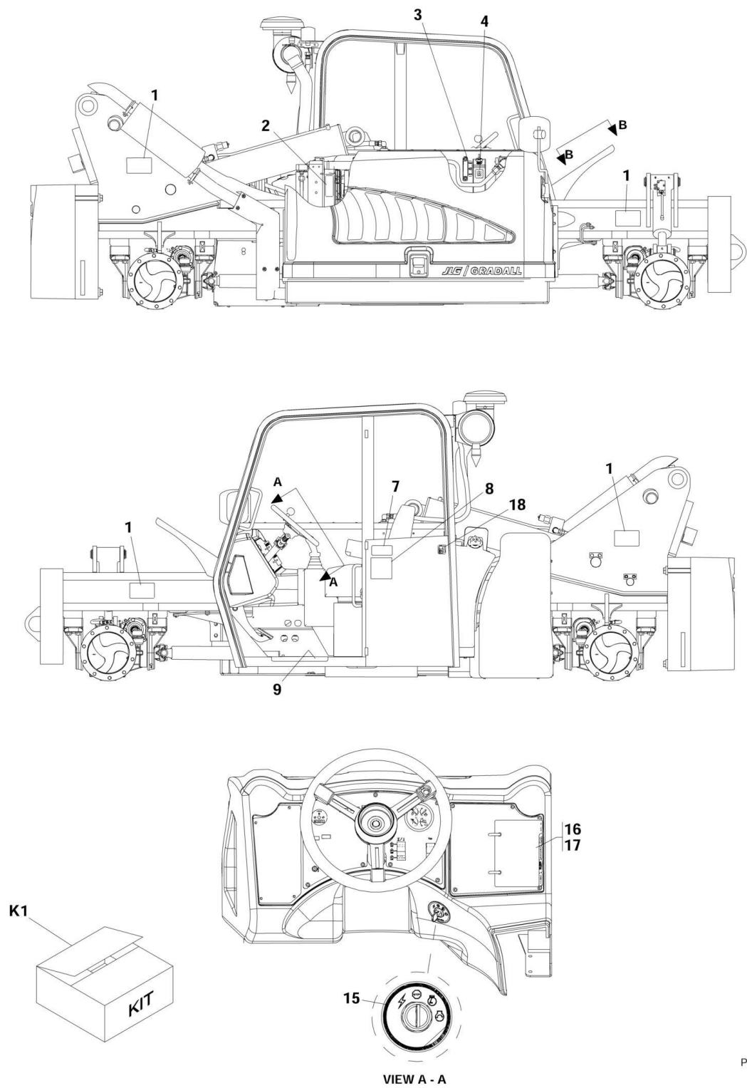
FIGURE 11-2. CAB AND FRAME DECALS (SN 0160000683 through 0160006218)
