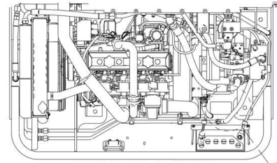
VIEW OF TOP OF ENGINE SN 0160001867 THROUGH 0160006218
