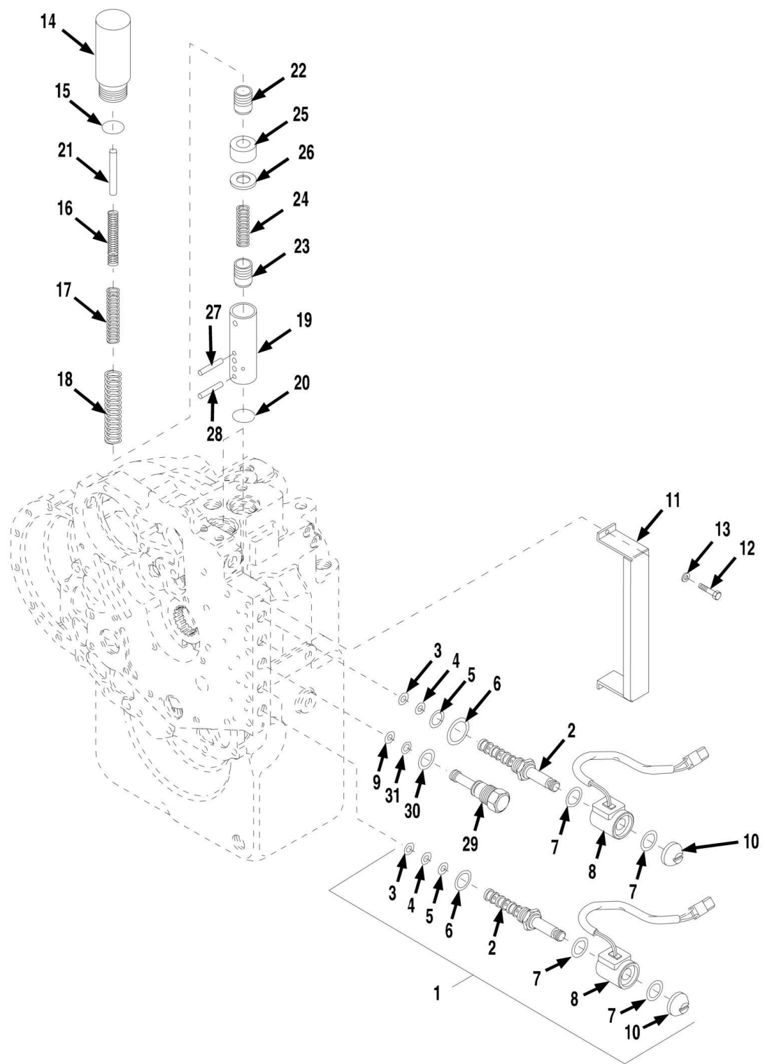
FIGURE 4-35. DANA TRANSMISSION - ELECTRIC CONTROL GROUP (SN 0193001 through 0193007, SN 0160000008 through 0160011036)
