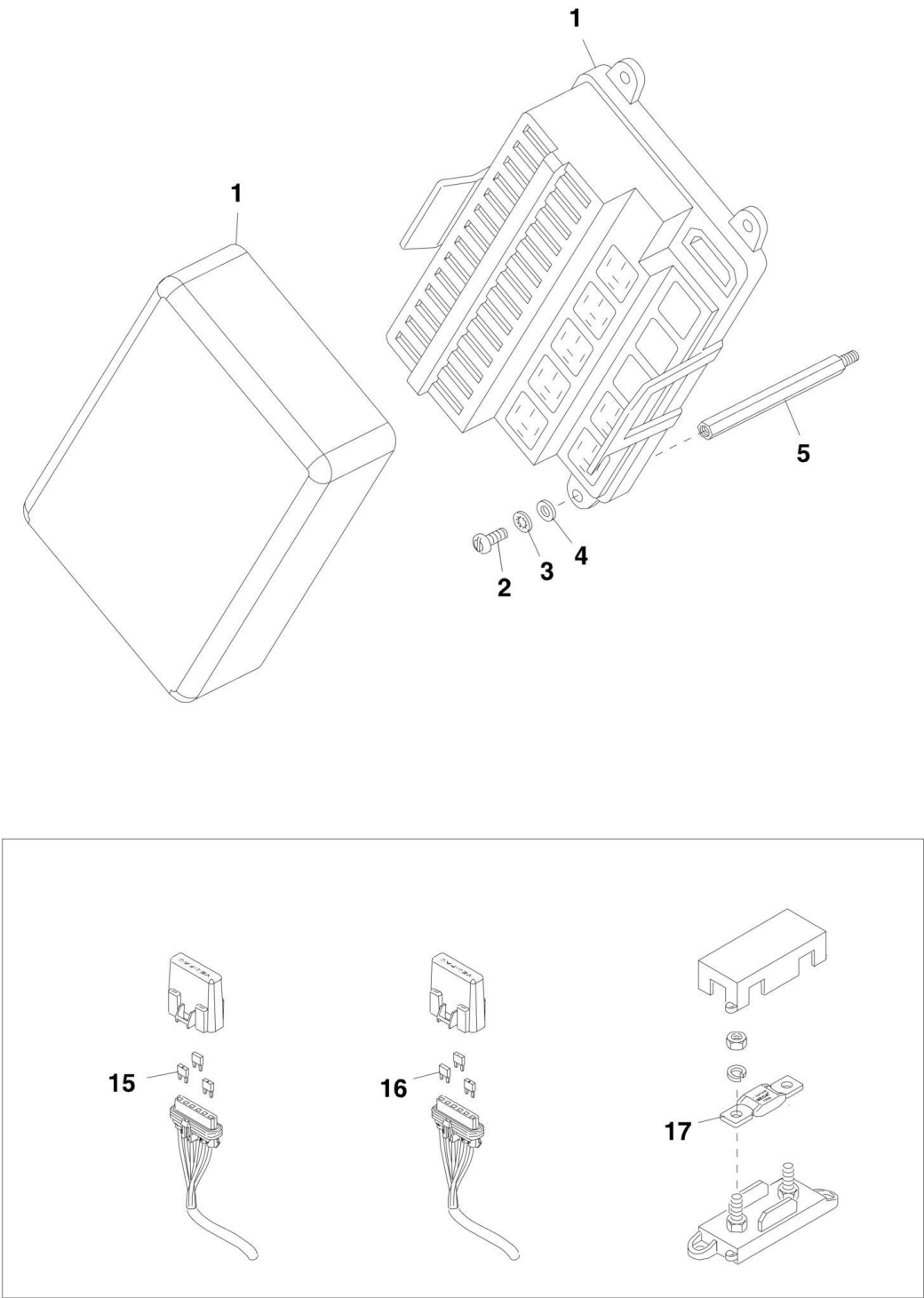
944E ECM POWER HARNESS FIGURE 10-2
