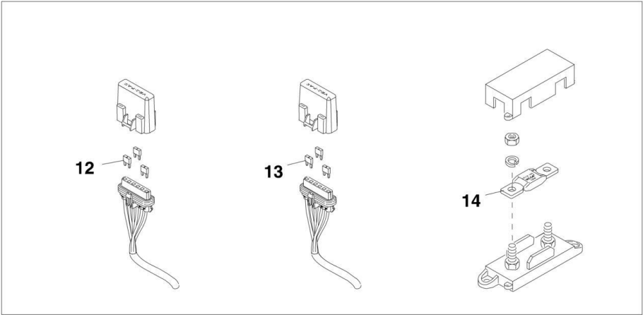
944E ECM POWER HARNESS FIGURE 10-2
