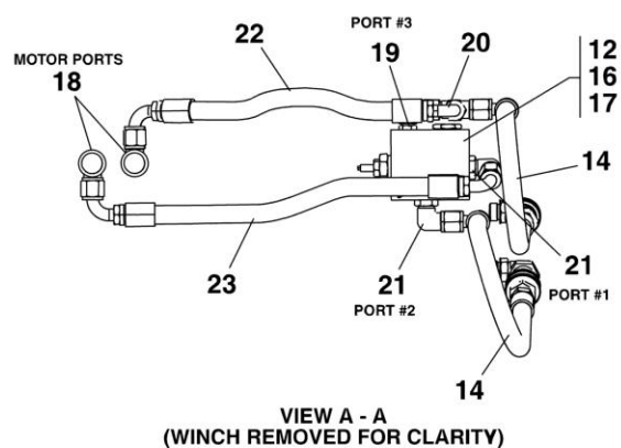
FIGURE 12-10. WINCH INSTALLATION (G10-55A SN 0160024420 to Present; G12-55A SN 0160032083 to Present)
