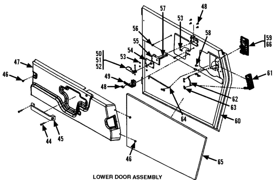
LOWER DOOR ASSEMBLY
