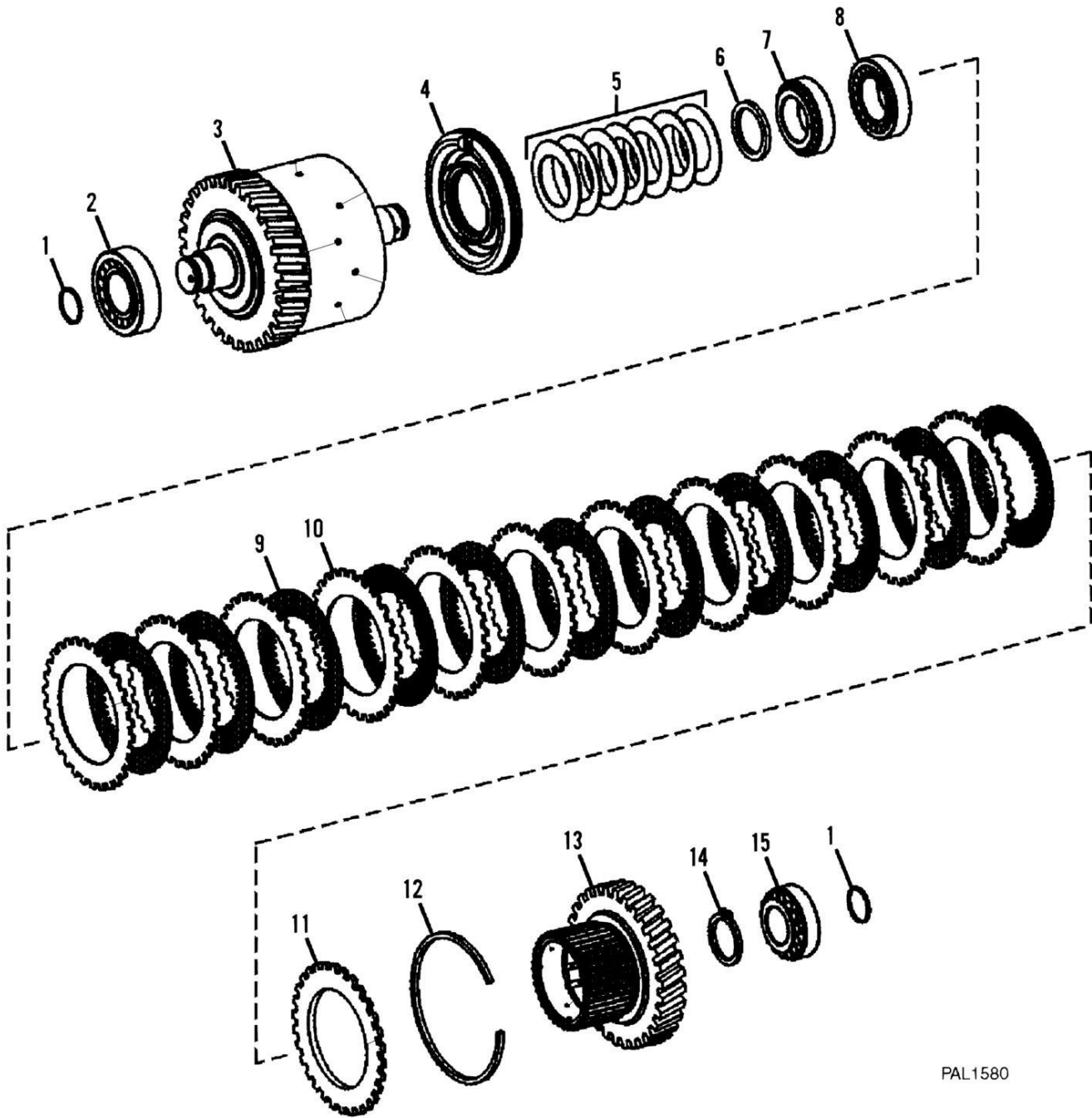
FIGURE 4-23. ZF TRANSMISSION - FORWARD GEAR GROUP
