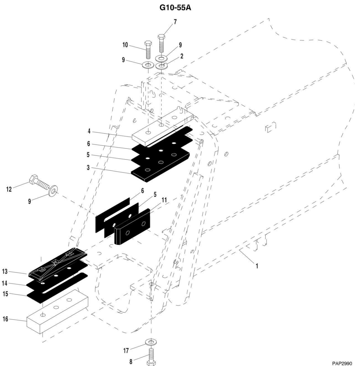
FIGURE 2-3. BEARINGS, PADS, SPACERS AND SHIMS, (FIRST BOOM SECTION) (G10-55A)
