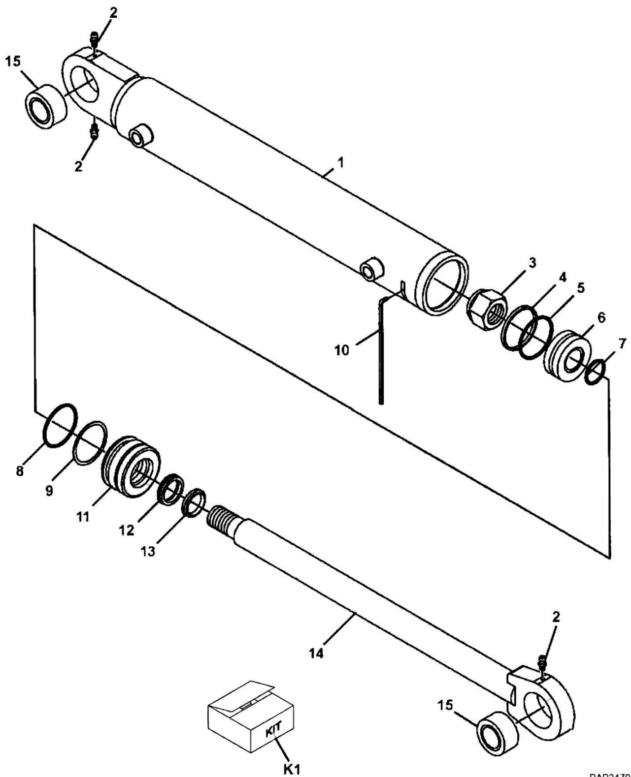
FIGURE 9-57. 180, SWING CARRIAGE CYLINDER
