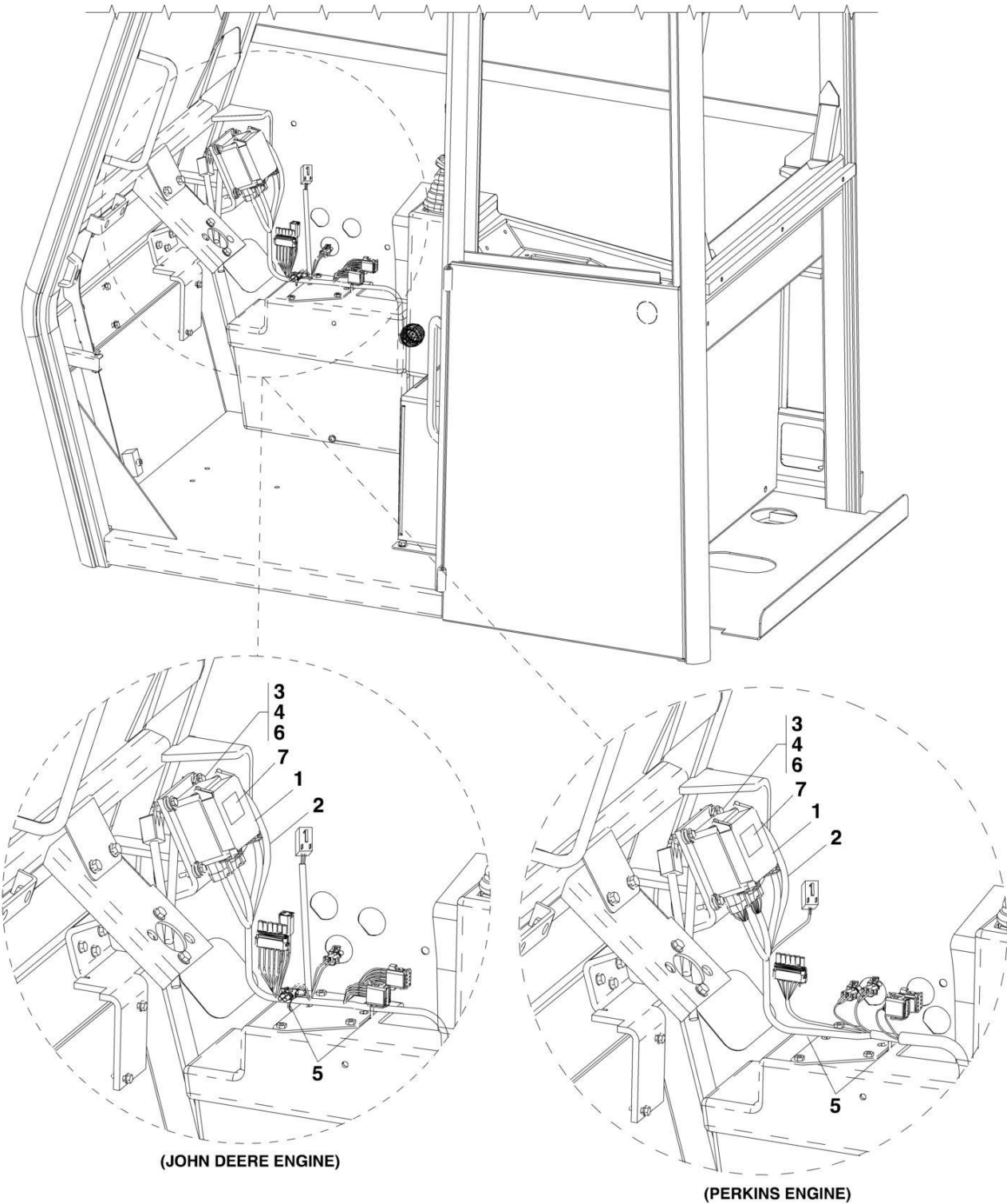
FIGURE 10-25. POWER DISTRIBUTION BOX INSTALLATION
