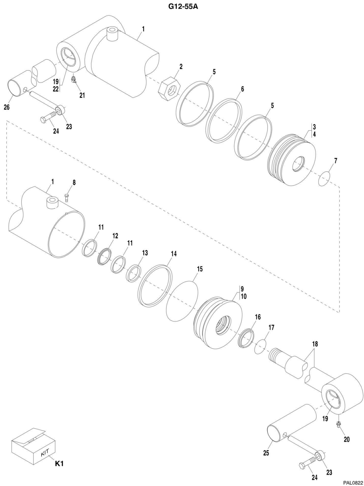
FIGURE 9-31. COMPENSATING CYLINDER (G12-55A) (G12-55A Prior to SN 0160033659; Excluding 0160033452)
