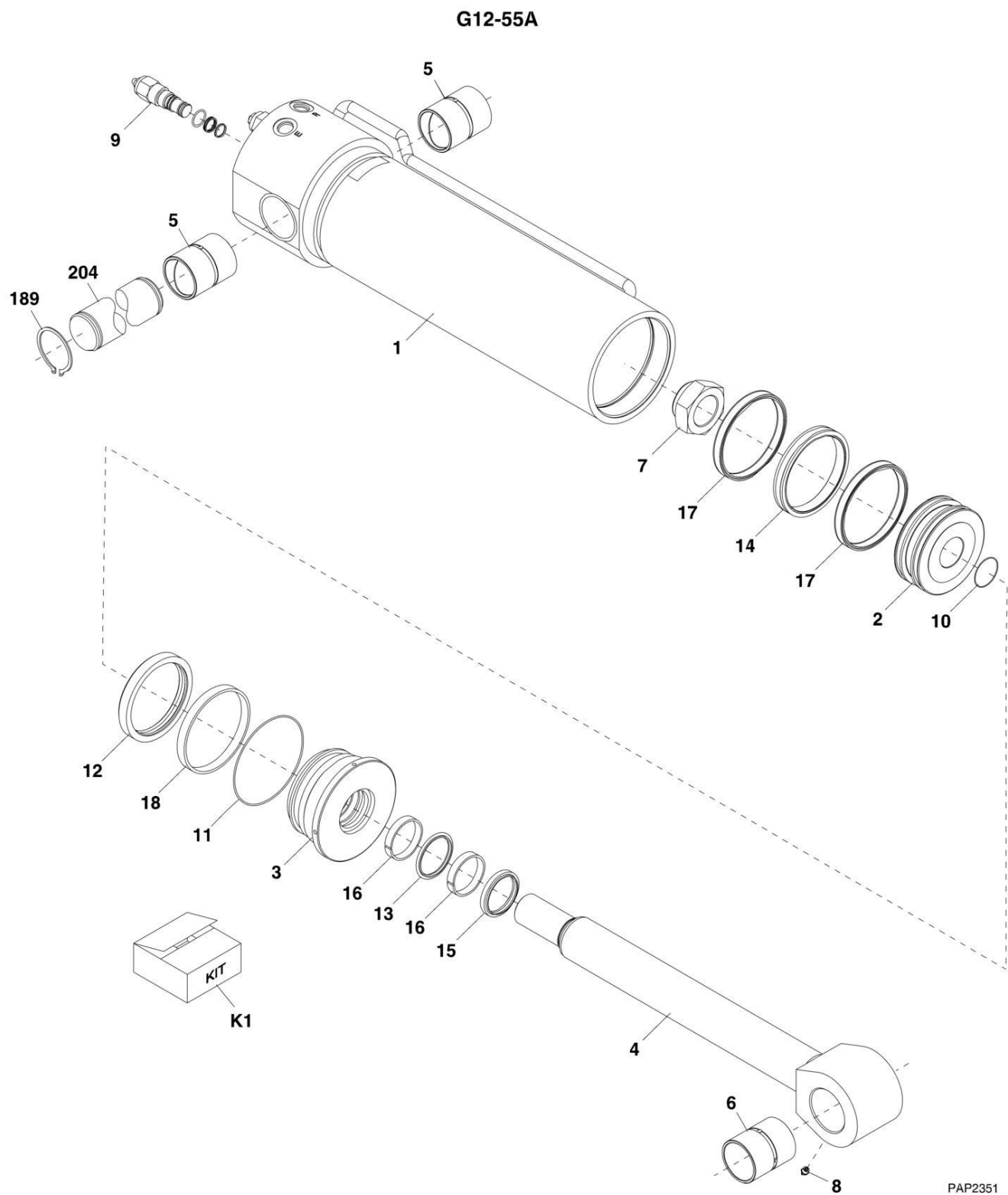
FIGURE 9-26. TILT CYLINDER (G12-55A) (G12-55A SN 0160037689 to Present)
