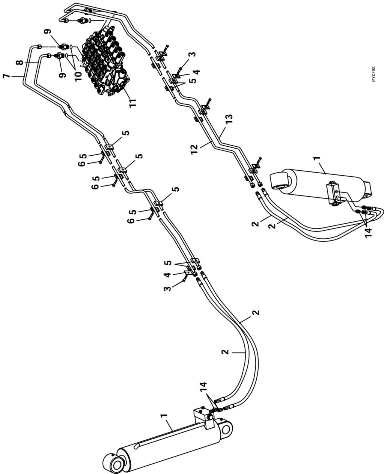
FIGURE 8-37. OUTRIGGER CYLINDERS - PERKINS ENGINE
