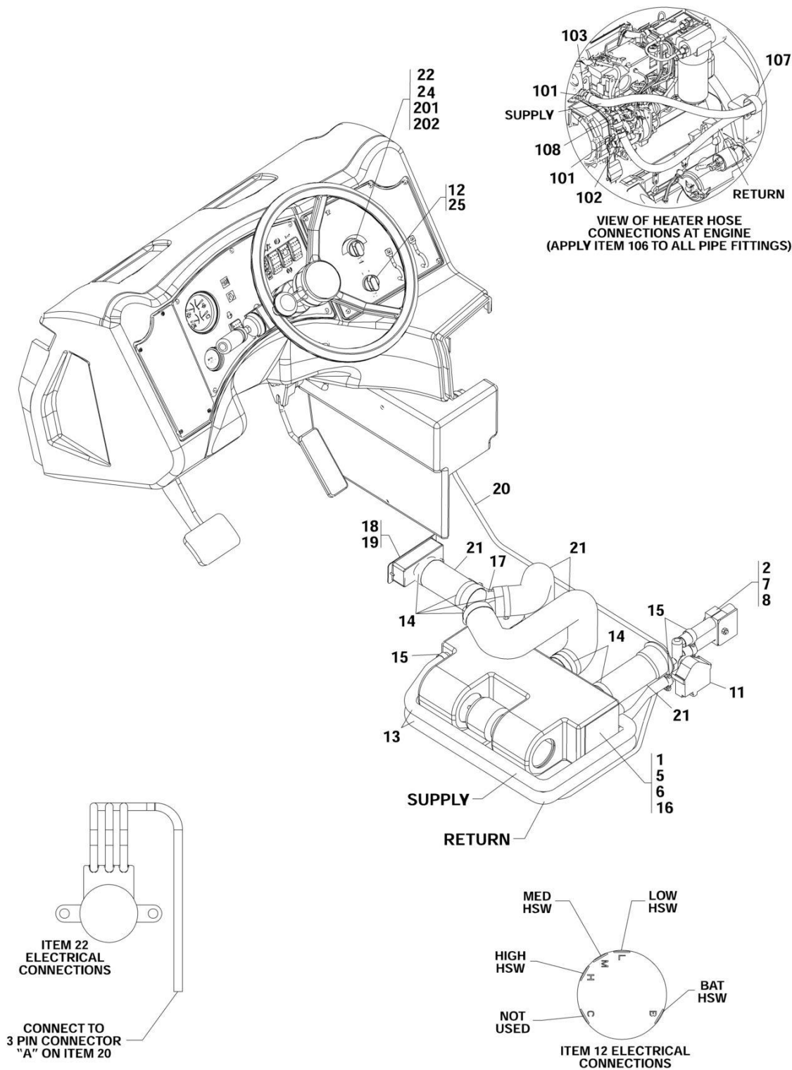
FIGURE 6-10. OPEN CAB HEATER (Prior to SN 0160039103, Excluding 0160038973)
