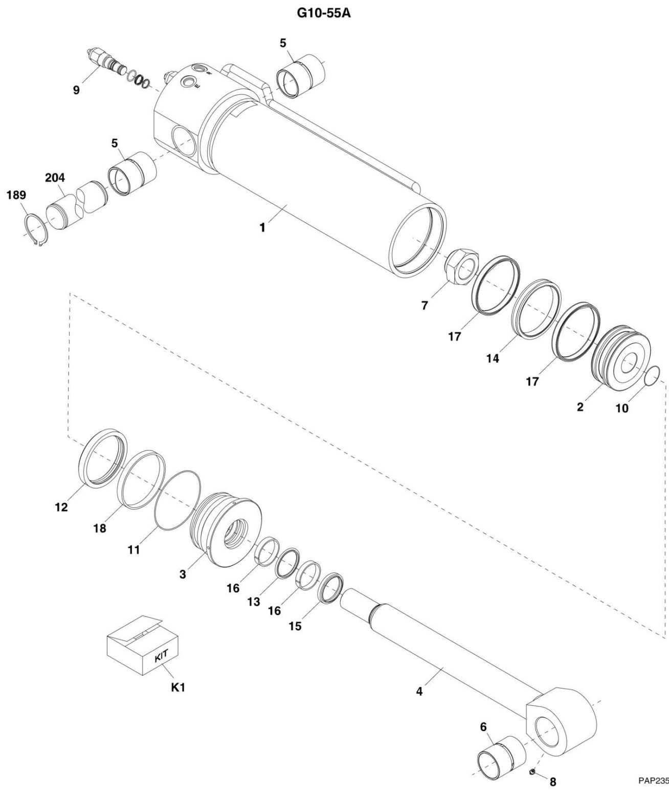
FIGURE 9-22. TILT CYLINDER (G10-55A) (G10-55A SN 0160037689 to Present)
