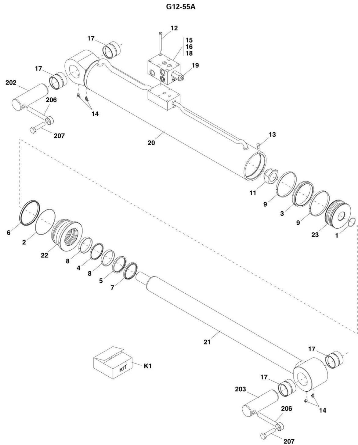
FIGURE 9-8. LIFT CYLINDER (G12-55A) (G12-55A SN 0160033659 through 0160035879; Including 0160033452)
