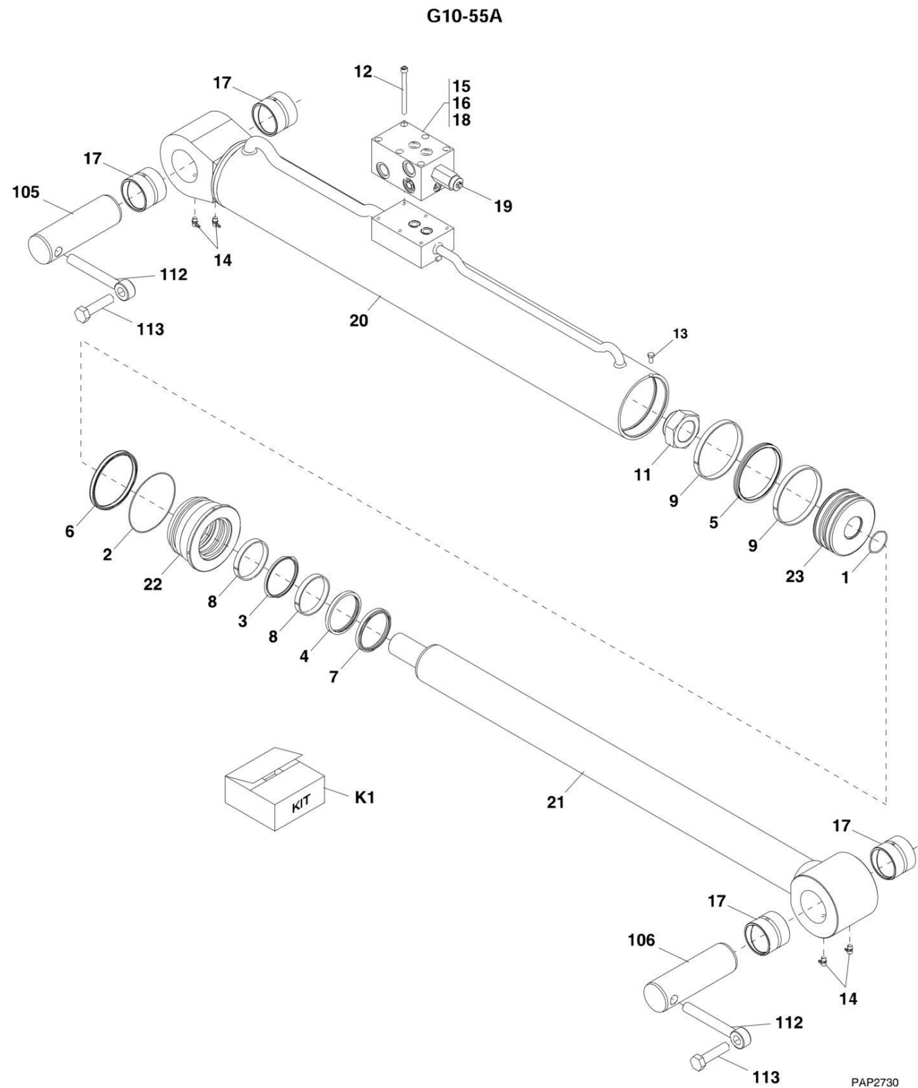
FIGURE 9-2. LIFT CYLINDER (G10-55A) (G10-55A SN 0160033659 through 0160035822; Including 0160033452)
