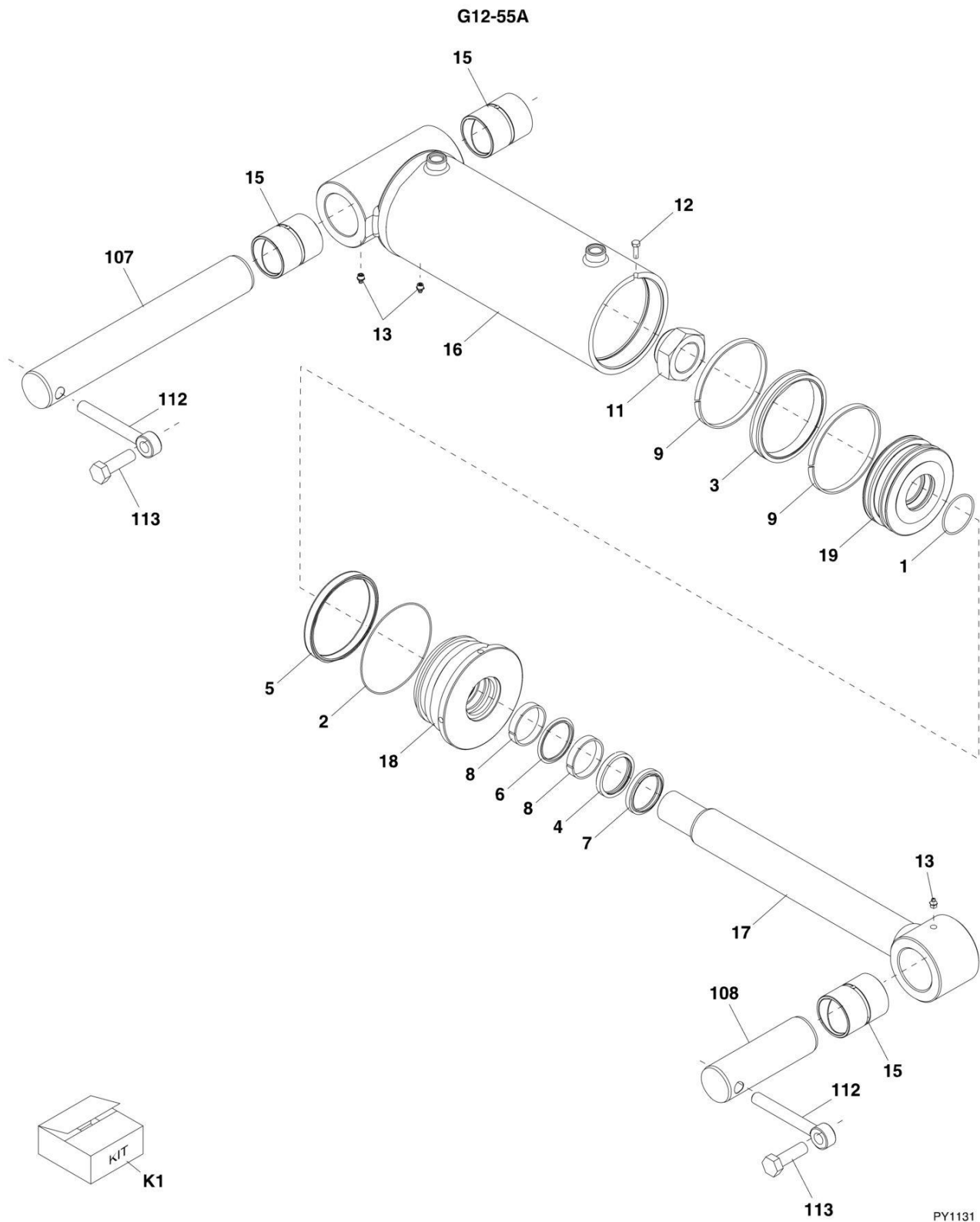
FIGURE 9-32. COMPENSATING CYLINDER (G12-55A) (G12-55A SN 0160033659 through 0160037689; Including 0160033452)
