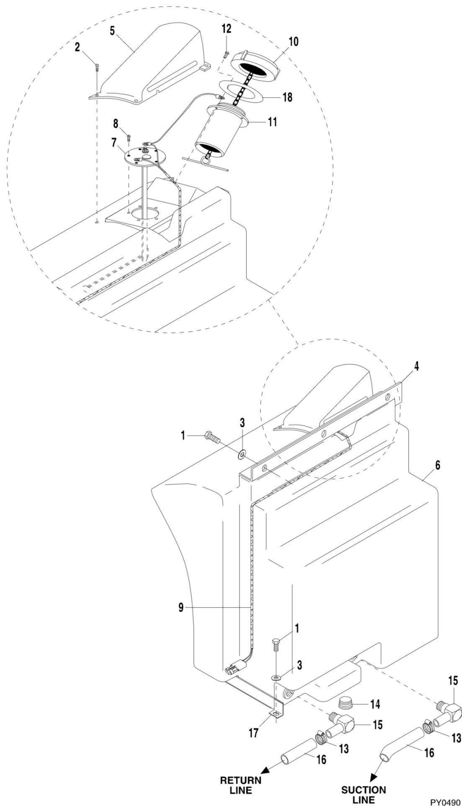
FIGURE 4-7. FUEL TANK AND LINES (Prior to SN 0160020149)
