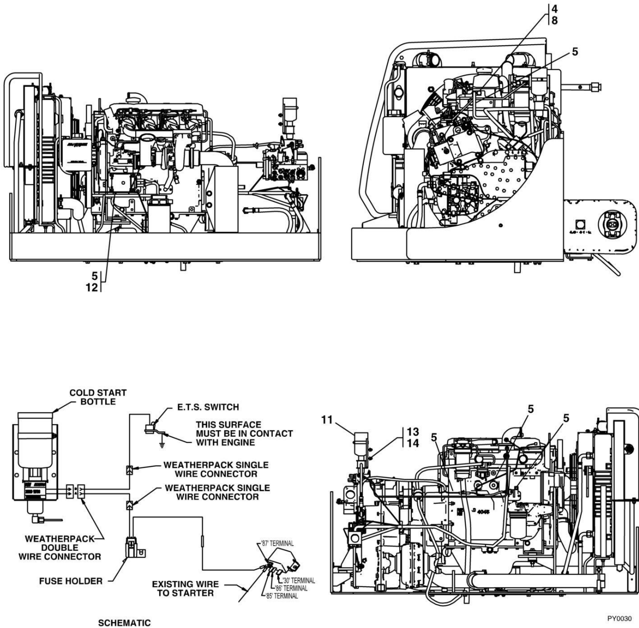
FIGURE 12-4. COLD START INSTALLATION - JOHN DEERE ENGINE
