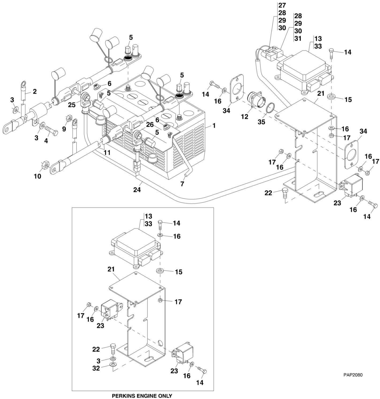
FIGURE 10-1. BATTERY AND CABLES - JOHN DEERE AND PERKINS ENGINE
