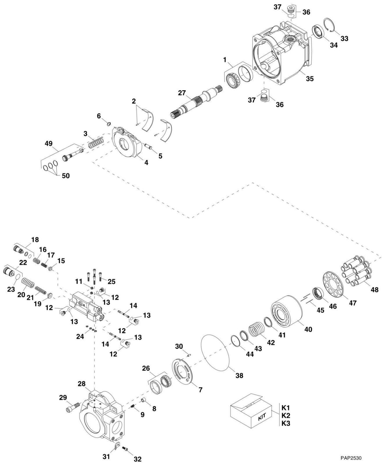
FIGURE 9-47. HYDRAULIC PUMP - CUMMINS ENGINE
