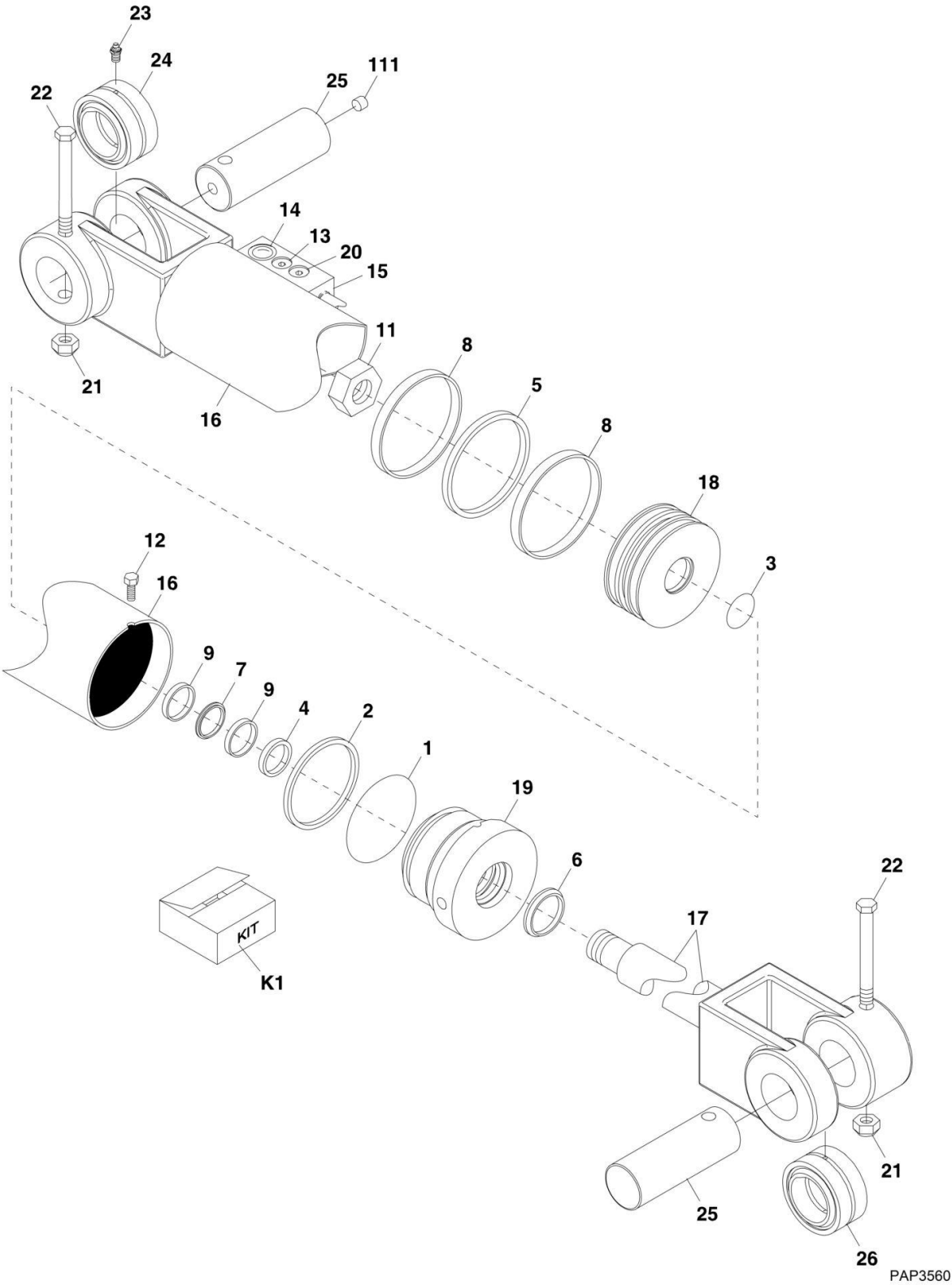
FIGURE 9-40. STABILIZER CYLINDER (G10-55A SN 0160033661 through 0160039837; G12-55A SN 0160033659 through 0160039838)
