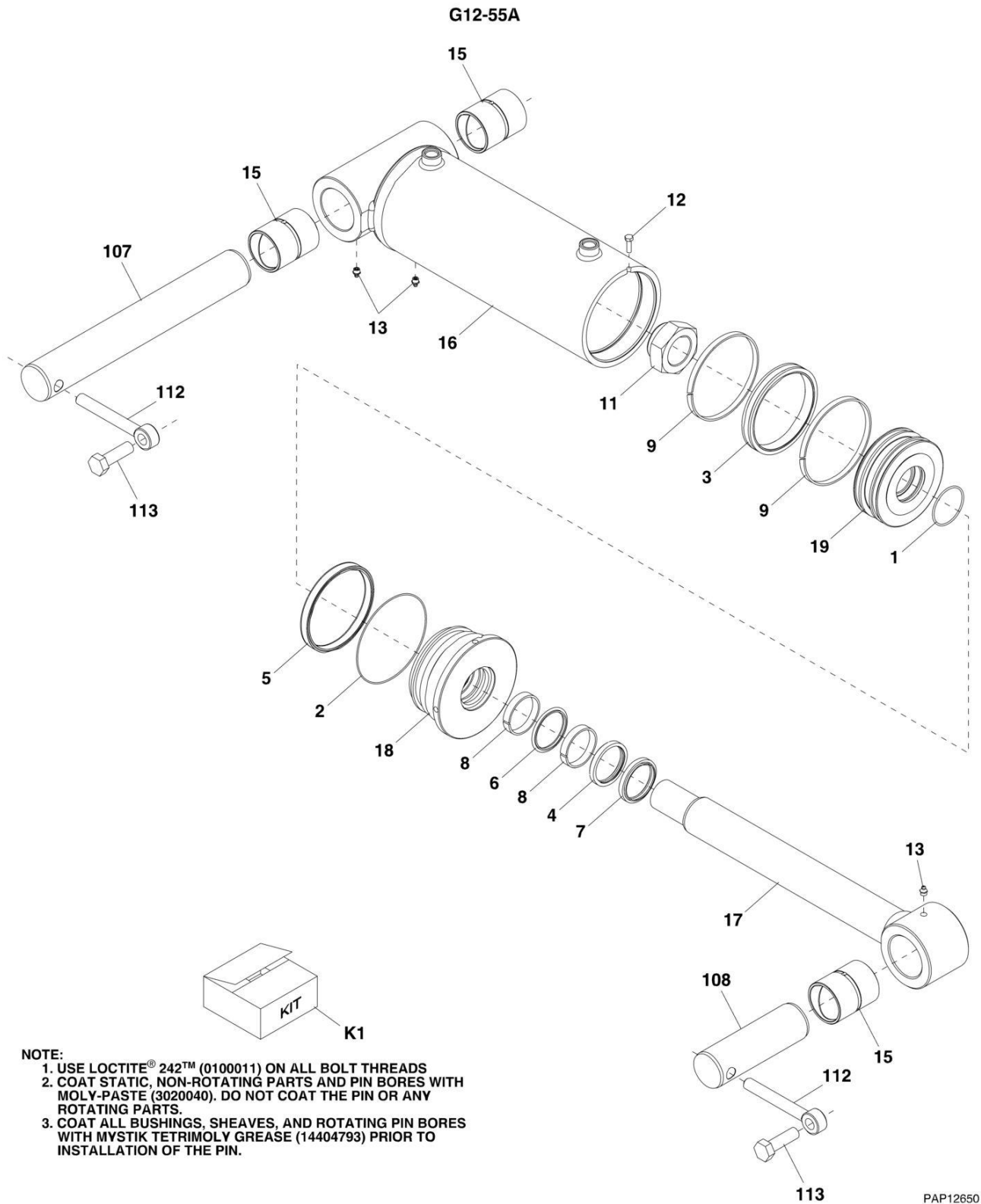
FIGURE 9-33. COMPENSATING CYLINDER (G12-55A) (G12-55A SN 0160037689 through 0160041564)
