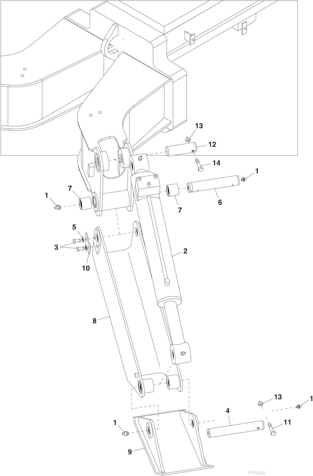
FIGURE 1-4. OUTRIGGER MOUNTING
