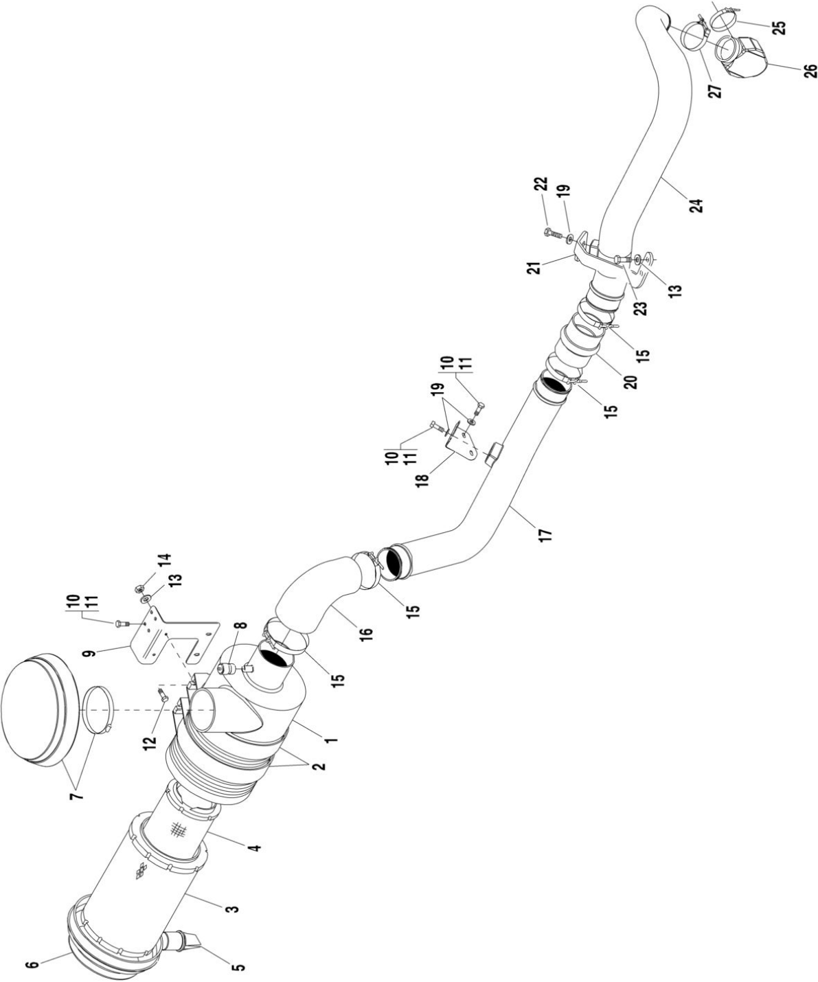
FIGURE 4-12. AIR CLEANER INSTALLATION - JOHN DEERE ENGINE (G10-55A)
