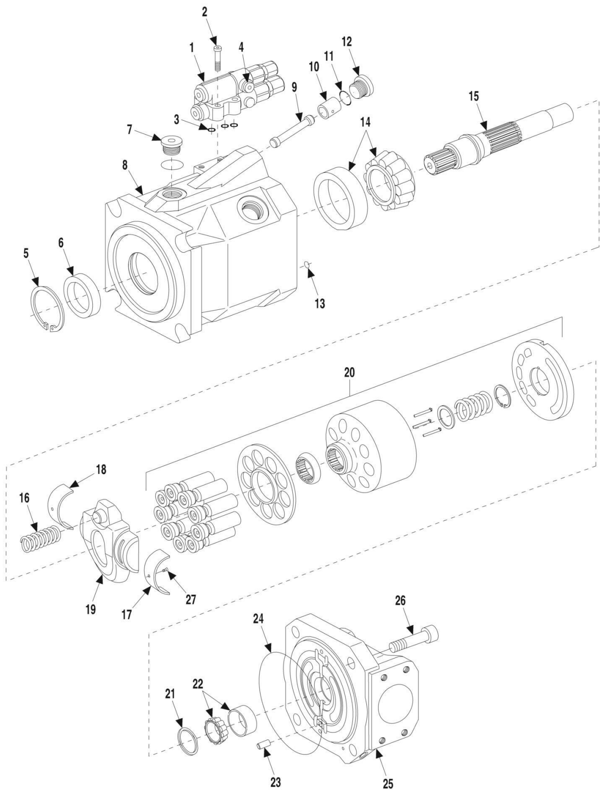
FIGURE 9-46. HYDRAULIC PUMP
