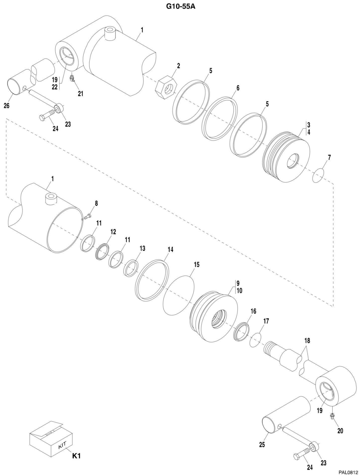
FIGURE 9-27. COMPENSATING CYLINDER (G10-55A) (G10-55A Prior to SN 0160033659; Excluding 0160033452)
