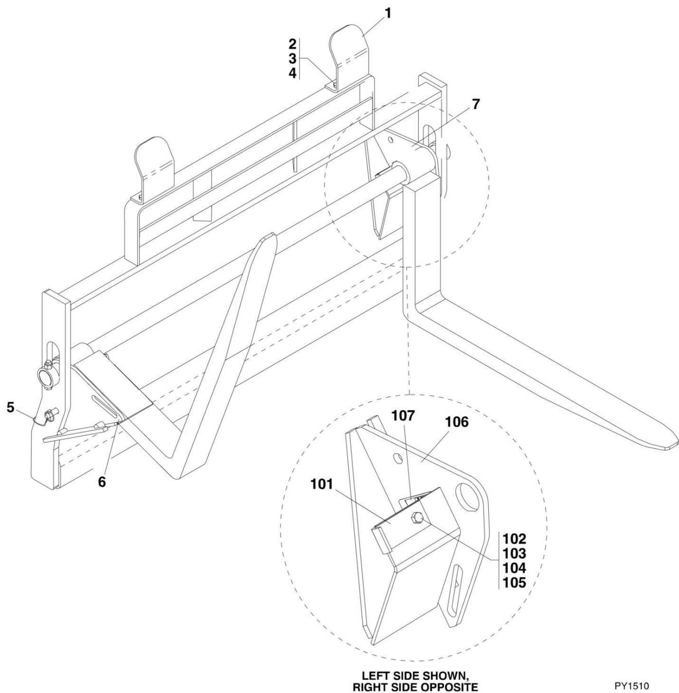
FIGURE 3-13. SHEET MATERIAL HANDLER (SN 0160037689 to Present)
