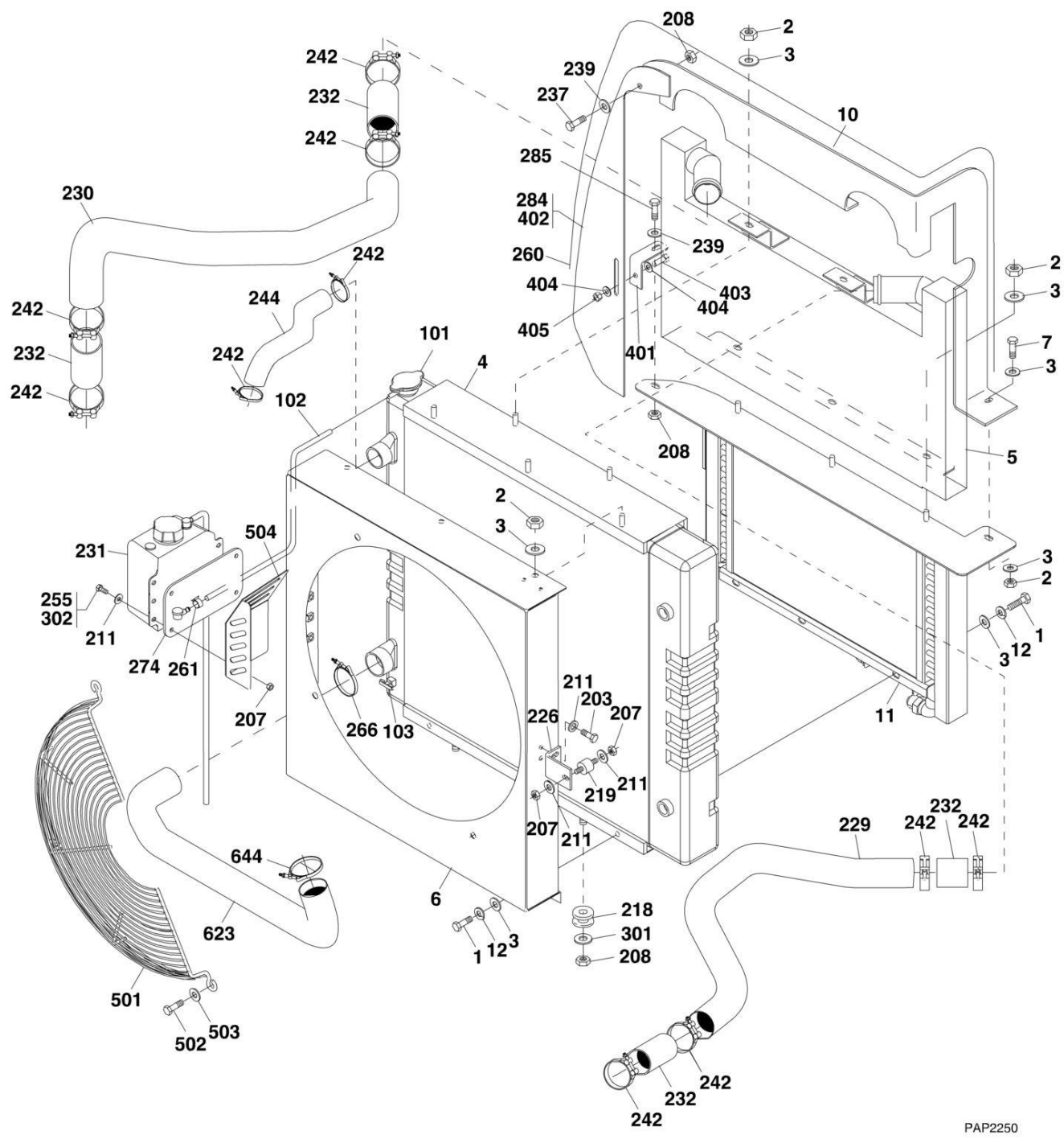
FIGURE 4-9. RADIATOR ASSEMBLY - JOHN DEERE ENGINE
