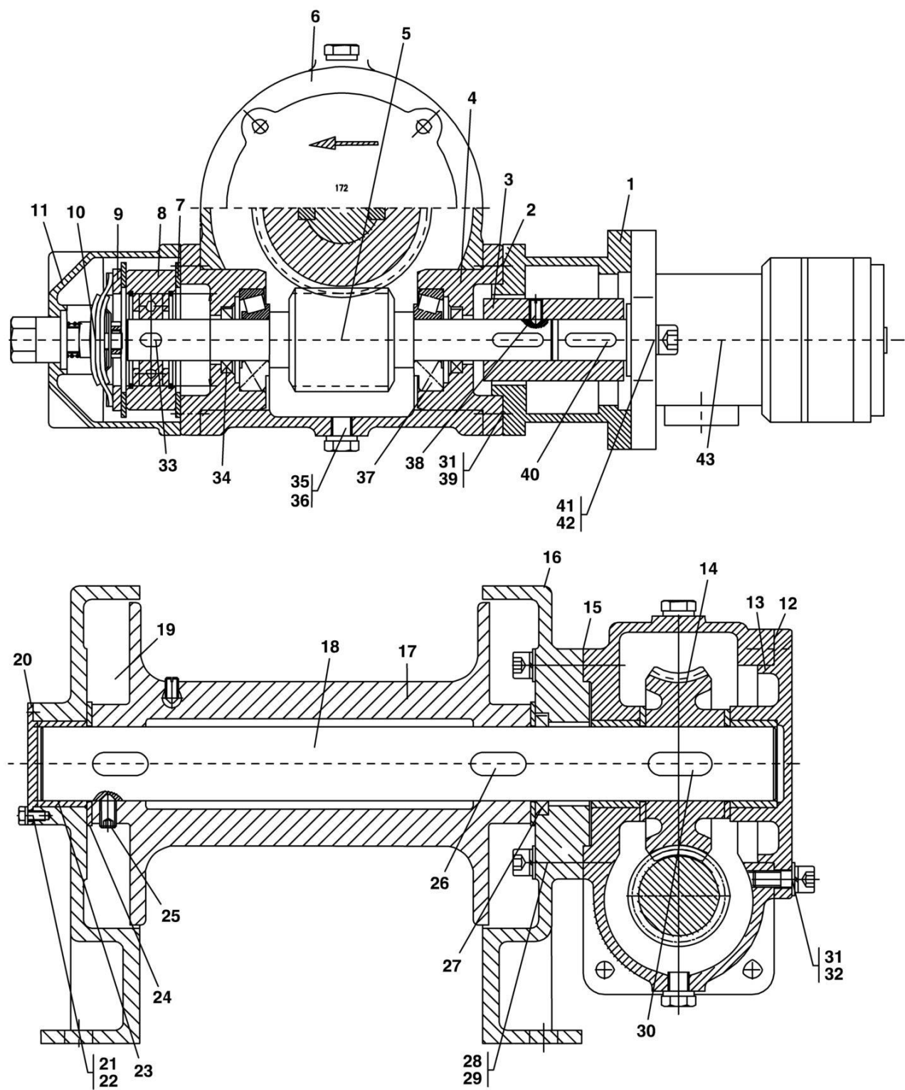
FIGURE 12-25. WINCH
