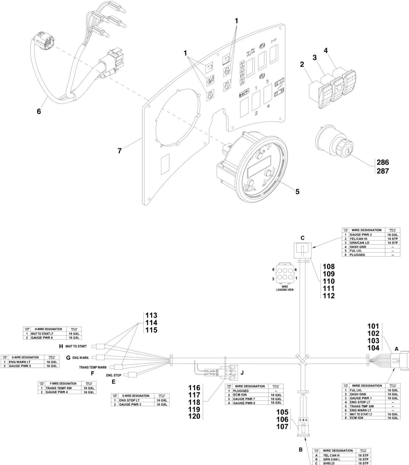
FIGURE 6-8. INSTRUMENT PANEL (SN 0160037186 to Present)
