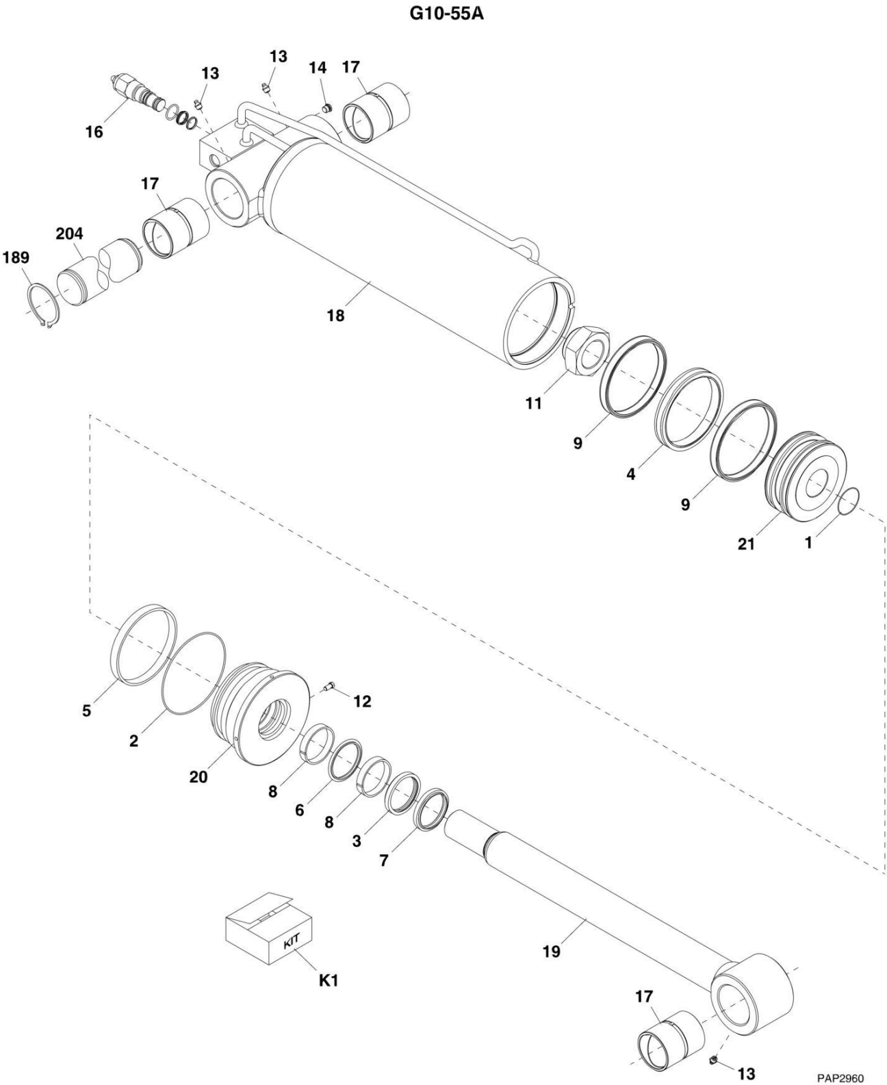
FIGURE 9-21. TILT CYLINDER (G10-55A) (G10-55A SN 0160035822 through 0160037689)
