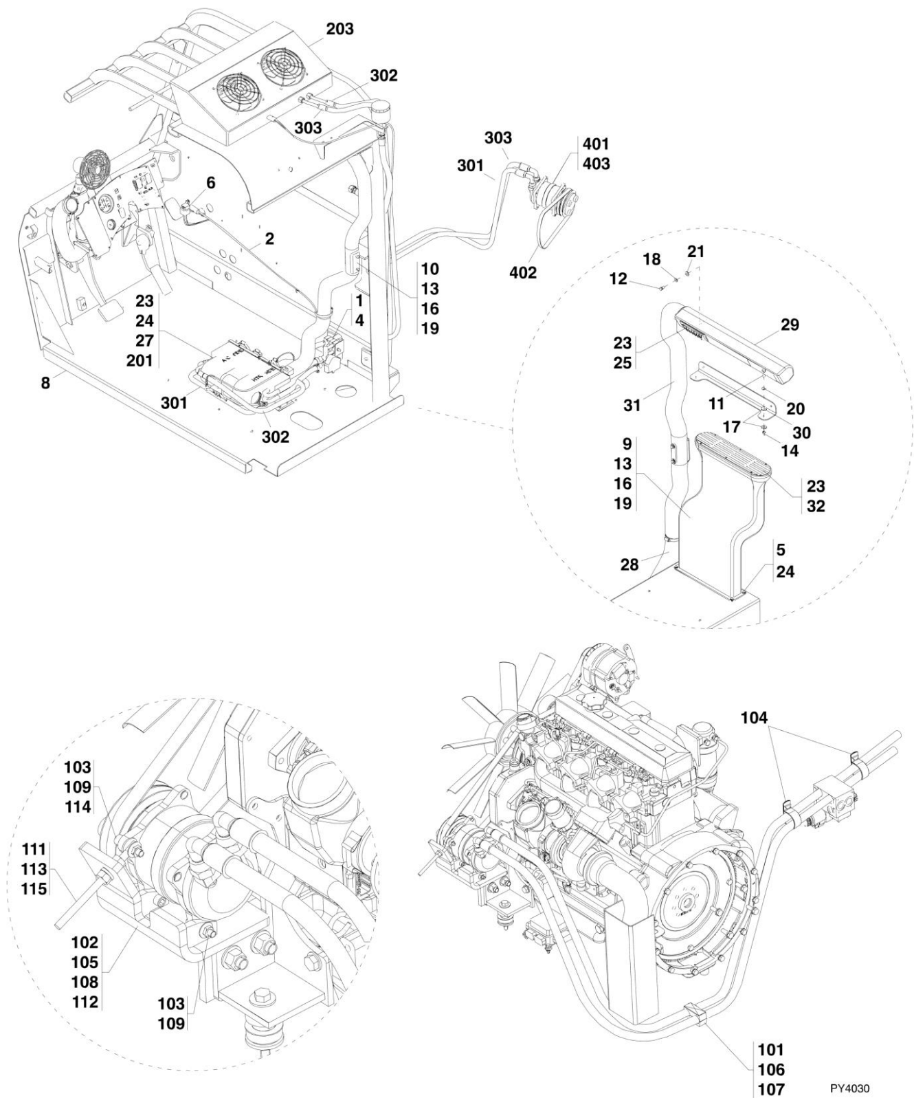
FIGURE 6-12. AIR CONDITIONING - JOHN DEERE ENGINE
