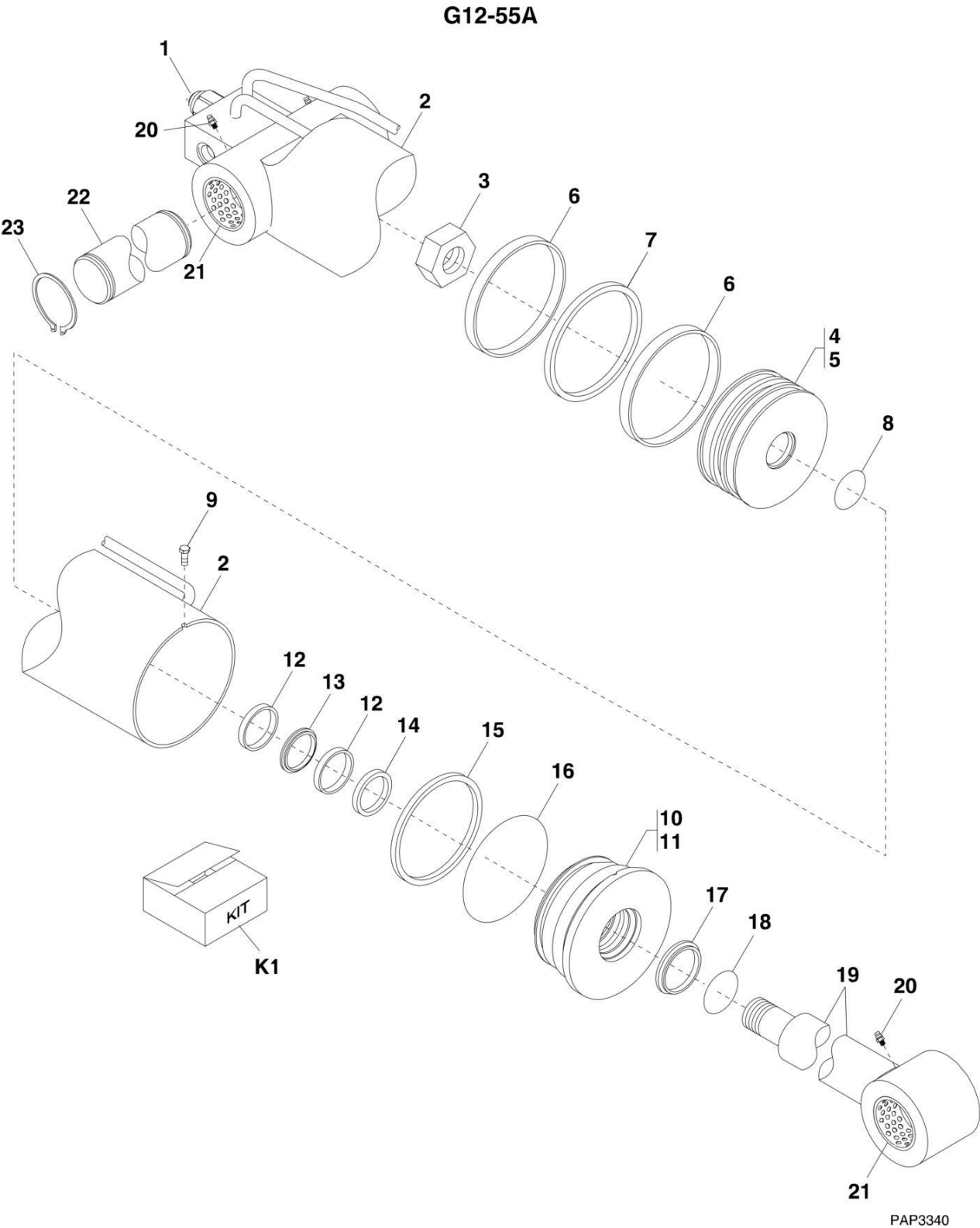
FIGURE 9-23. TILT CYLINDER (G12-55A) (G12-55A Prior to SN 0160033659; Excluding 0160033452)
