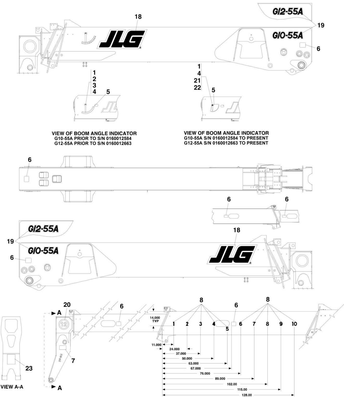
FIGURE 11-3. BOOM DECALS
