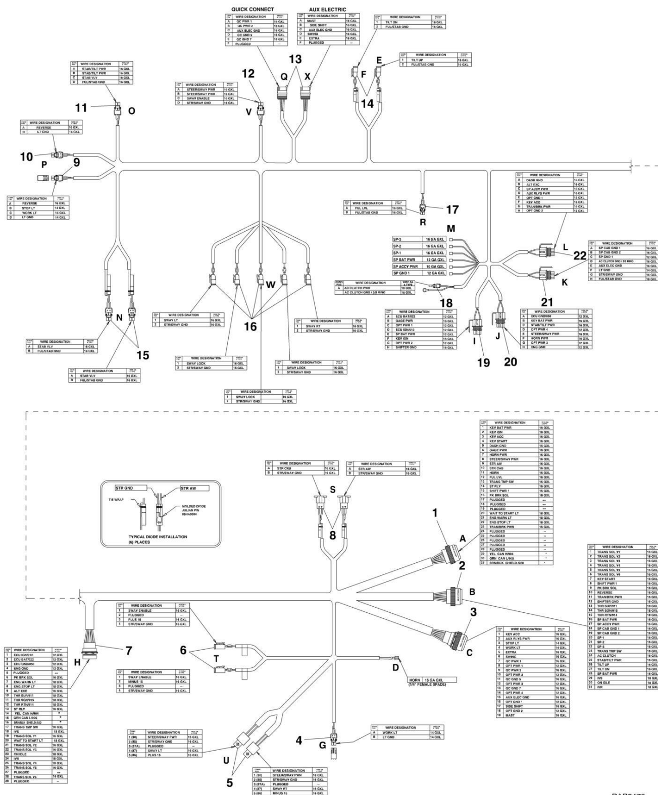
FIGURE 10-12. CHASSIS HARNESS - PERKINS AND CUMMINS ENGINE (SN 0160037795 to Present)
