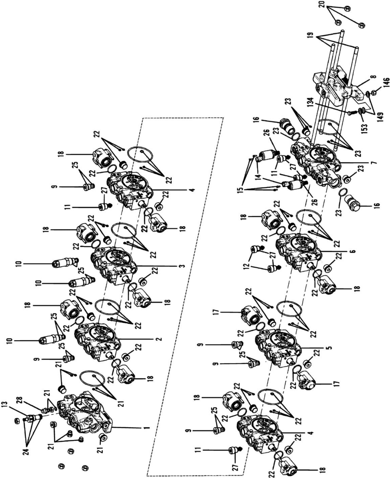
FIGURE 9-45. MAIN CONTROL VALVE (SN 0160037877 to Present)
