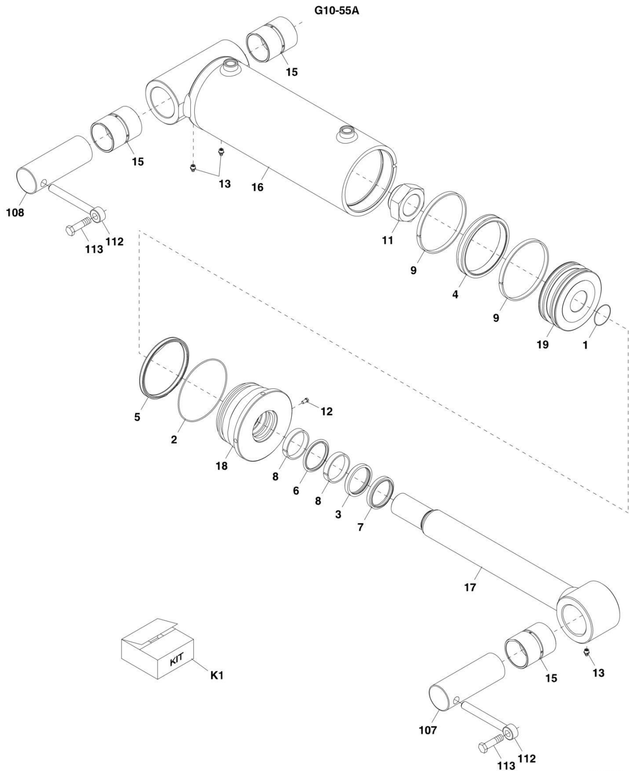
FIGURE 9-28. COMPENSATING CYLINDER (G10-55A) (G10-55A SN 0160033659 through 0160037689; Including 0160033452)
