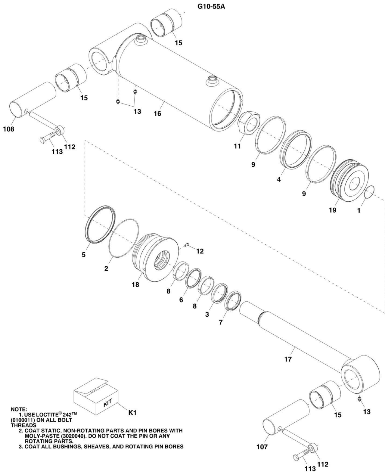
FIGURE 9-29. COMPENSATING CYLINDER (G10-55A) (G10-55A SN 0160037689 through 0160041564)
