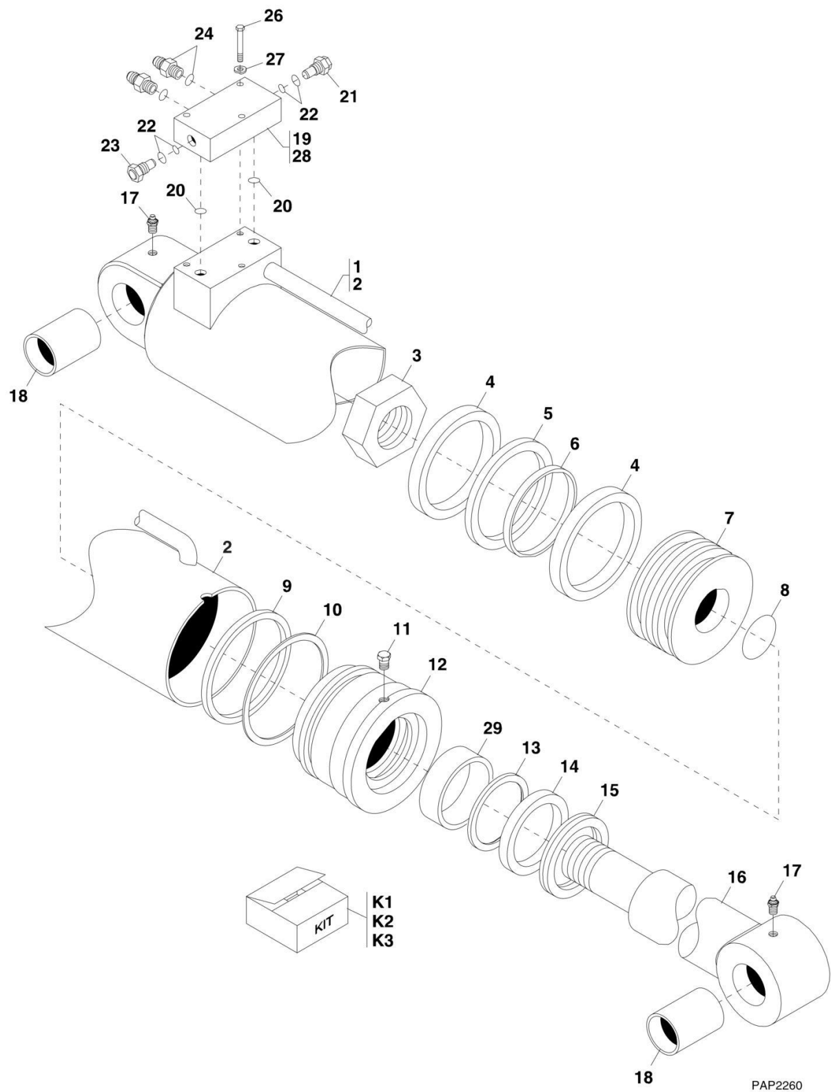
FIGURE 9-42. OUTRIGGER CYLINDER ASSEMBLY (Prior to SN 0160039838)
