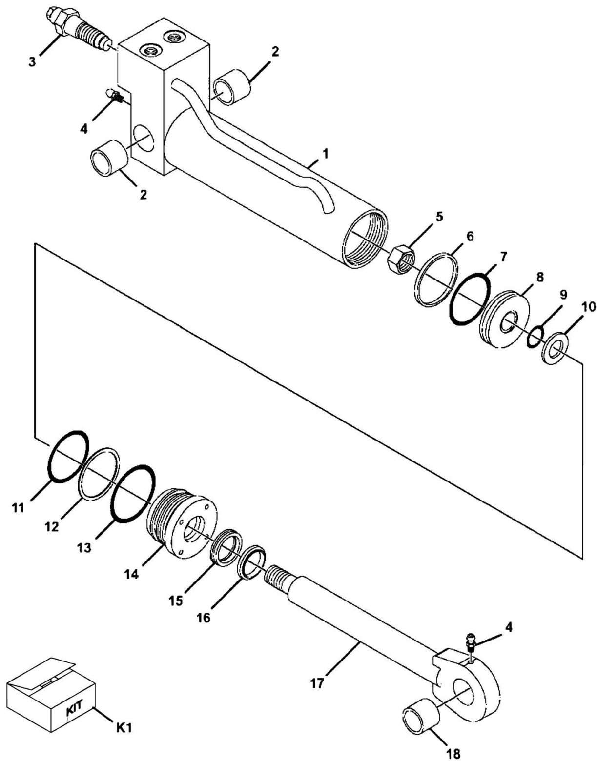
FIGURE 9-58. GRAPPLE BUCKET CYLINDER
