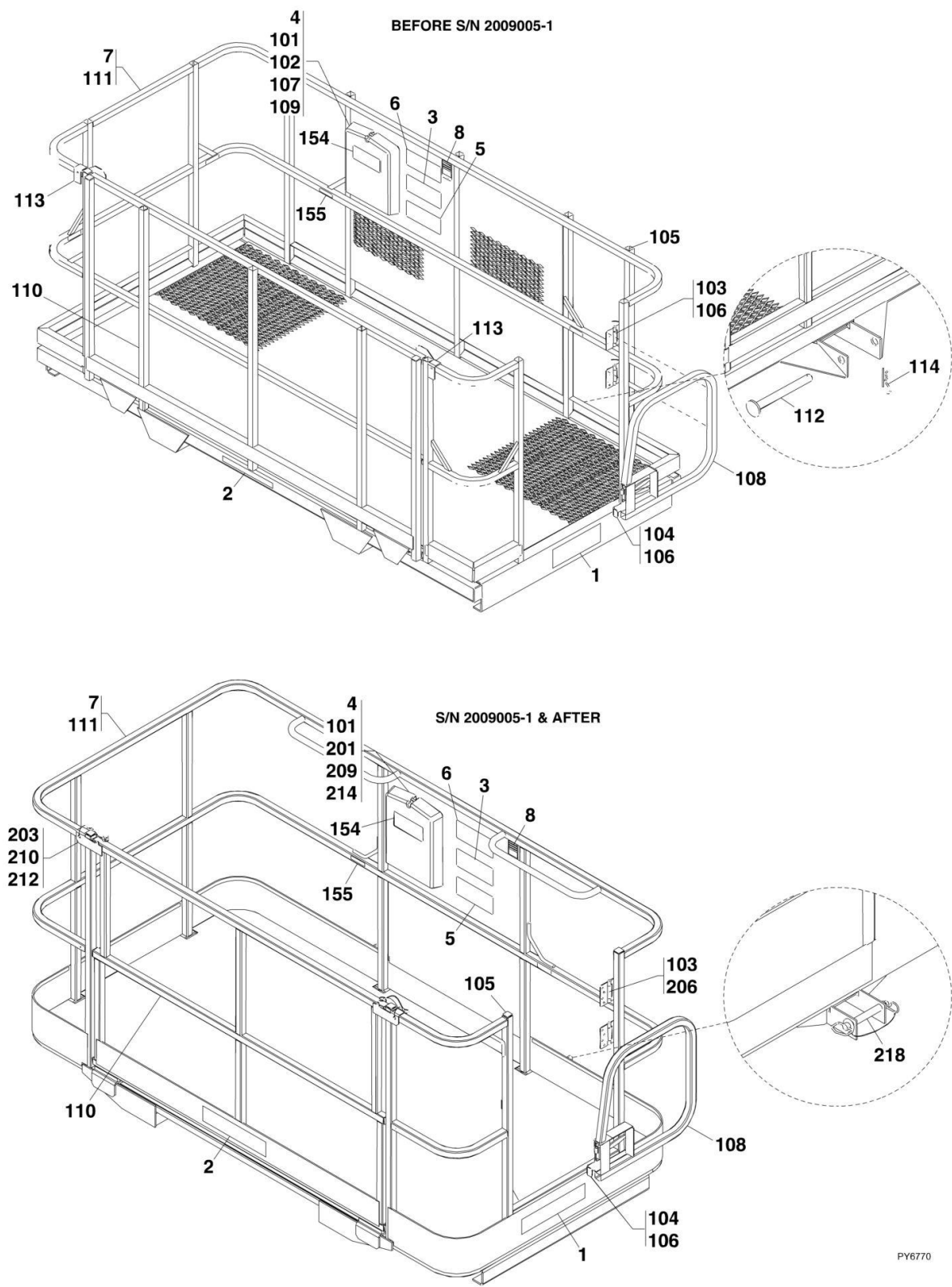
FIGURE 3-20. FORK MOUNTED PLATFORM
