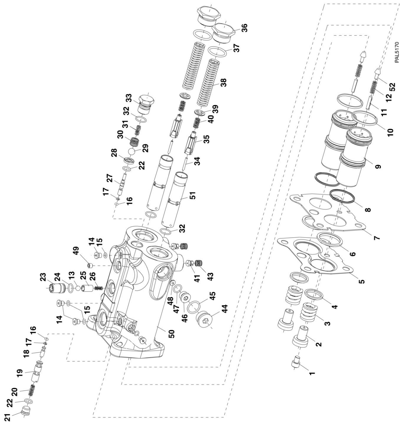
FIGURE 9-53. BRAKE VALVE (G10-55A SN 0160029245 to Present; G12-55A SN 0160029250 to Present)
