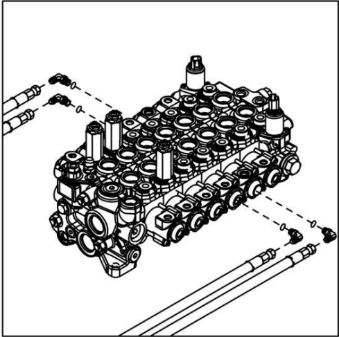
7 SECTION MAIN CONTROL VALVE
