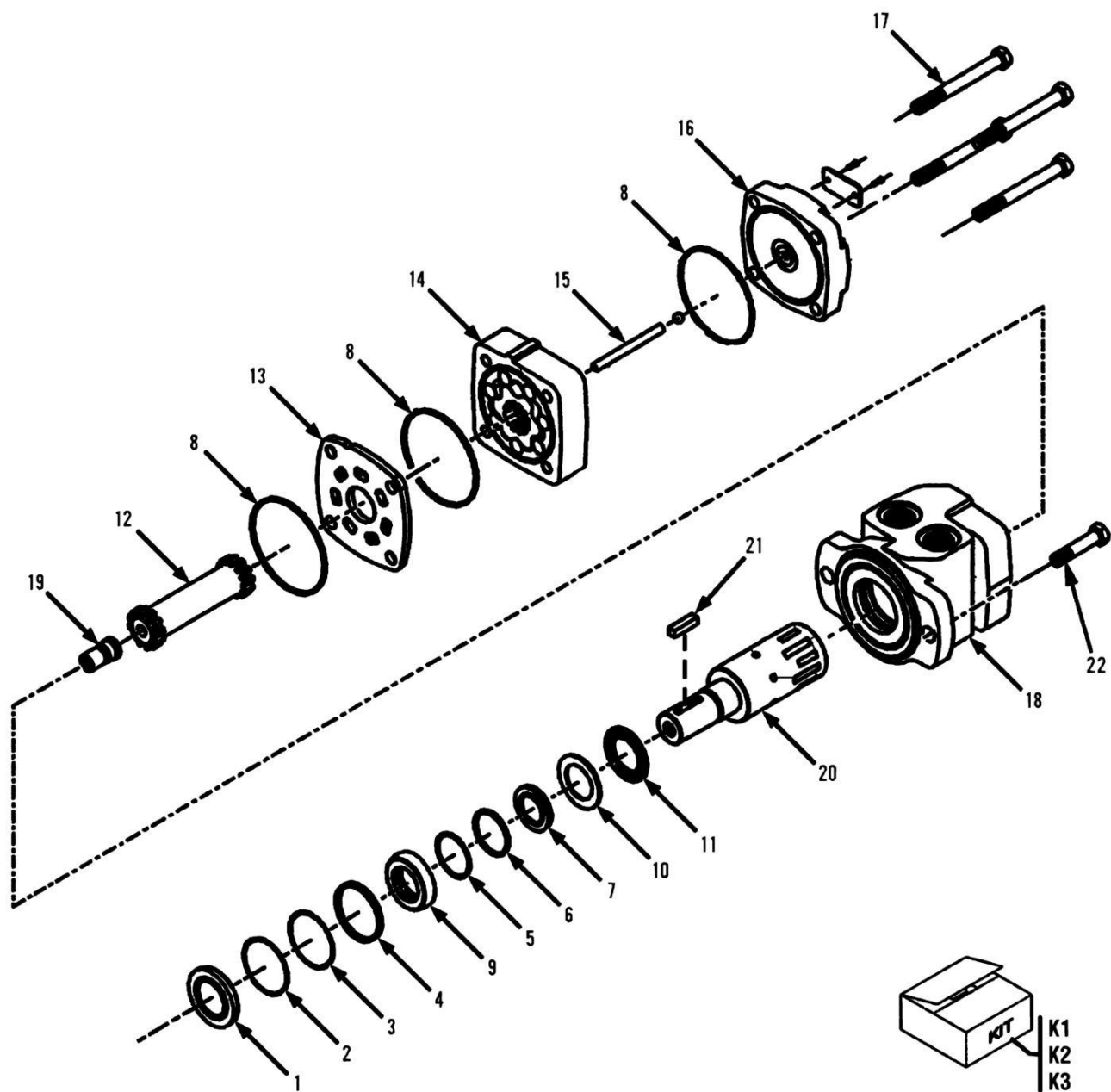
FIGURE 12-12. WINCH MOTOR
