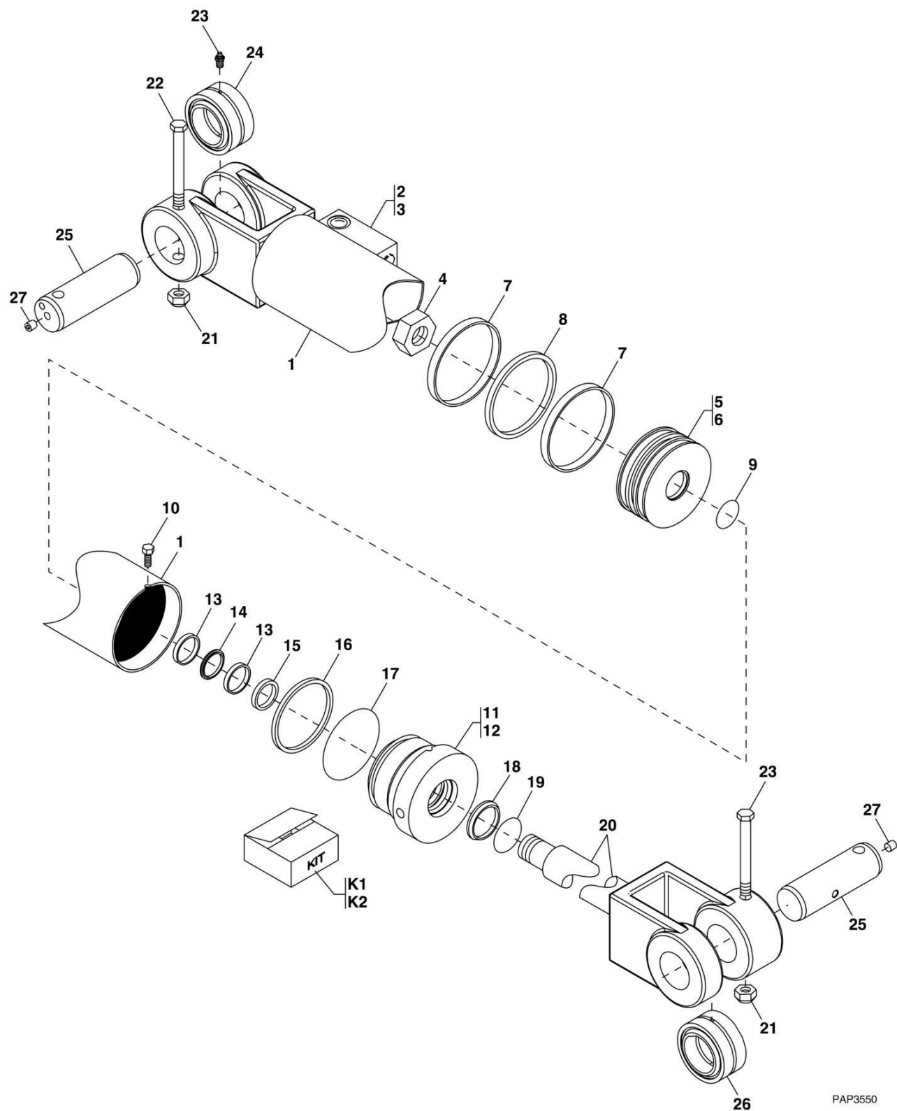
FIGURE 9-39. STABILIZER CYLINDER (G10-55A Prior to SN 0160033661; G12-55A Prior to SN 0160033659; Excluding 0160033452)
