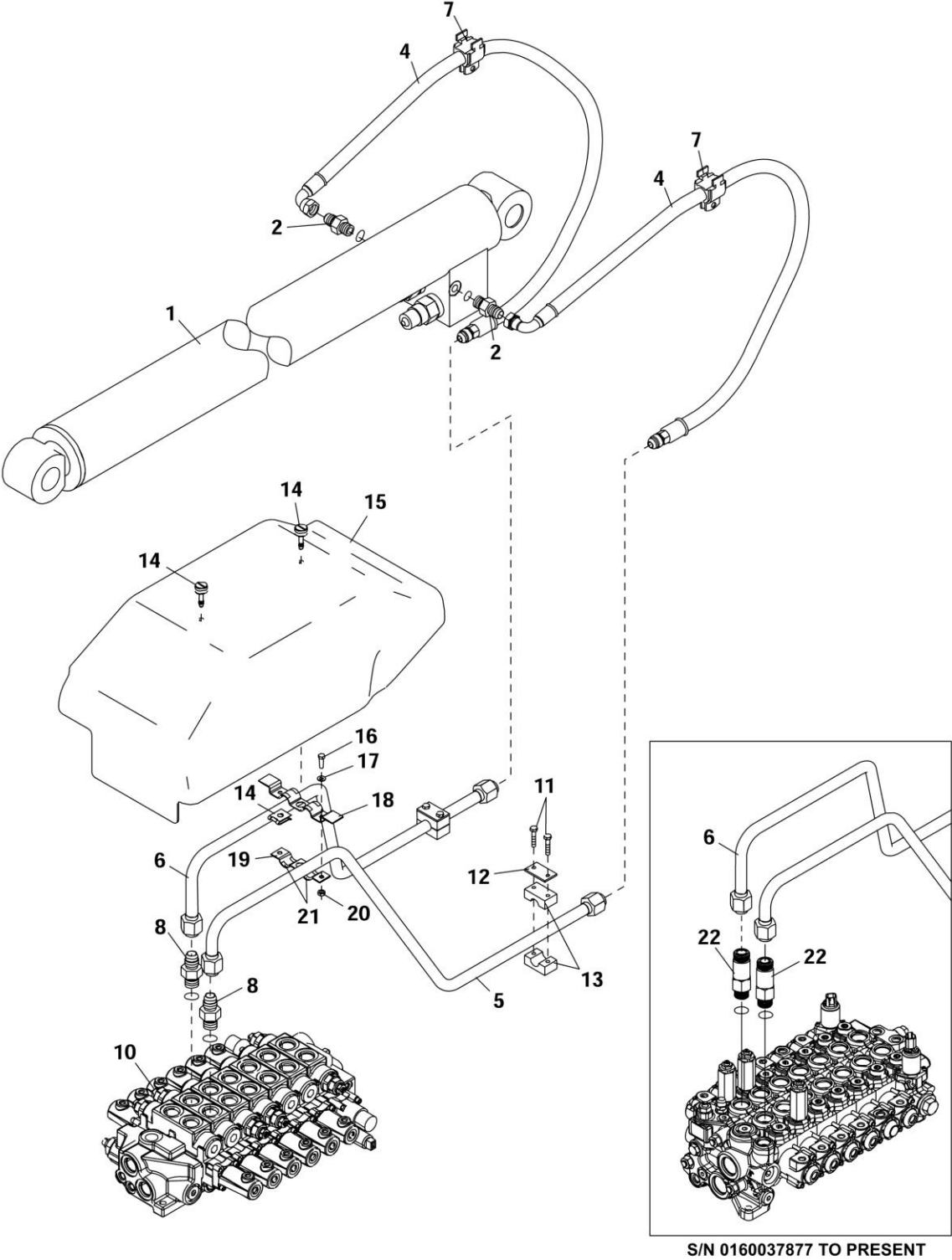
FIGURE 8-25. CROWD CYLINDER - PERKINS AND CUMMINS ENGINE
