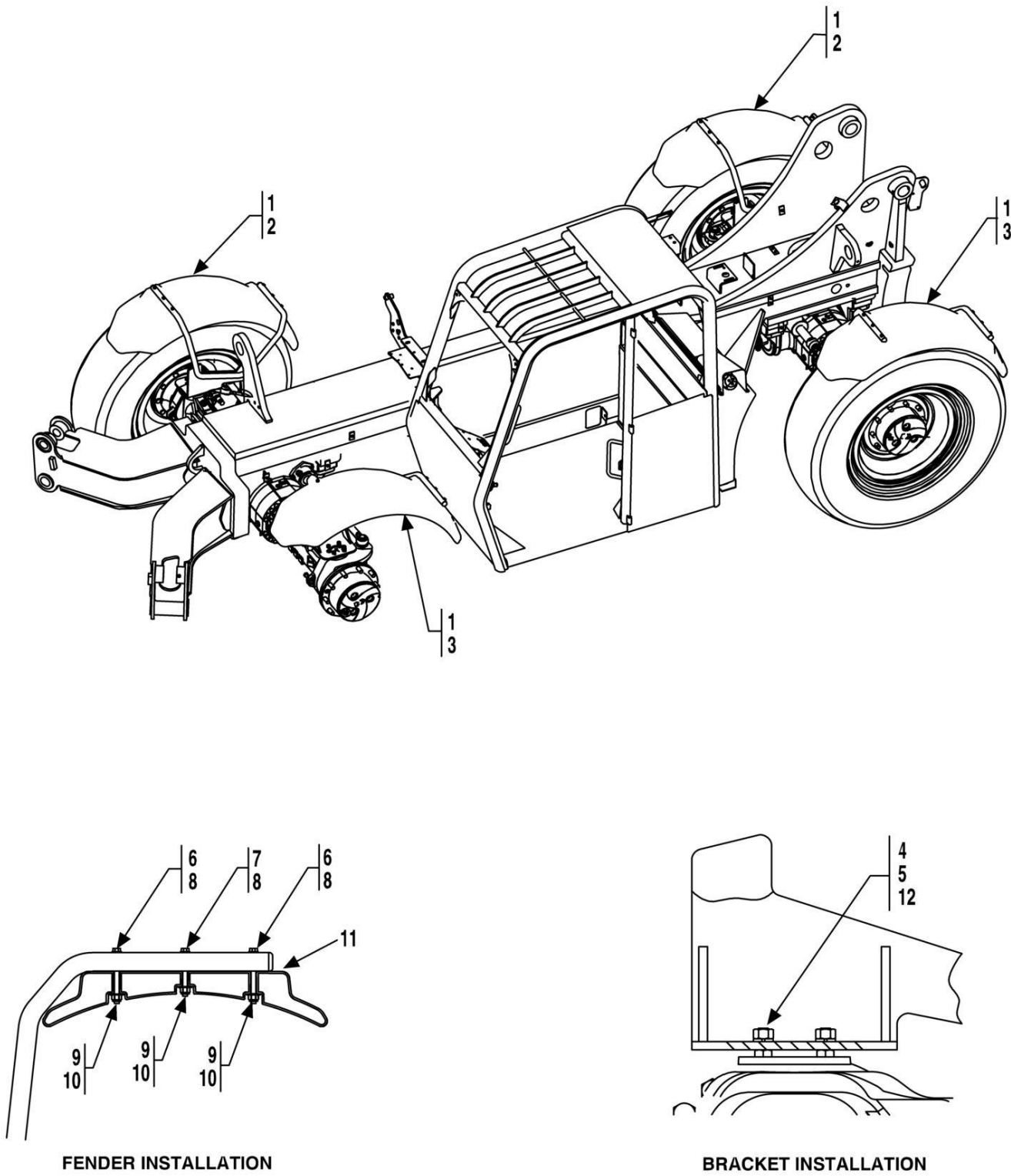
FIGURE 12-7. FENDER INSTALLATION
