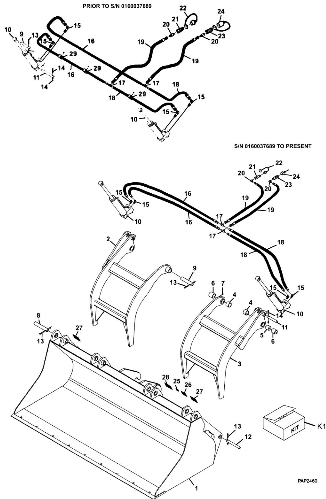
FIGURE 3-24. GRAPPLE BUCKET
