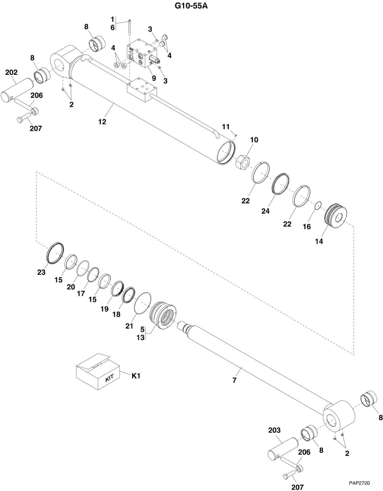
FIGURE 9-5. LIFT CYLINDER (G10-55A) (G10-55A SN 0160041374 to Present)
