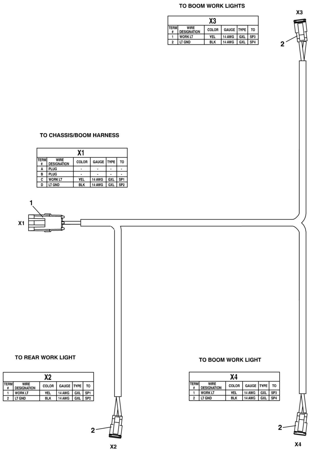
FIGURE 12-20. BOOM WORK LIGHT HARNESS
