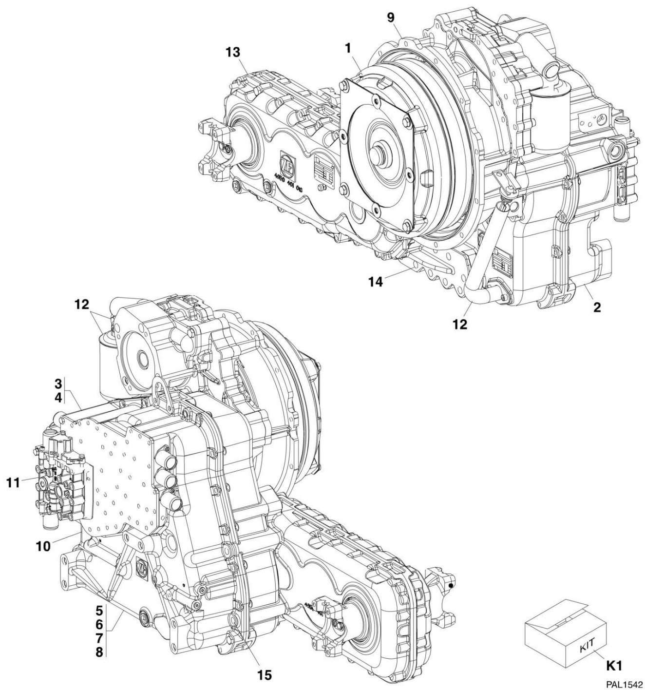
FIGURE 4-20. ZF TRANSMISSION
