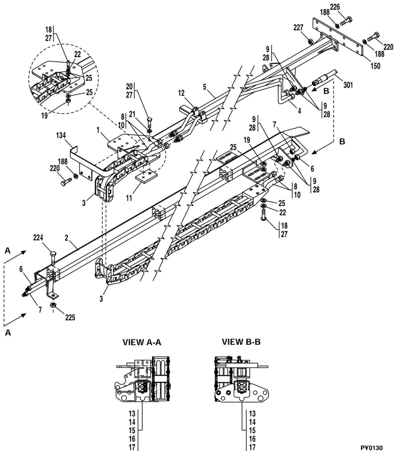
FIGURE 8-30. BOOM HYDRAULICS ASSEMBLY (Prior to SN 0160025075, Excluding 0160022656 and 0160025022)
