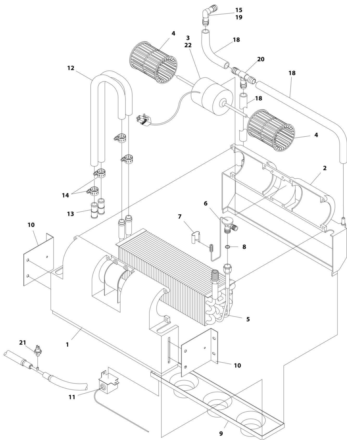
FIGURE 6-16. AIR CONDITIONING COMPONENTS (SN 0160045292 to Present)
