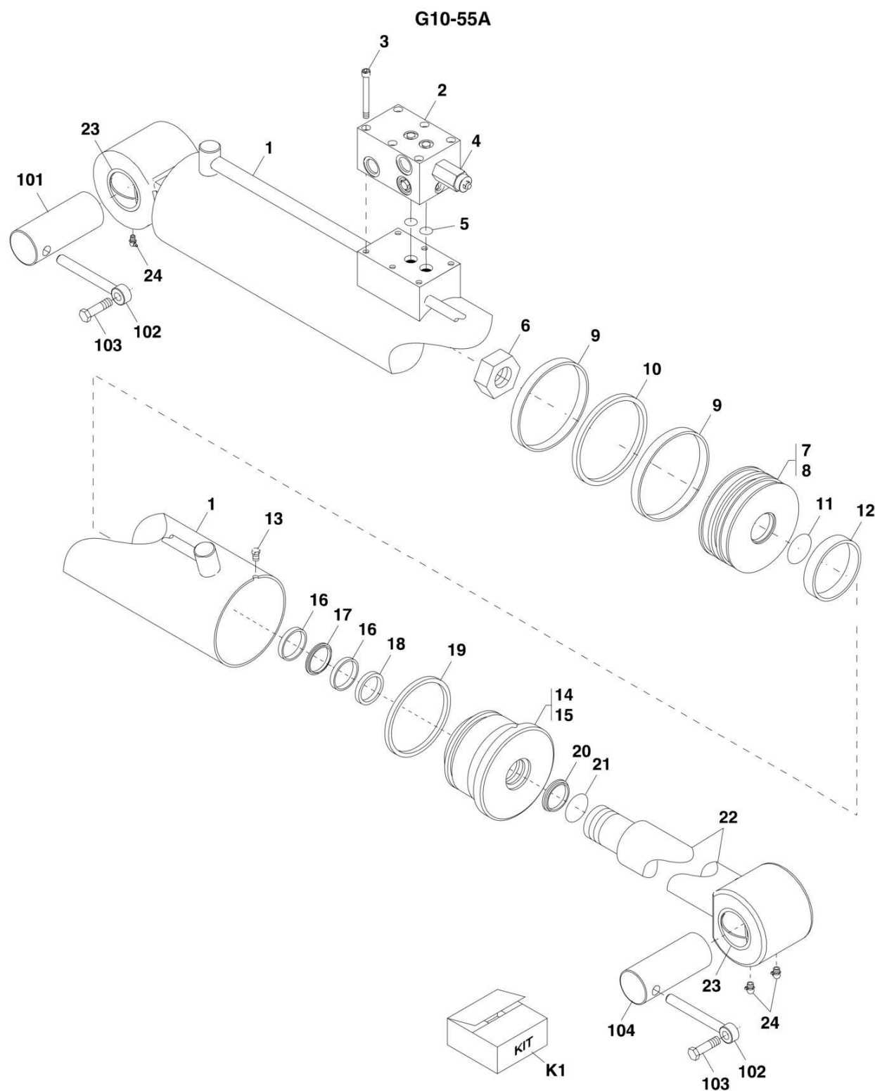
FIGURE 9-1. LIFT CYLINDER (G10-55A) (G10-55A Prior to SN 0160033659; Excluding 0160033452)
