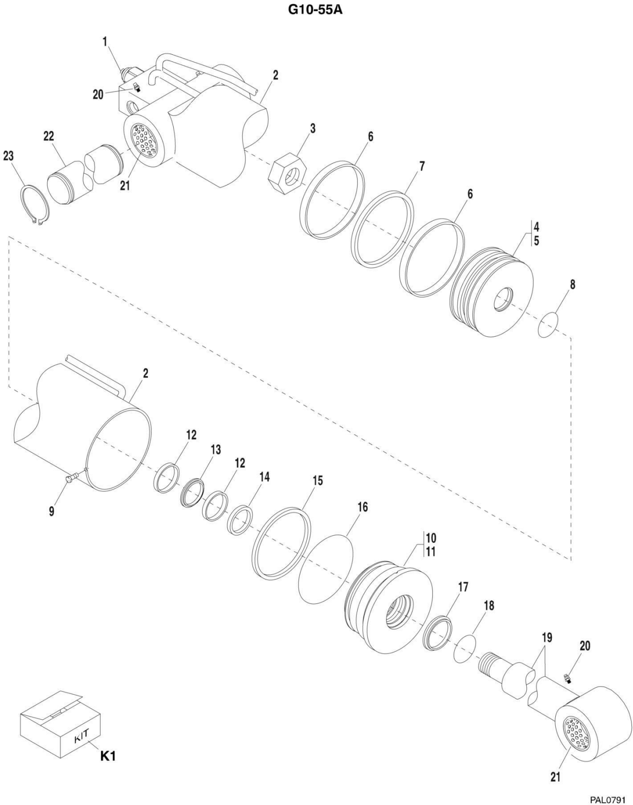
FIGURE 9-19. TILT CYLINDER (G10-55A) (G10-55A Prior to SN 0160033661)
