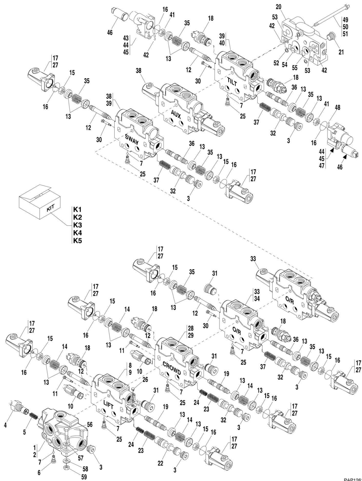
FIGURE 9-44. MAIN CONTROL VALVE (Prior to SN 0160037877)
