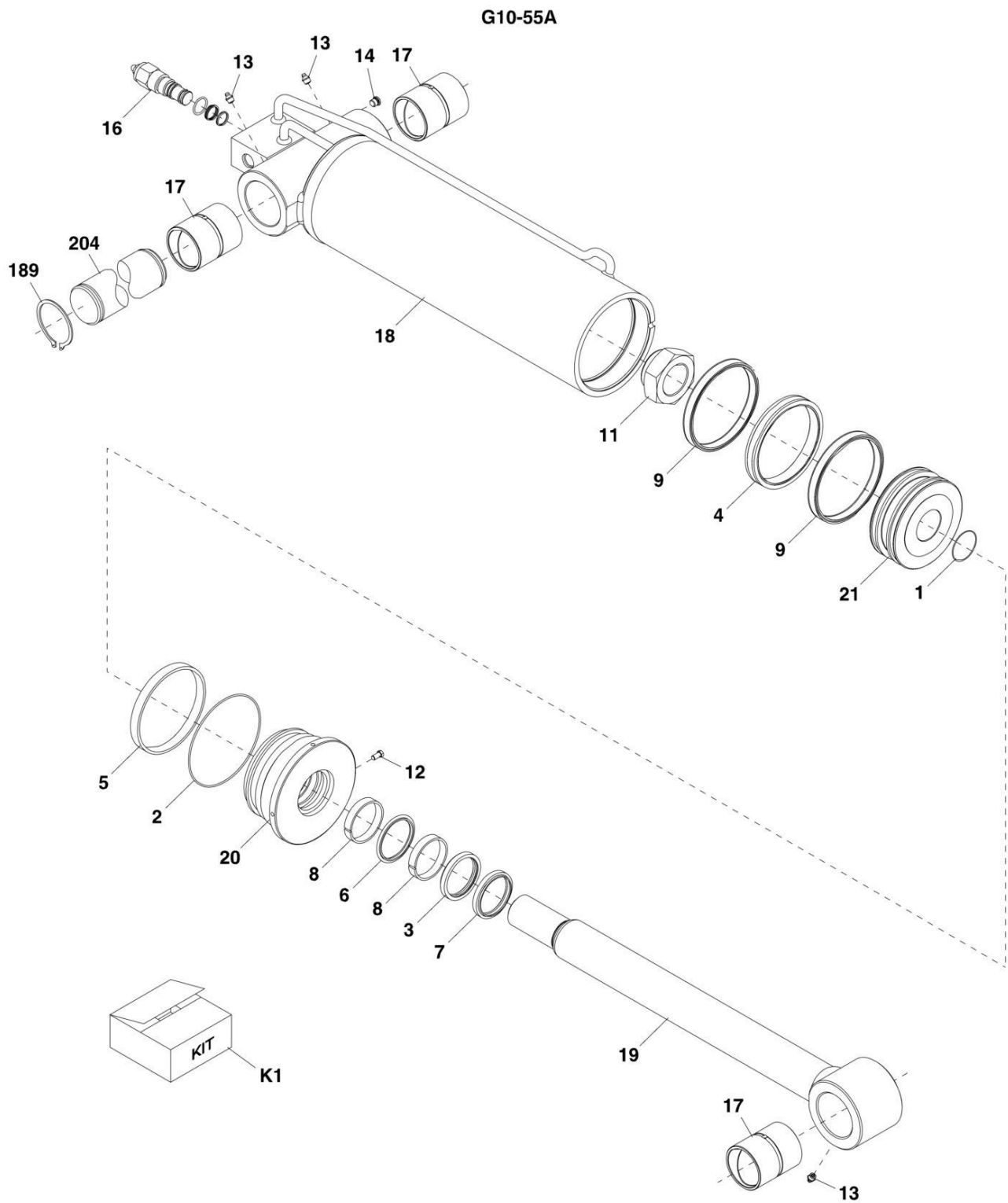
FIGURE 9-20. TILT CYLINDER (G10-55A) (G10-55A SN 0160033661 through 0160035822)
