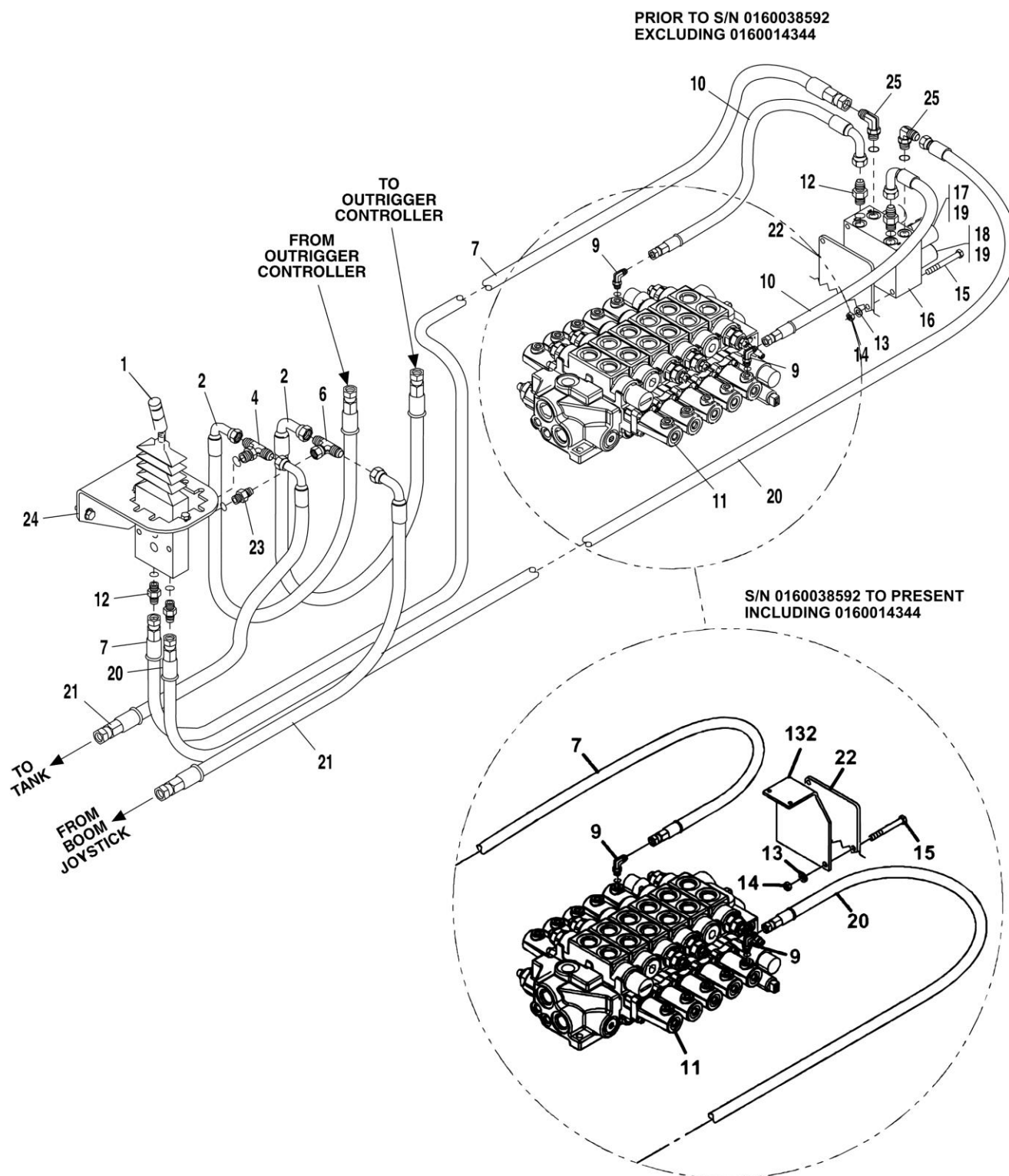
FIGURE 8-16. SWAY CONTROLLER - PERKINS ENGINE
