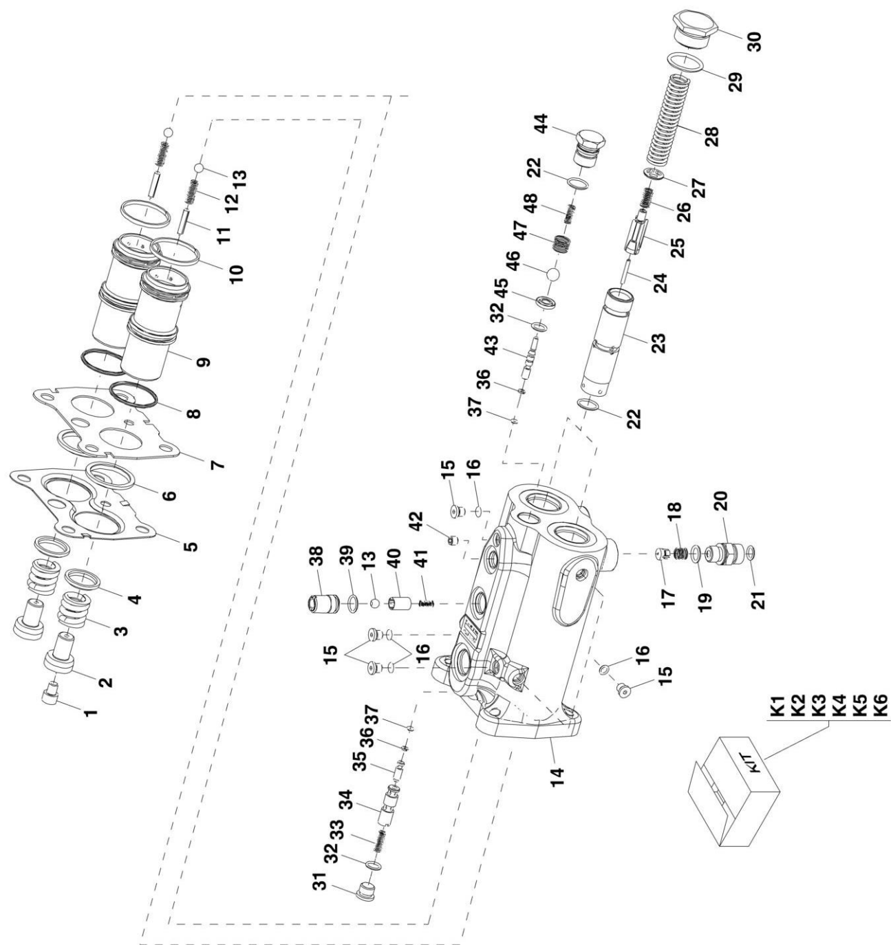
FIGURE 9-52. BRAKE VALVE (G10-55A Prior to SN 0160029245; G12-55A Prior to SN 0160029250)
