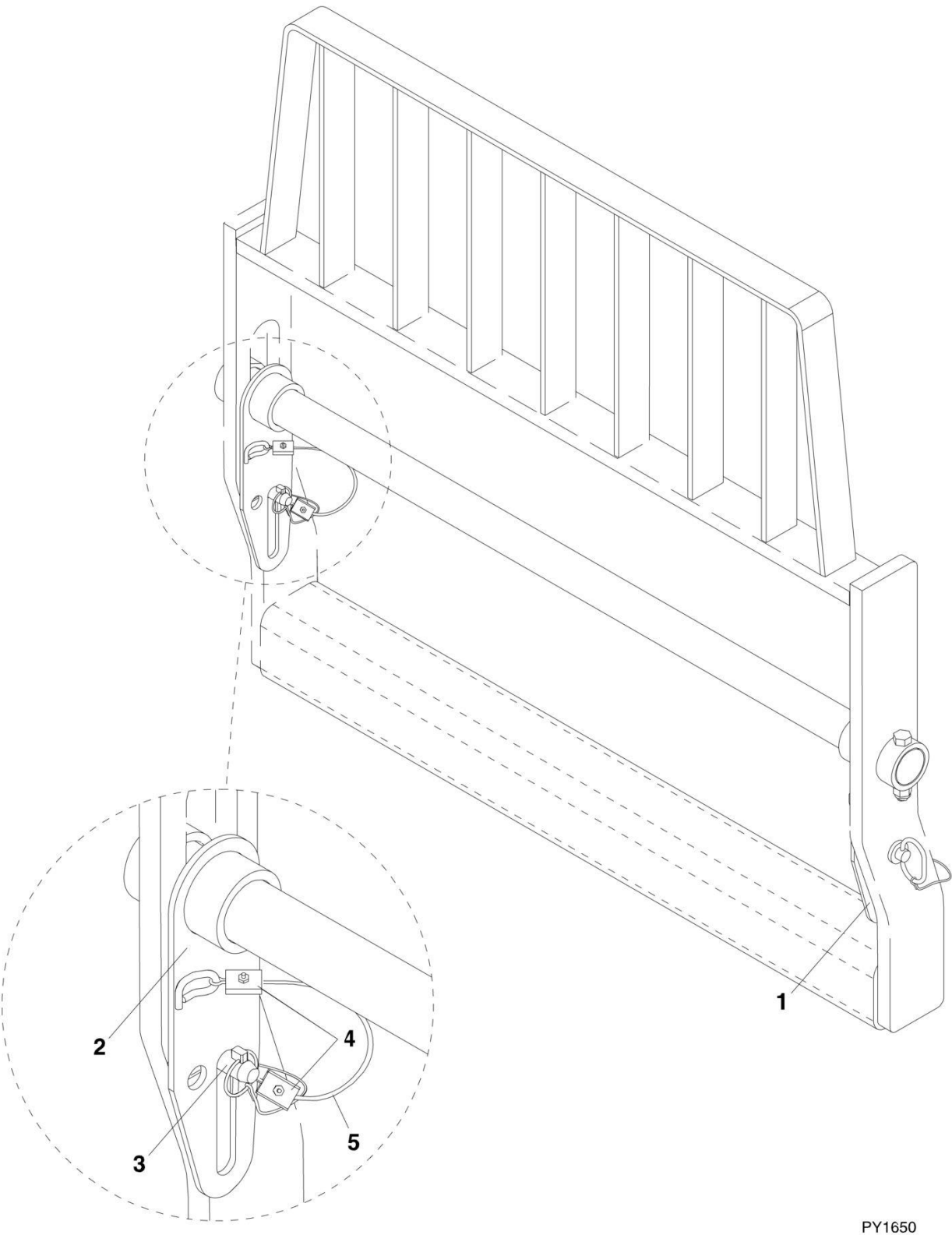
FIGURE 3-25. FORK PIN LOCK INSTALLATION (SN 0160037689 to Present)
