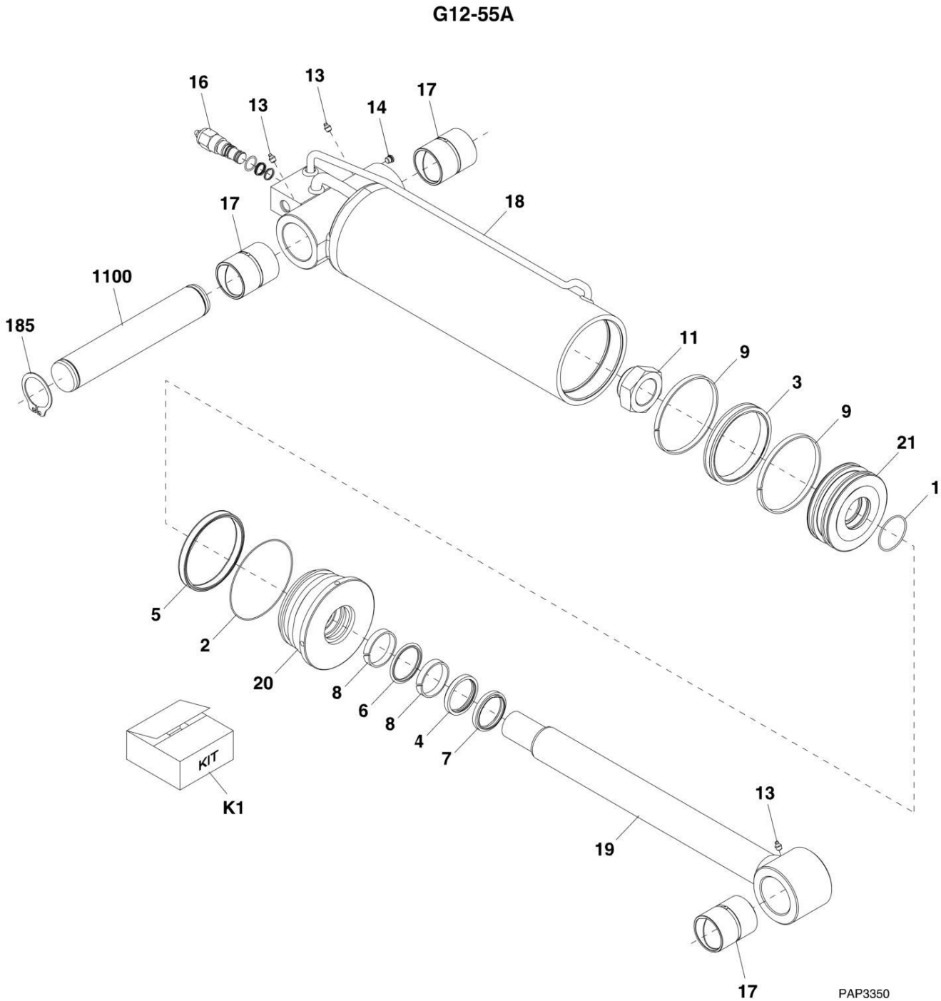
FIGURE 9-24. TILT CYLINDER (G12-55A) (G12-55A SN 0160033659 through 0160035879; Including 0160033452)
