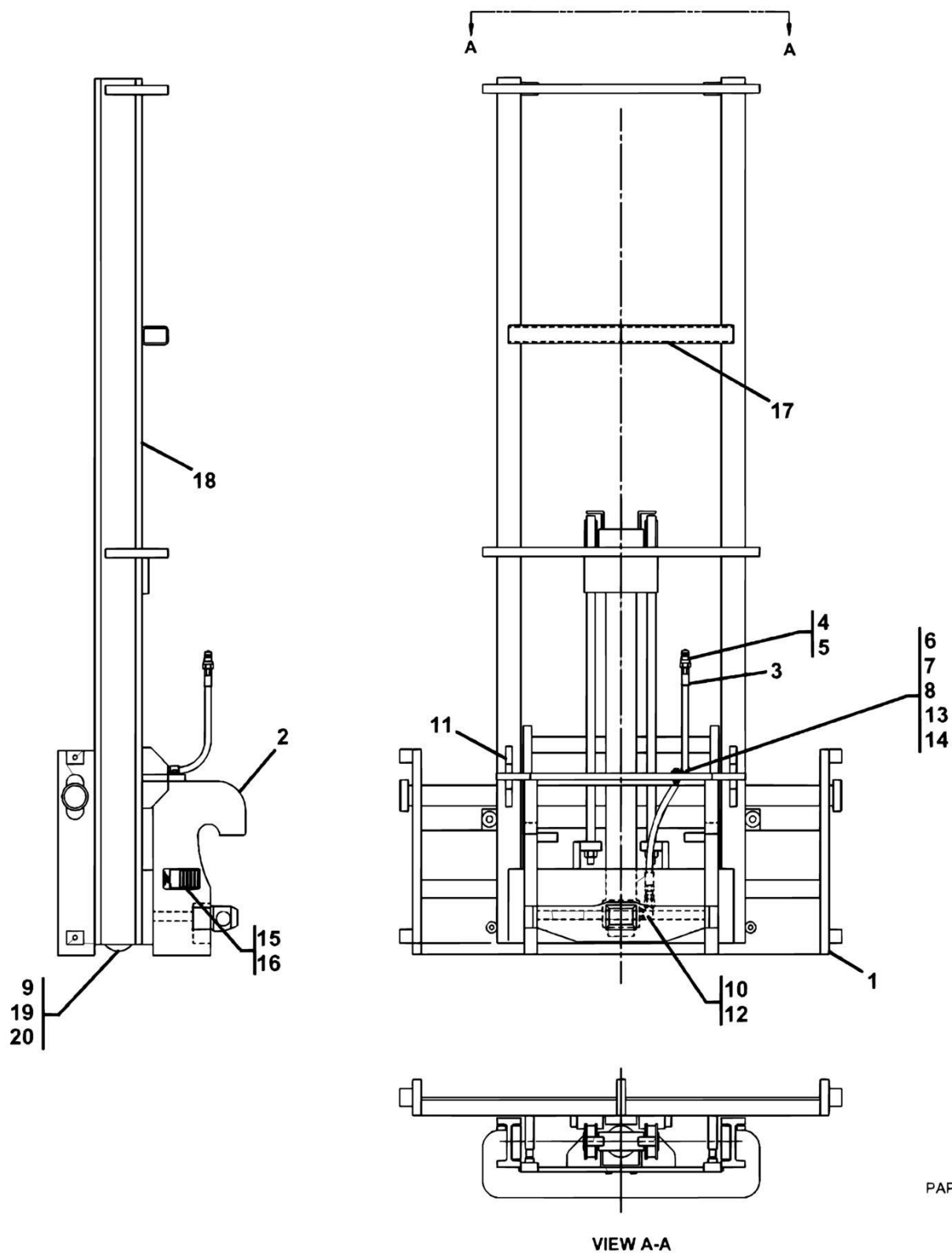
FIGURE 3-27. 6 FT MAST WITH 72 IN CARRIAGE (Prior to SN 0160037938)
