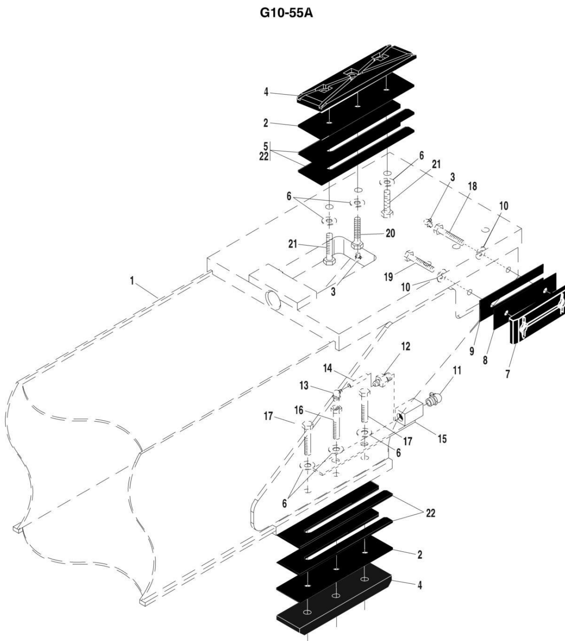
FIGURE 2-15. BEARINGS, PADS, SPACERS AND SHIMS, (FOURTH BOOM SECTION) (G10-55A)
