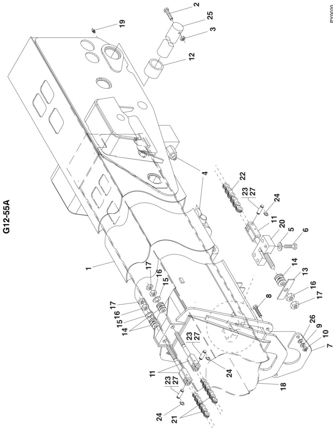
FIGURE 2-2. FIRST BOOM SECTION (G12-55A)
