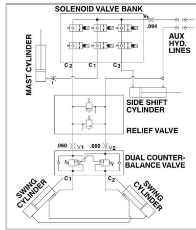
HYDRAULIC SCHEMATIC
