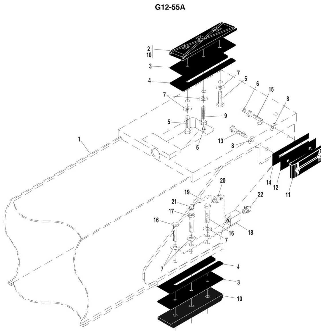
FIGURE 2-16. BEARINGS, PADS, SPACERS AND SHIMS, (FOURTH BOOM SECTION) (G12-55A)
