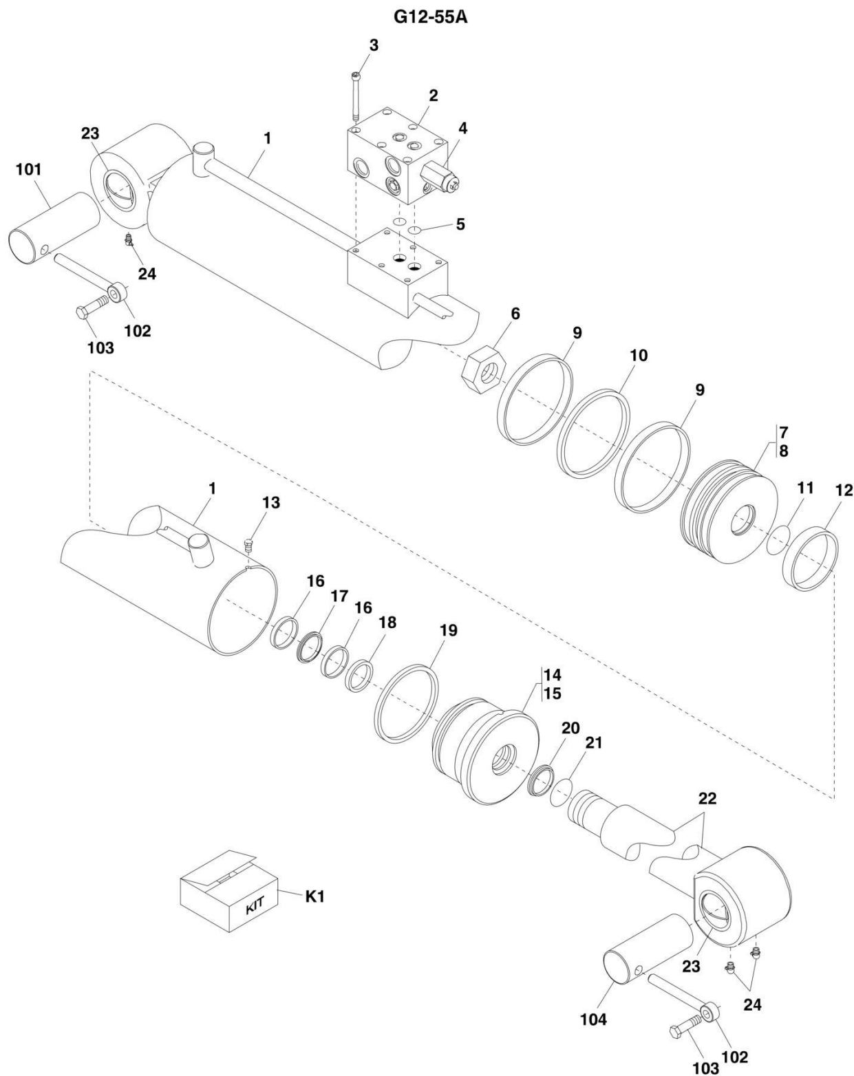
FIGURE 9-7. LIFT CYLINDER (G12-55A) (G12-55A Prior to SN 0160033659; Excluding 0160033452)
