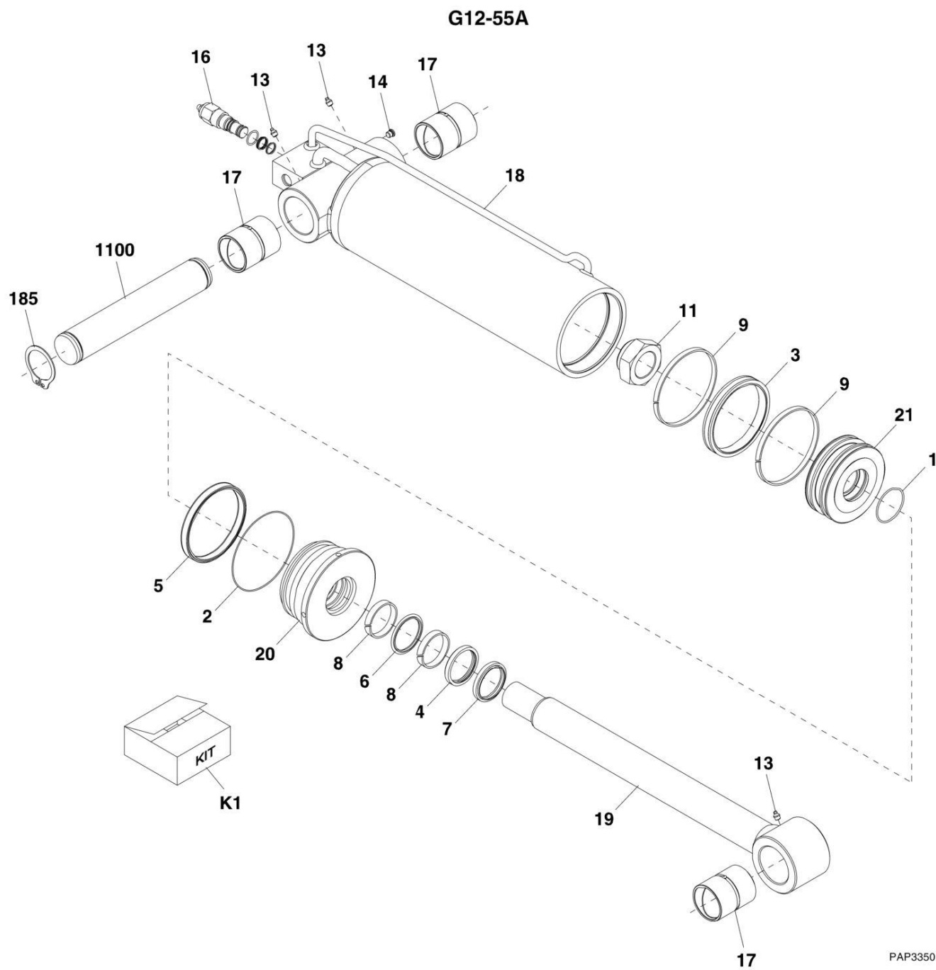
FIGURE 9-25. TILT CYLINDER (G12-55A) (G12-55A SN 0160035879 through 0160037689)
