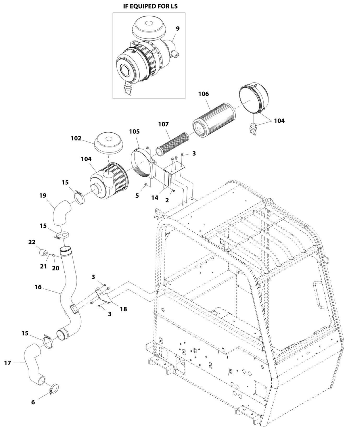
FIGURE 4-13. AIR CLEANER INSTALLATION IF EQUIPPED FOR LS (SN 0160071240 to Present, Including 0160018840, 0160019245 and 0160019746)
