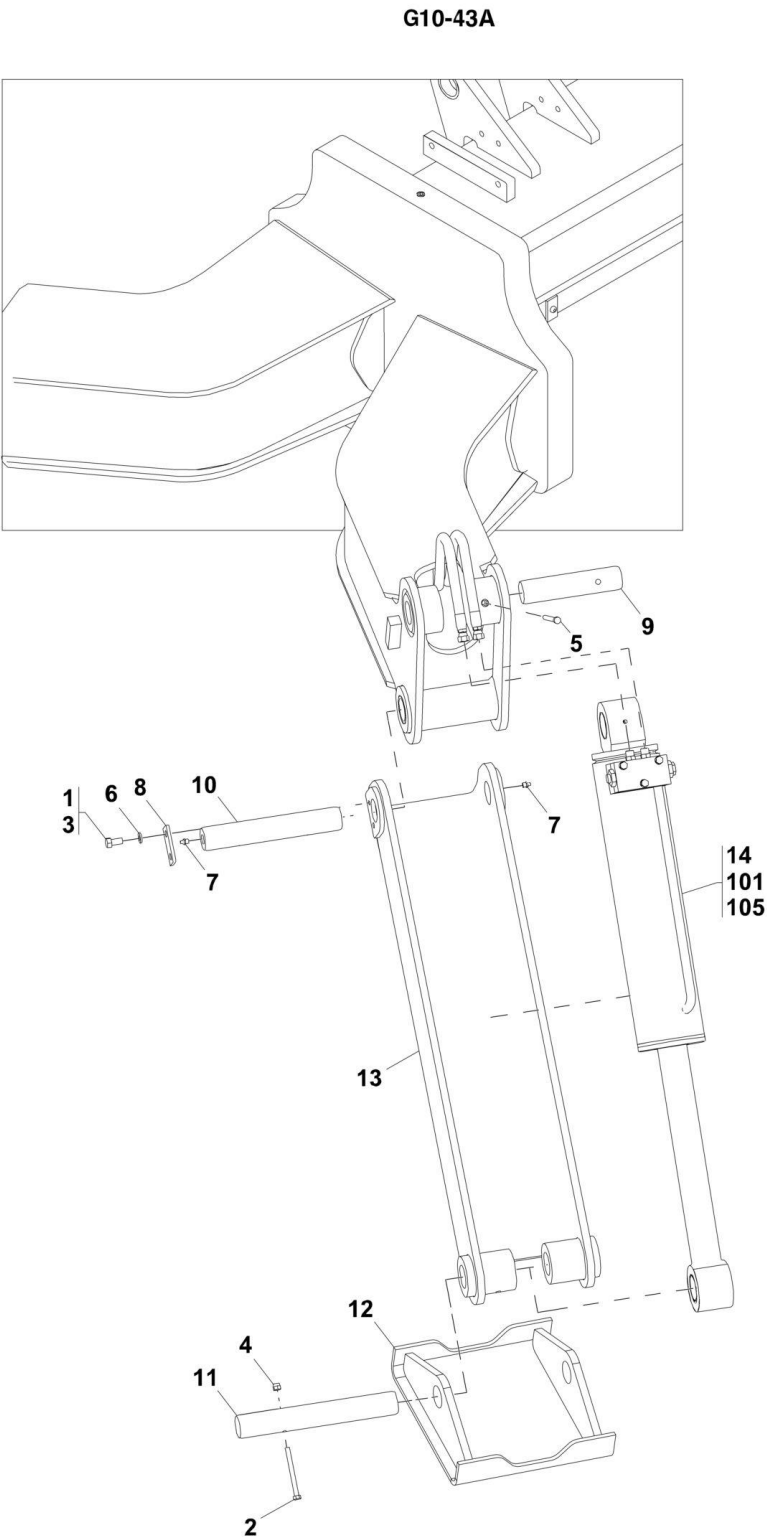
FIGURE 1-4. OUTRIGGER INSTALLATION (G10-43A)
