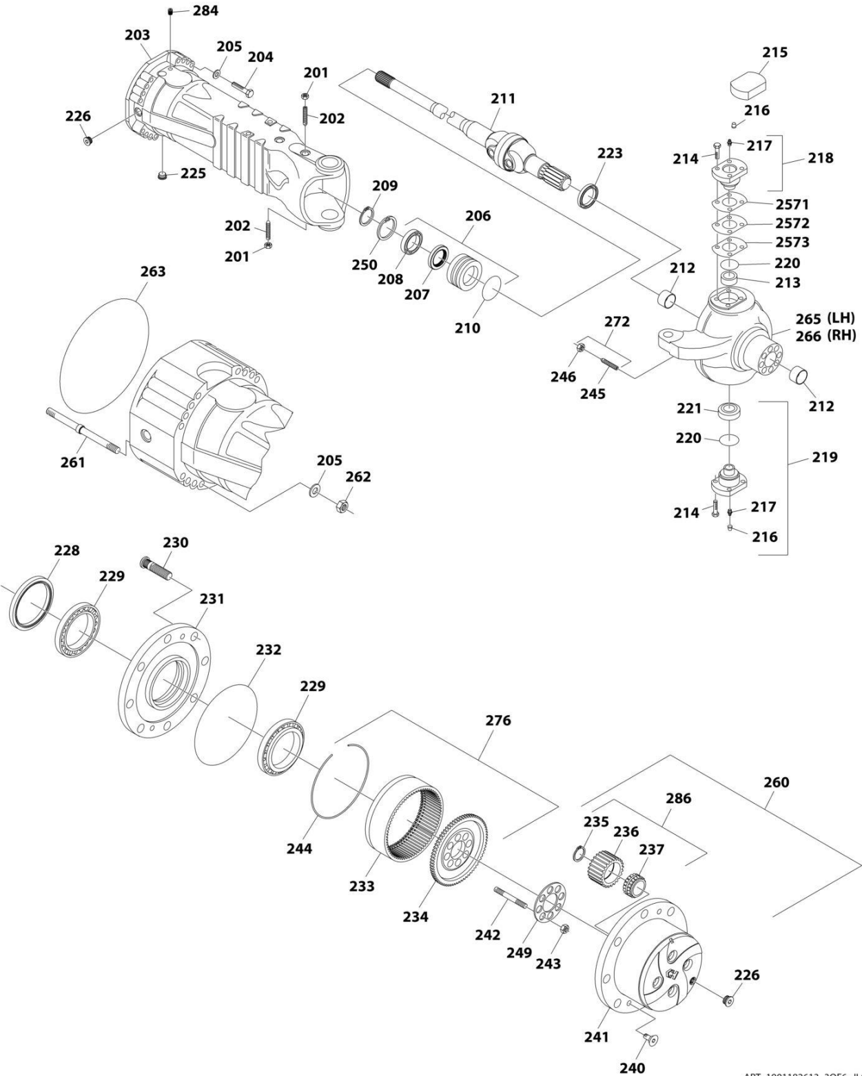
FIGURE 5-12. HUB REDUCTION (G6-42A) (SN 0160065511 to Present)
