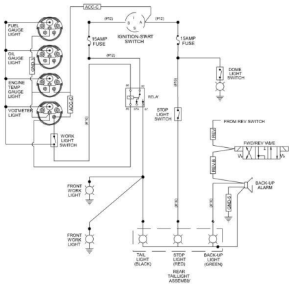
ELECTRICAL SCHEMATIC
