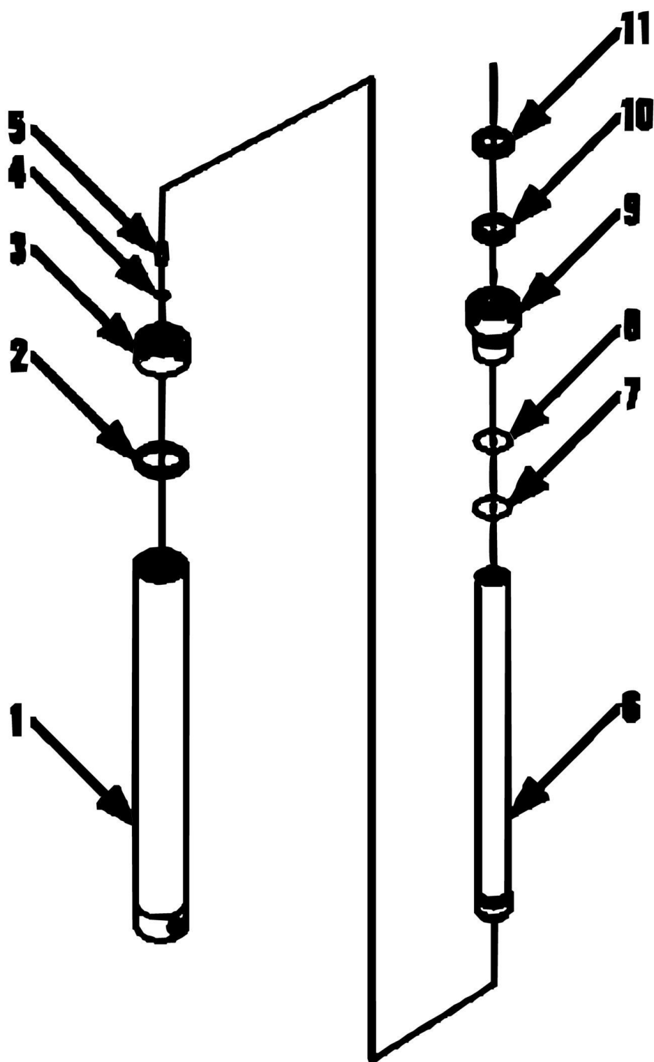
FIGURE 12-56. (91034404) RAIL CYLINDER ASSEMBLY (SN 0355001 to Present)
