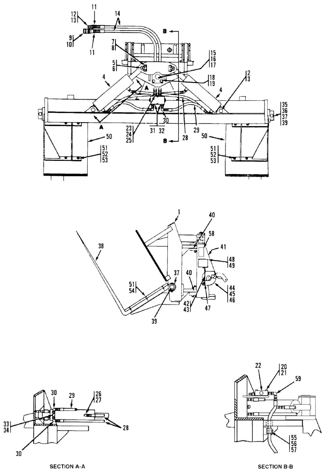
FIGURE 12-26. (90555013) 100 DRYWALL SWING FORK ASSEMBLY
