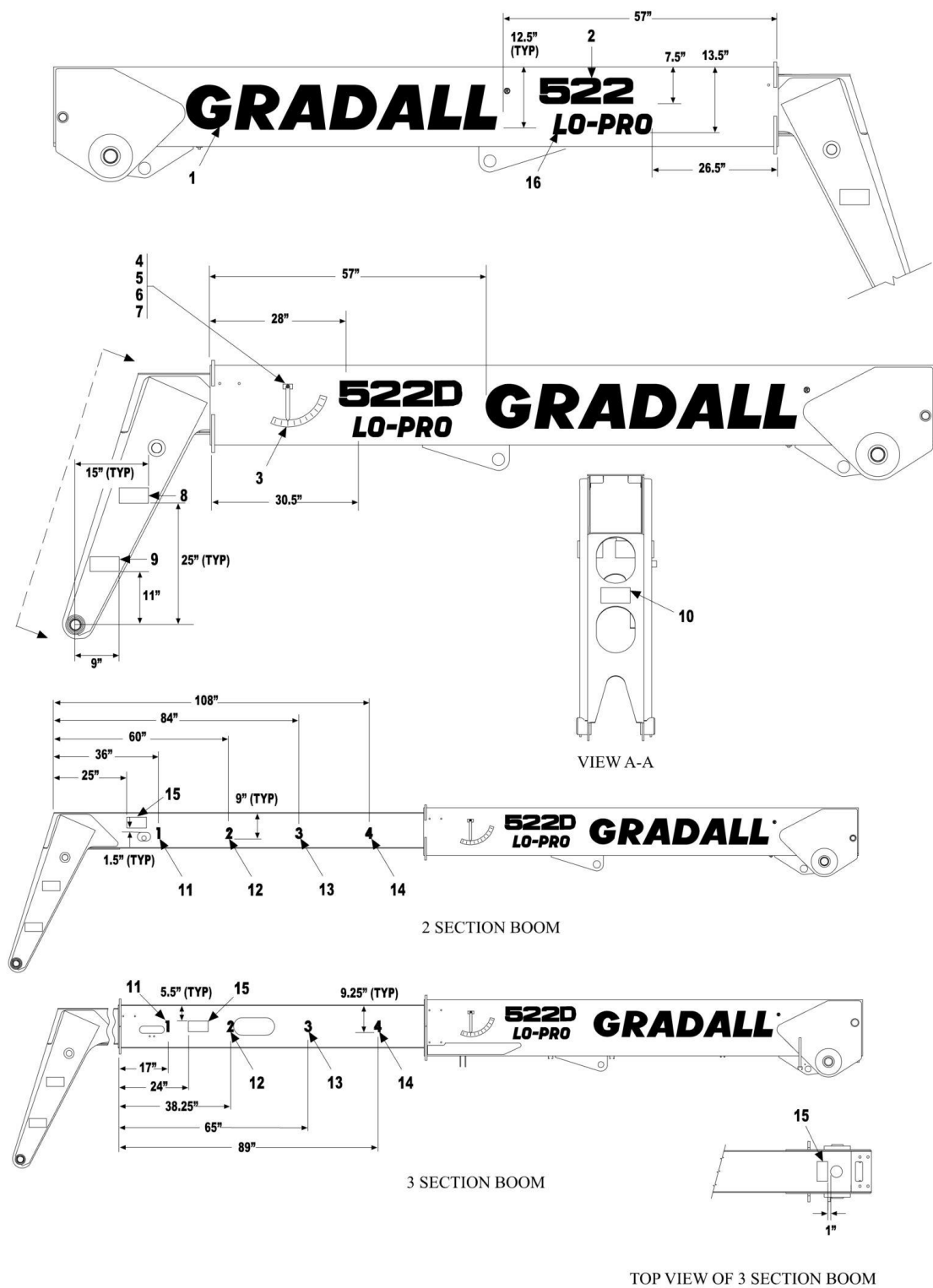
FIGURE 11-3. BOOM DECALS
