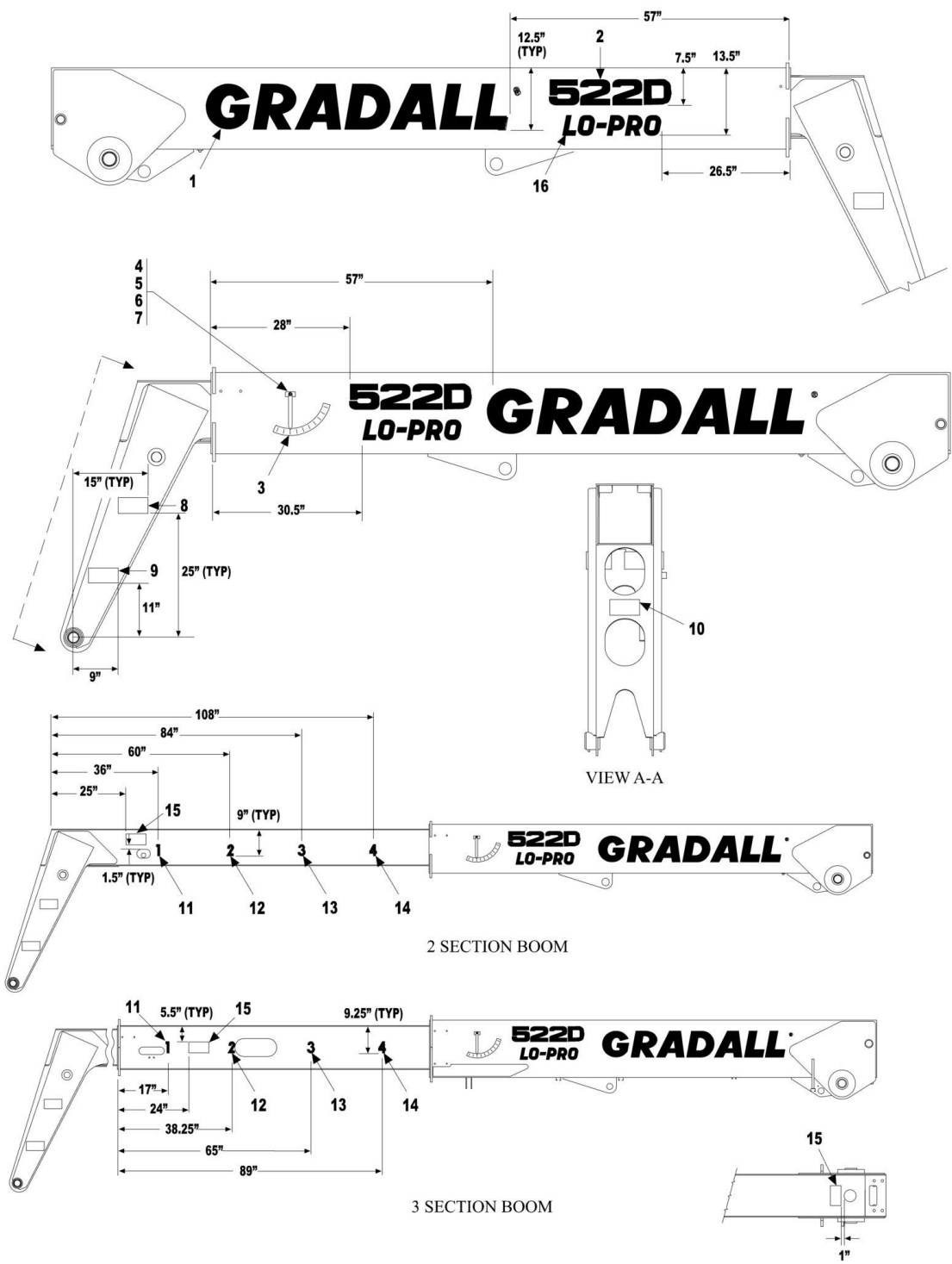
FIGURE 11-4. BOOM DECALS
