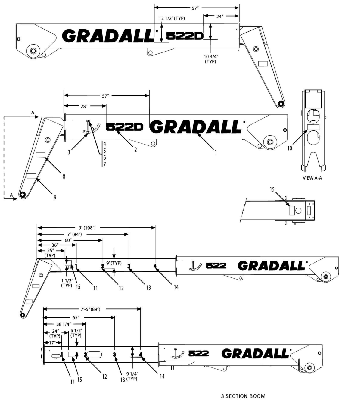
3 SECTION BOOM
