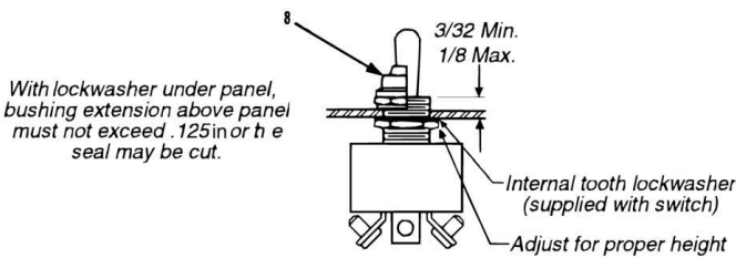
TYPICAL SWITCH AND BOOT INSTALLATION
