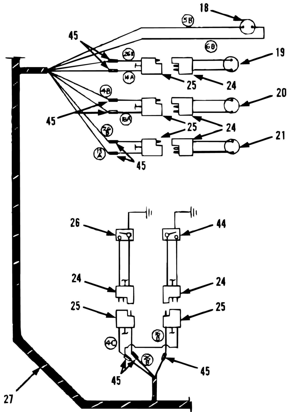
VIEW A
